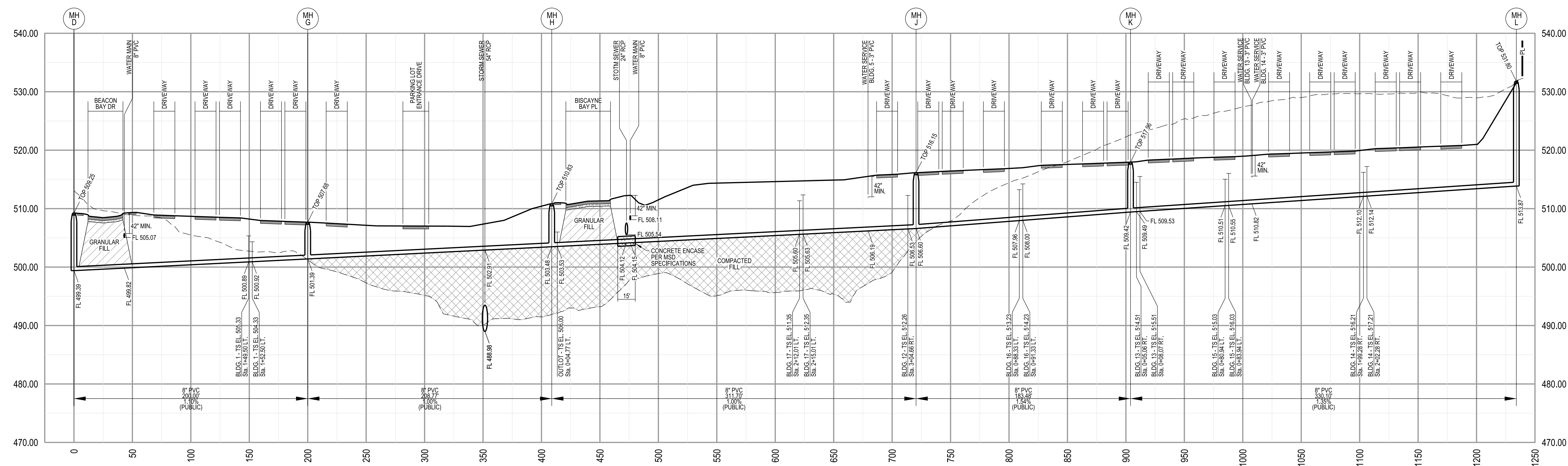
SANITARY PROFILE: MH D - MH L
