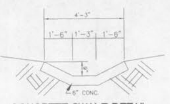
CONCRETE SWALE DETAIL BUILD SWALE WITH CONSTRUCTION JOINTS @ 5' CTRS. SEALED THE SAME AS PAVEMENT JOINTS.
