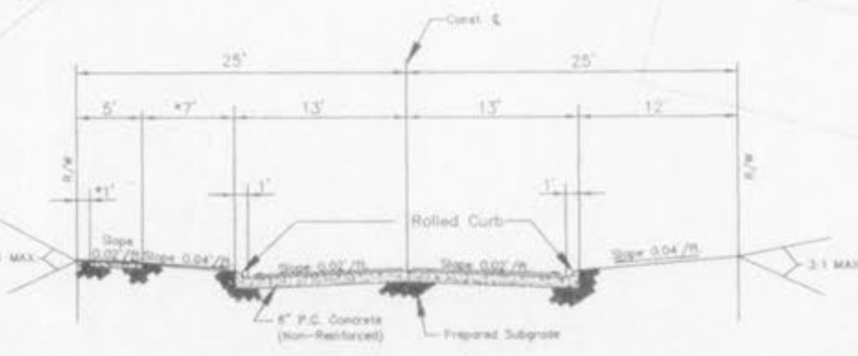
TYPICAL SECTION FALLON VILLAS CT.
