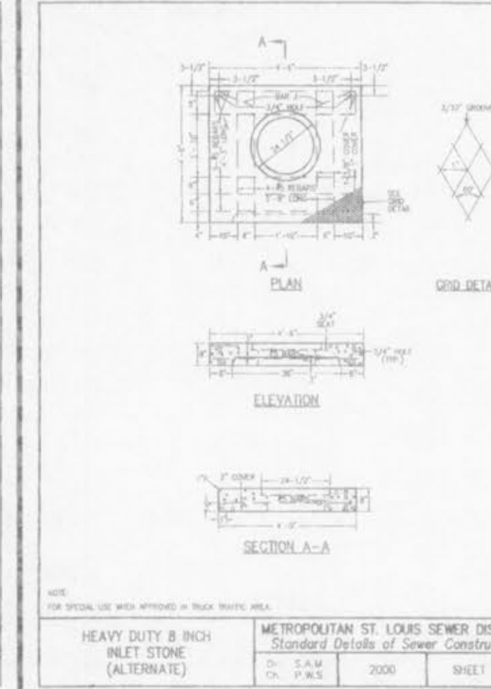
HEAVY DUTY 8 INCH INLET STONE (ALTERNATE) METROPOLITAN ST. LOUIS SEWER DISTRICT Standard Details of Sewer Construction
