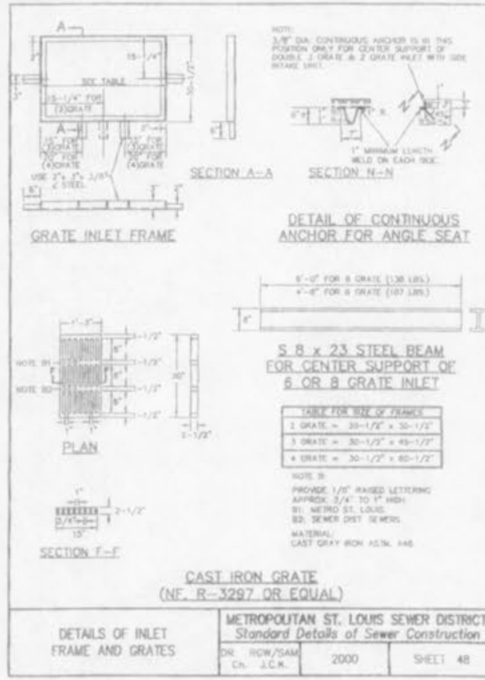
DETAILS OF INLET FRAME AND GRATES METROPOLITAN ST. LOUIS SEWER DISTRICT Standard Details of Sewer Construction
