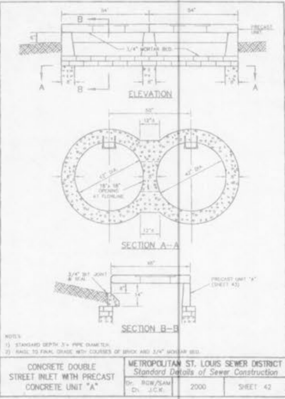
CONCRETE DOUBLE STREET INLET WITH PRECAST CONCRETE UNIT "A" METROPOLITAN ST. LOUIS SEWER DISTRICT Standard Details of Sewer Construction
