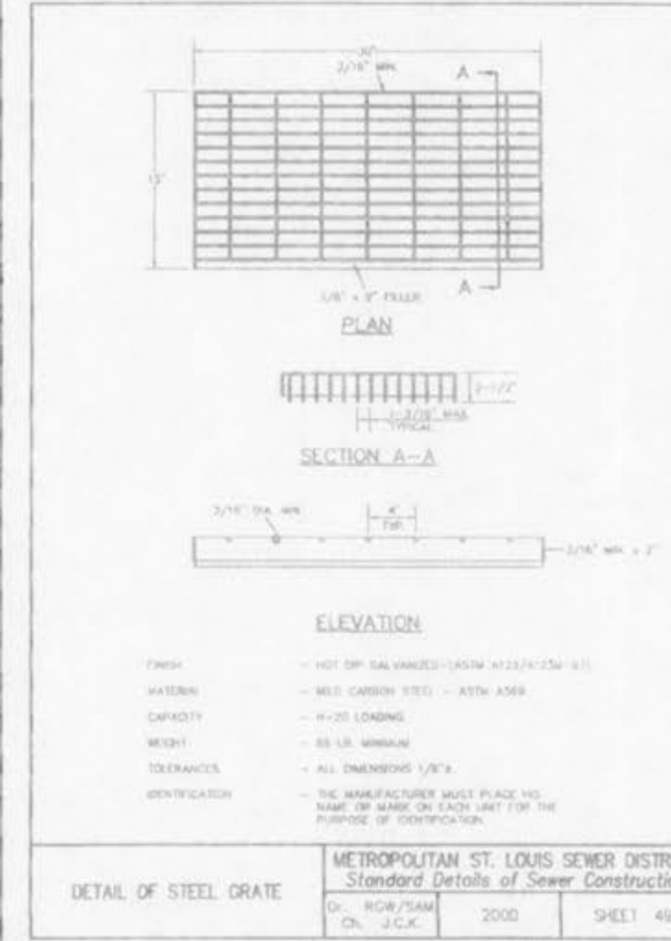
DETAIL OF STEEL GRATE METROPOLITAN ST. LOUIS SEWER DISTRICT Standard Details of Sewer Construction
