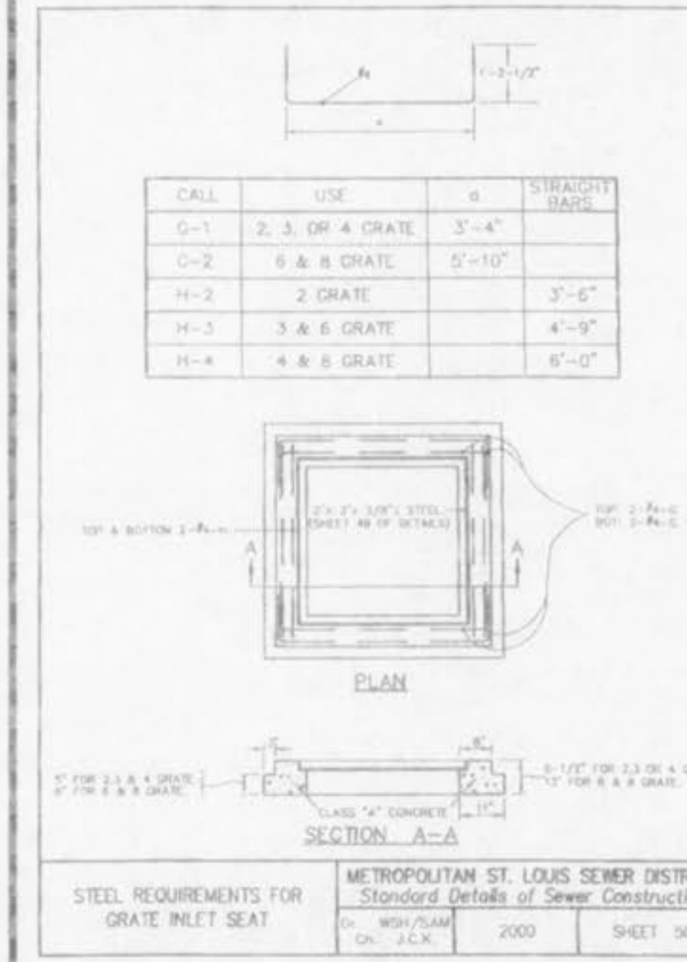
STEEL REQUIREMENTS FOR GRATE INLET SEAT METROPOLITAN ST. LOUIS SEWER DISTRICT Standard Details of Sewer Construction
