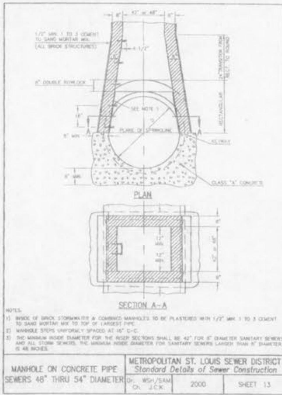
MANHOLE ON CONCRETE PIPE SEWERS 48\"/>
