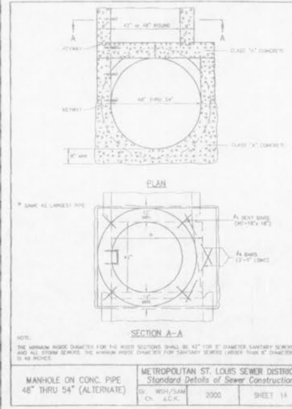
MANHOLE ON CONC. PIPE 48\"/>
