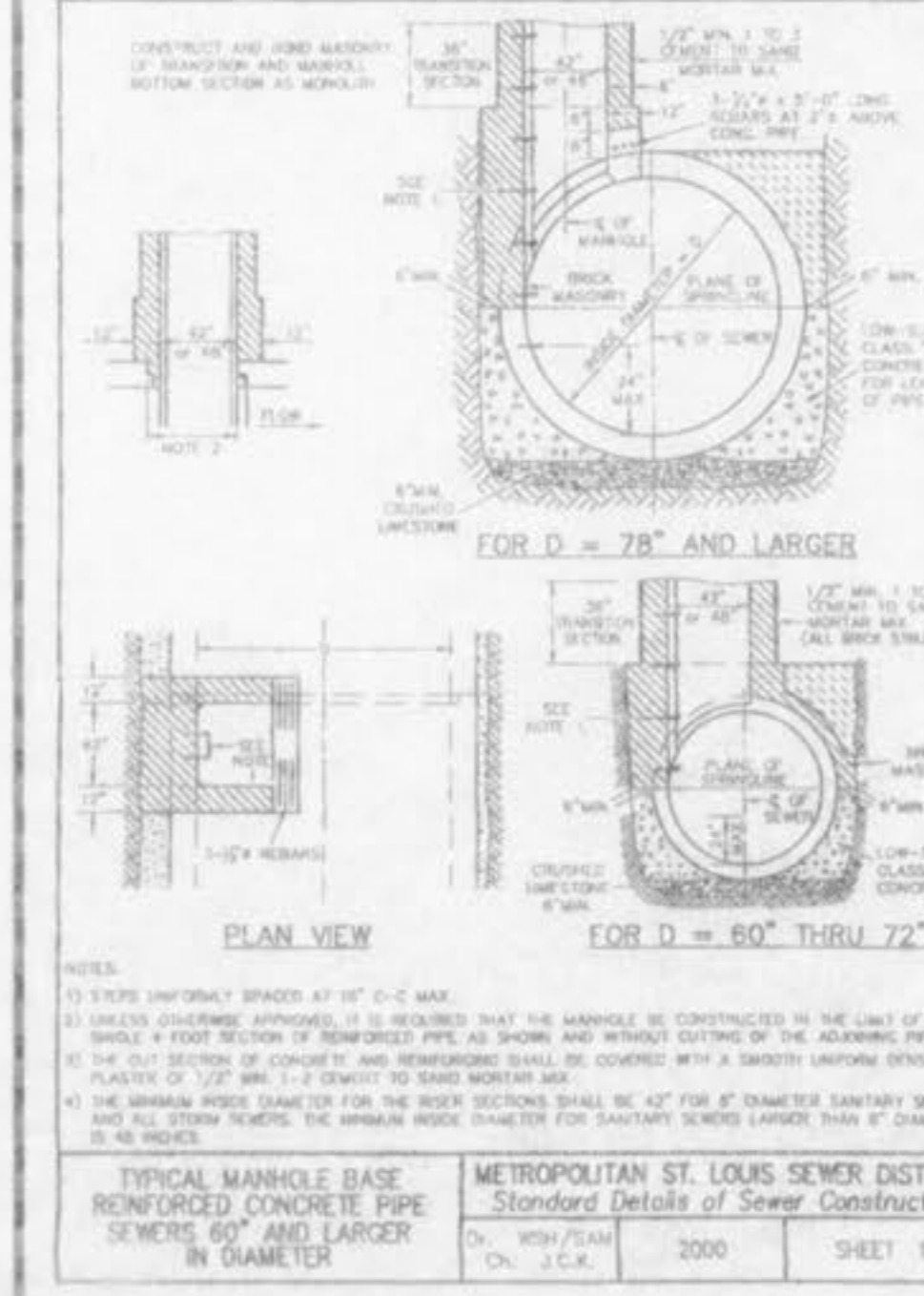
TYPICAL MANHOLE BASE REINFORCED CONCRETE PIPE SEWERS 60\"/>
