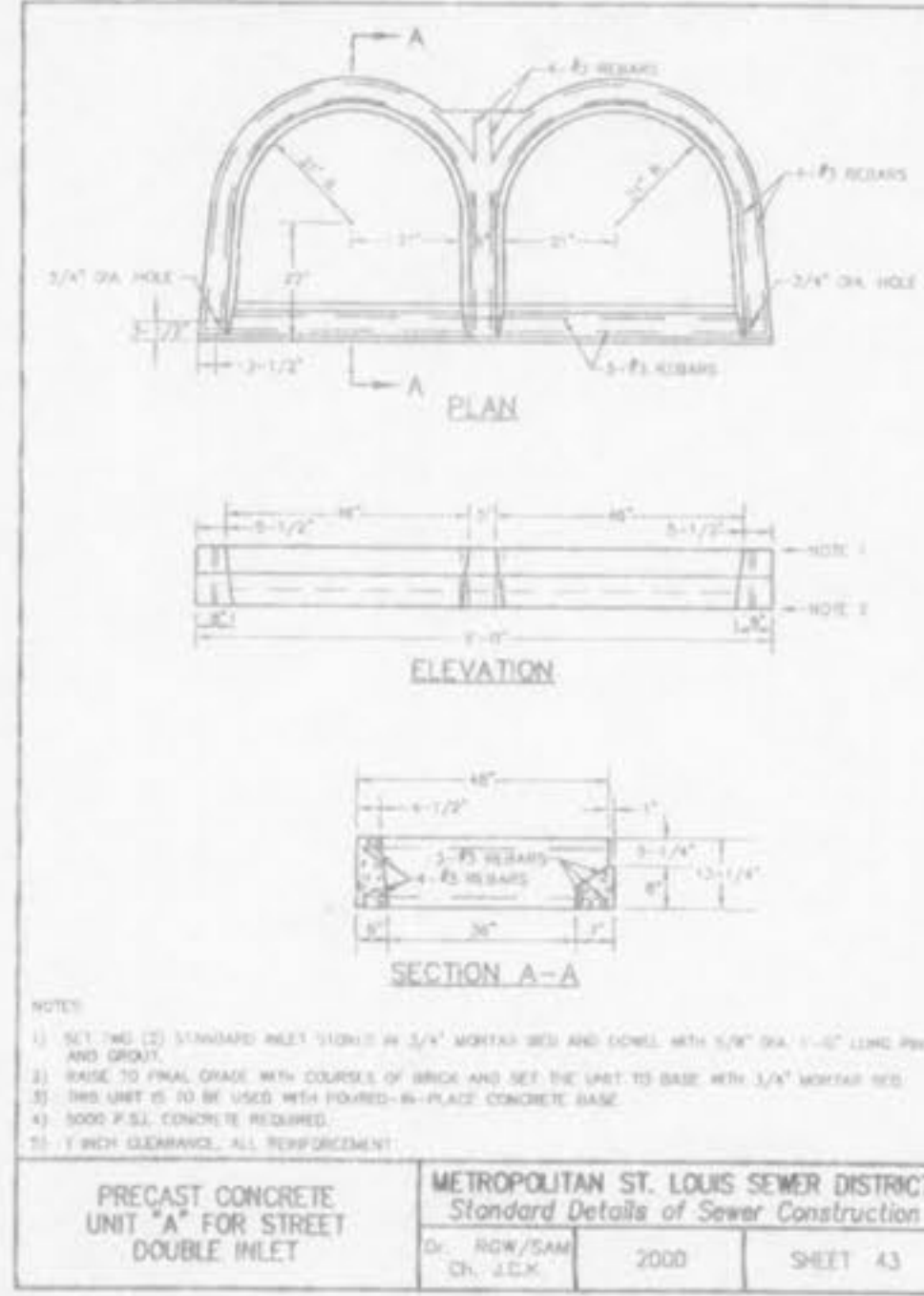
PRECAST CONCRETE UNIT "A" FOR STREET DOUBLE INLET METROPOLITAN ST. LOUIS SEWER DISTRICT Standard Details of Sewer Construction
