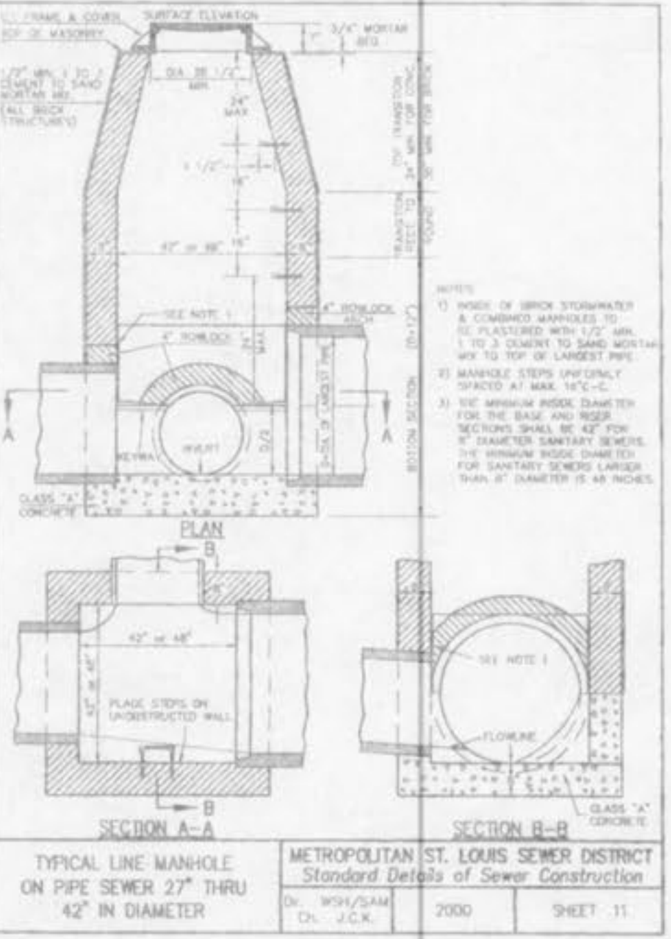
TYPICAL LINE MANHOLE ON PIPE SEWER 27\"/>
