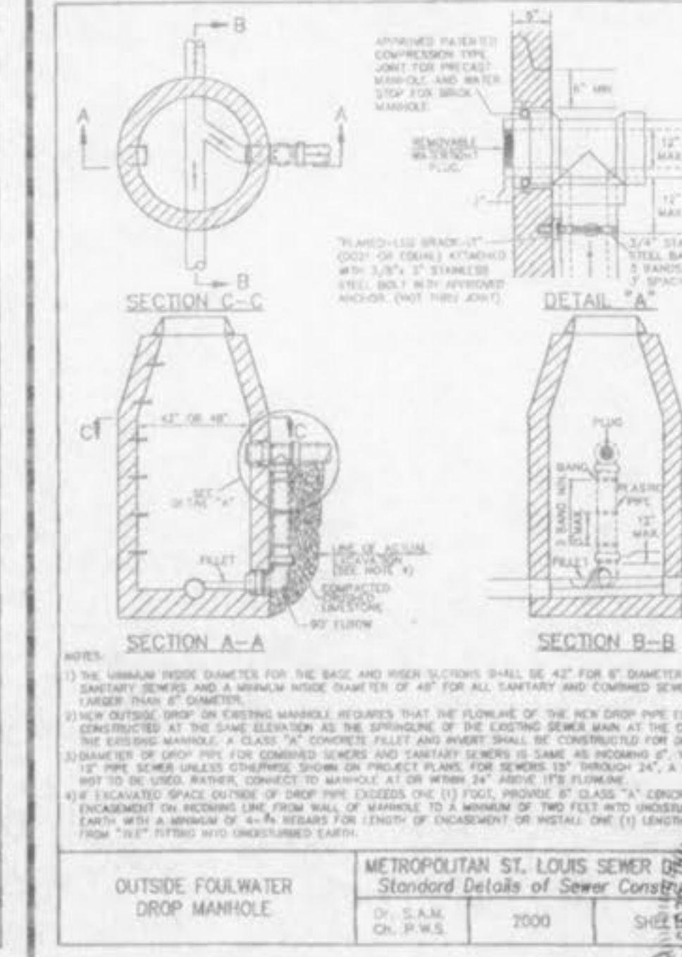
OUTSIDE FOULWATER DROP MANHOLE METROPOLITAN ST. LOUIS SEWER DISTRICT Standard Details of Sewer Construction
