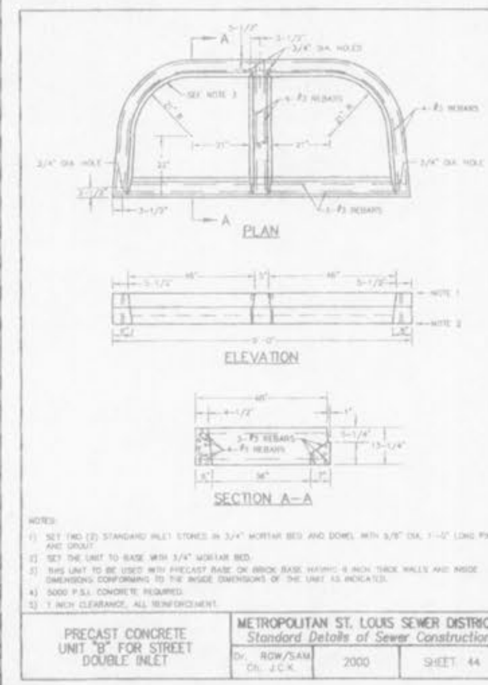
PRECAST CONCRETE UNIT "B" FOR STREET DOUBLE INLET METROPOLITAN ST. LOUIS SEWER DISTRICT Standard Details of Sewer Construction
