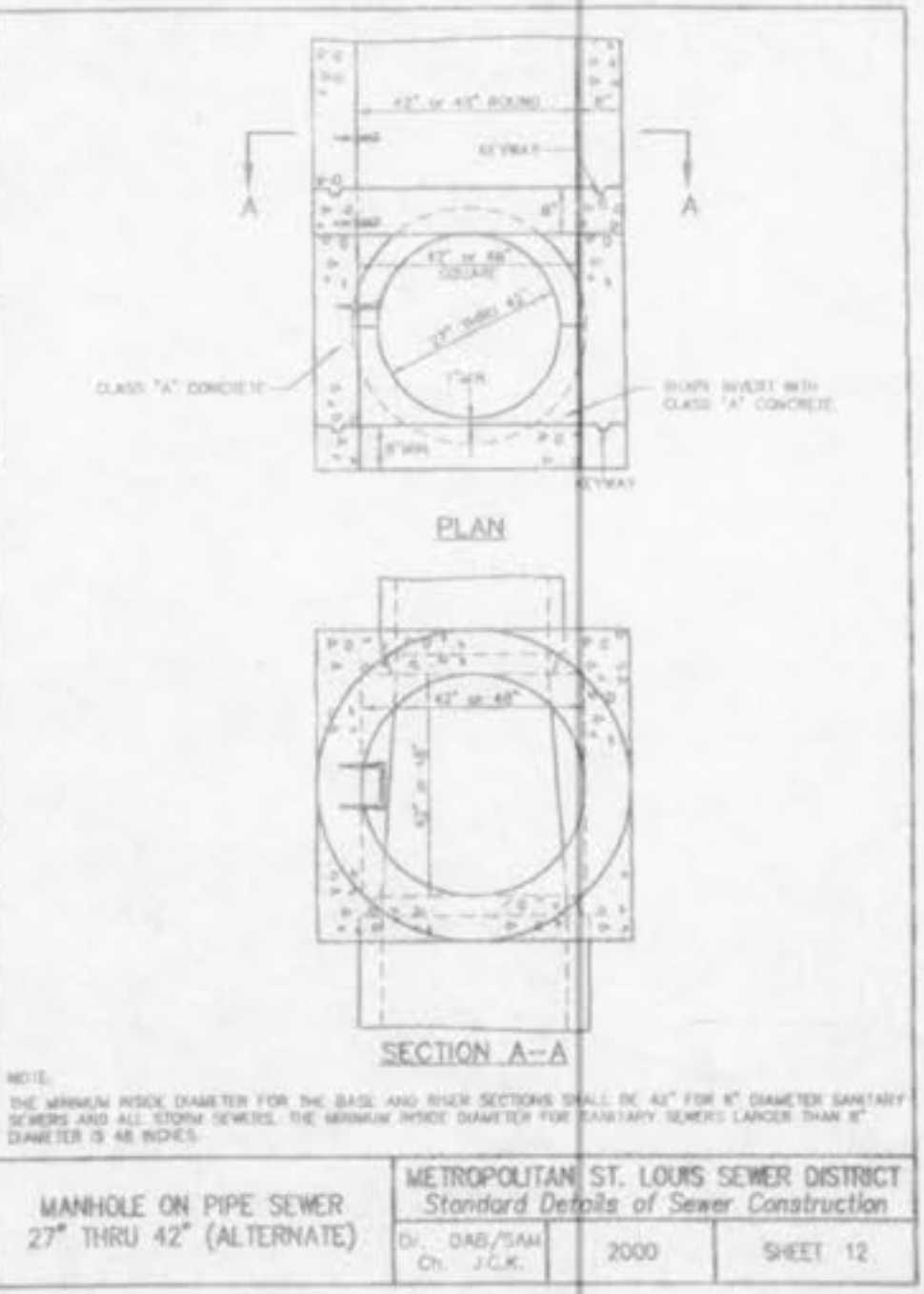
MANHOLE ON PIPE SEWER 27\"/>
