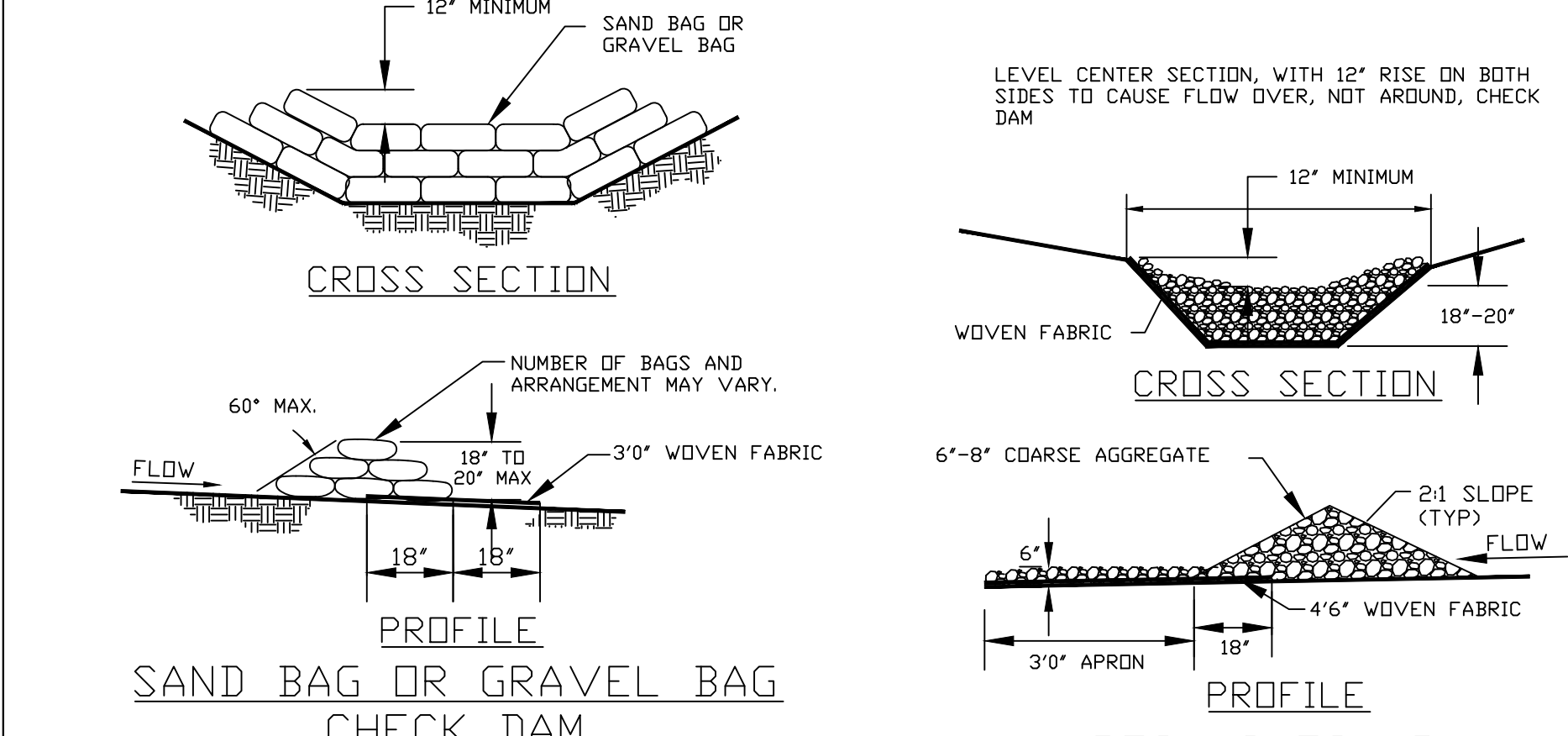
CITY OF O'FALLON ENGINEERING DEPARTMENT O'FALLON, MISSOURI CHECK DAMS
