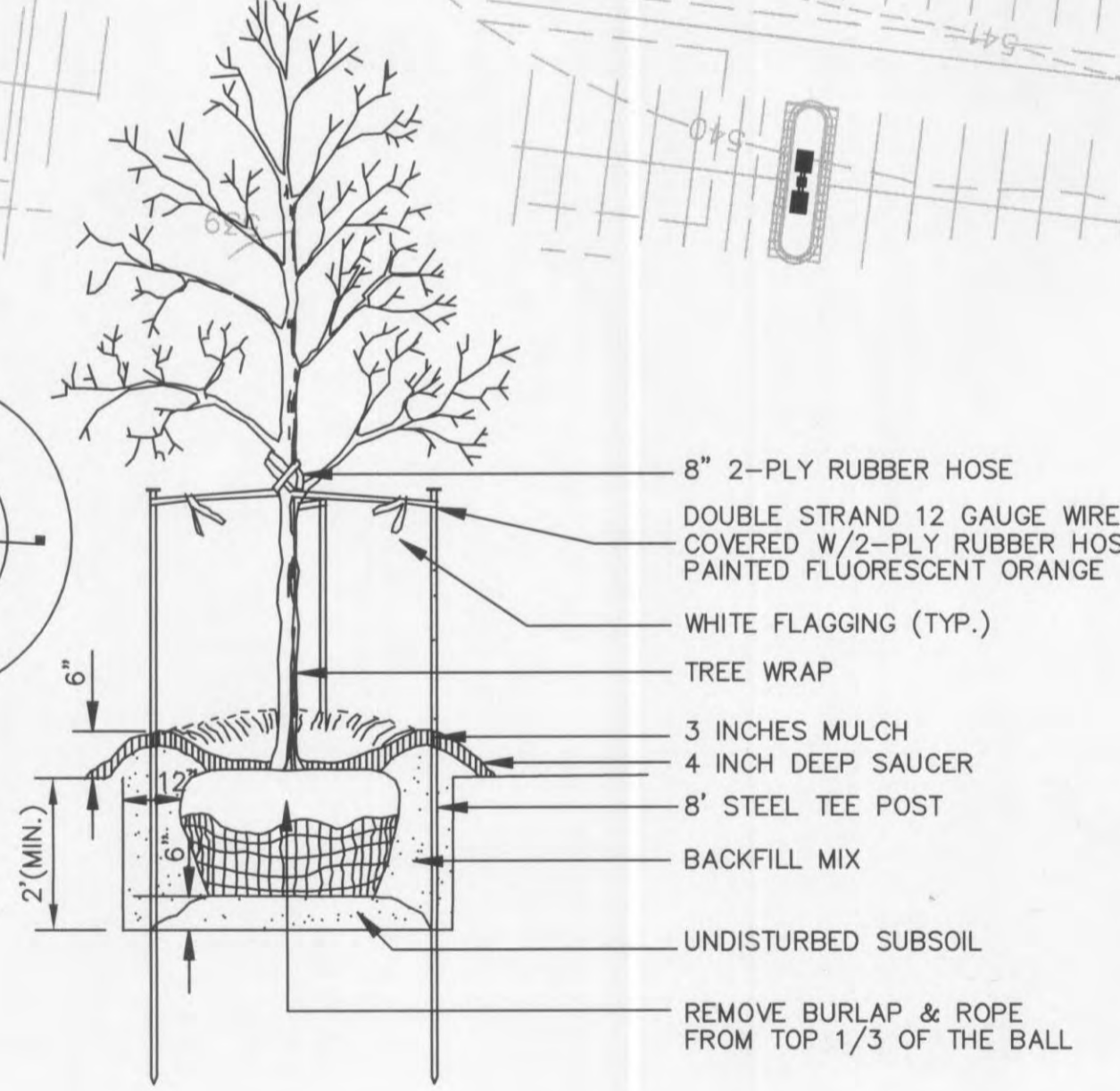
DECIDUOUS TREE PLANTING N.T.S.
