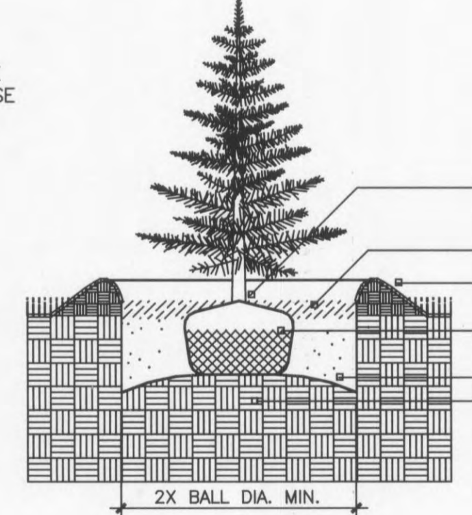
EVERGREEN TREE PLANTING N.T.S.
