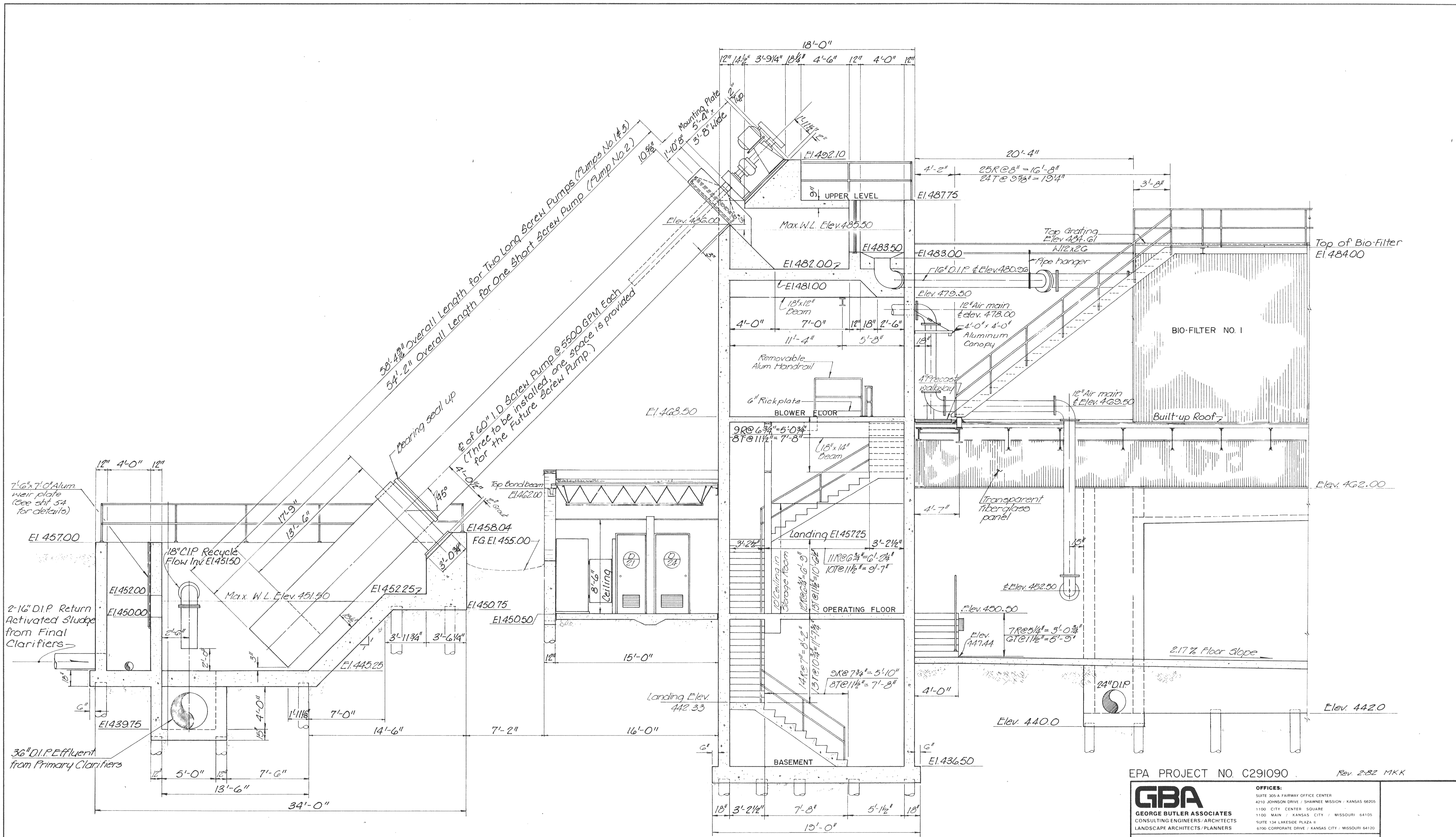
LONGITUDINAL SECTION OF BIO-FILTER COMPLEX
