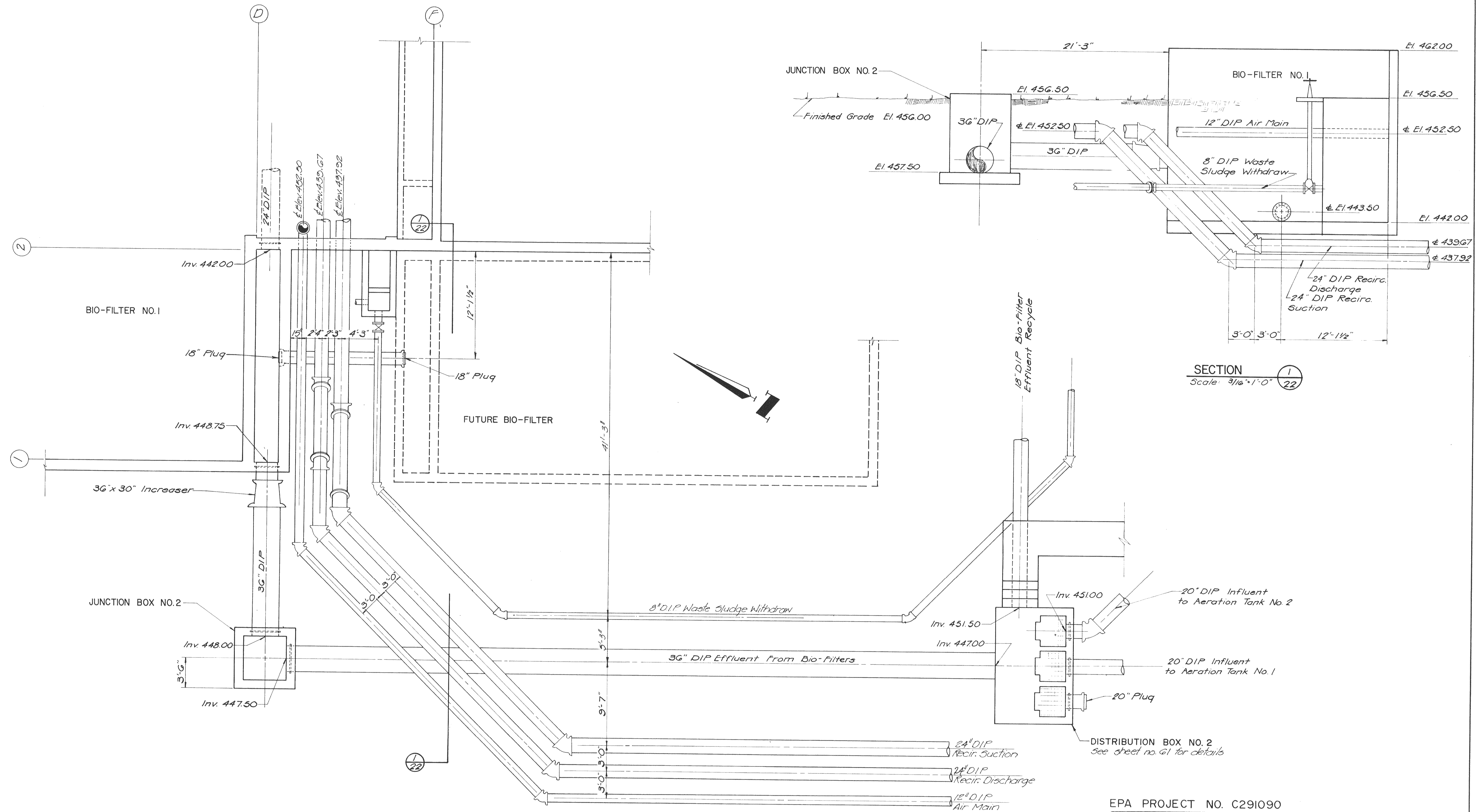
PARTIAL SITE PIPING PLAN — WEST OF BIO-FILTER COMPLEX Scale: 3/16" = 1'-0"
