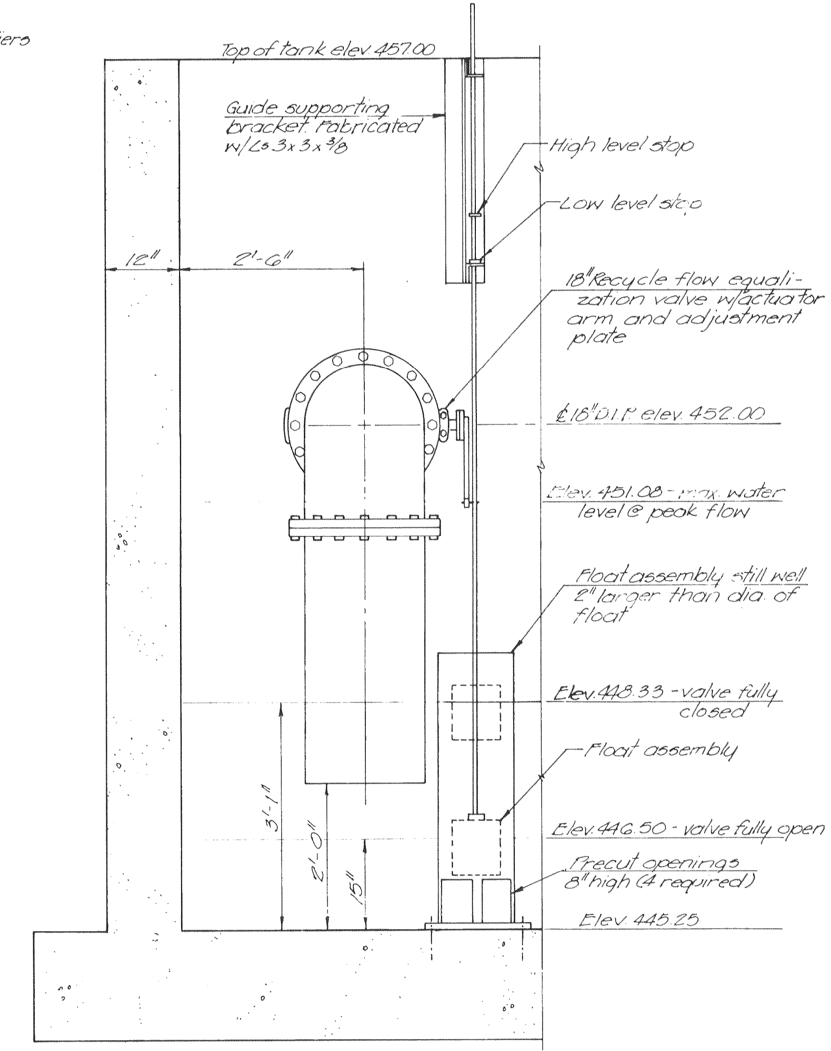
SECTION 1/37 Scale: 3/4" = 1'-0"
