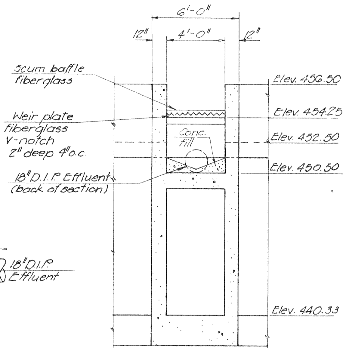
SECTION A Scale: 1/4" = 1'-0" (41) (Re. sht. 40)
