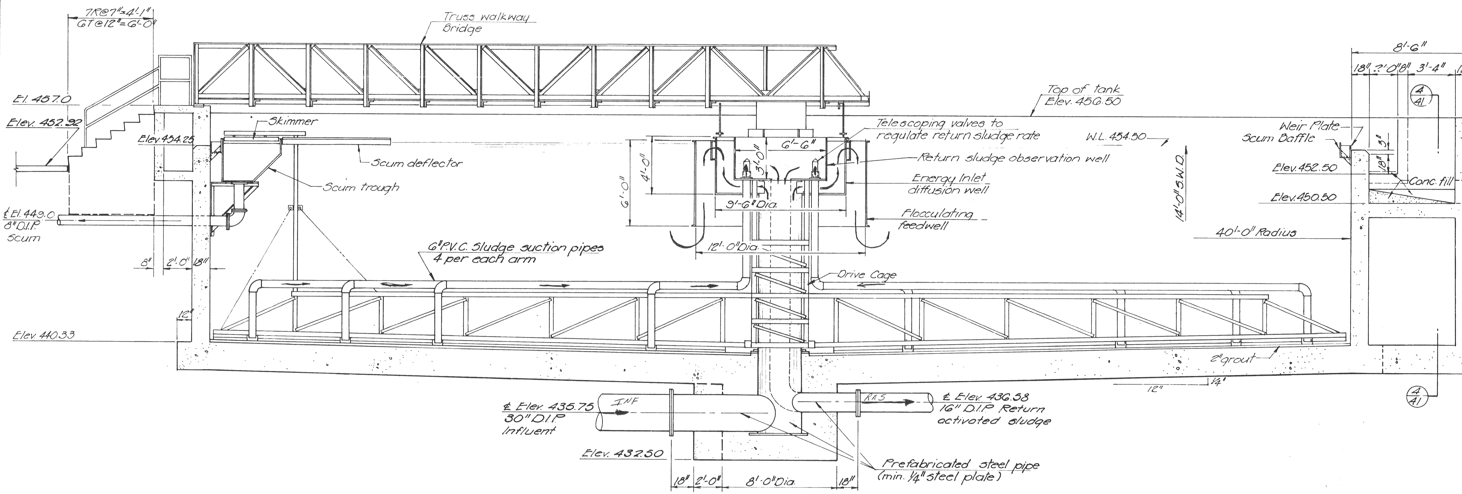
TYPICAL FINAL CLARIFIER
