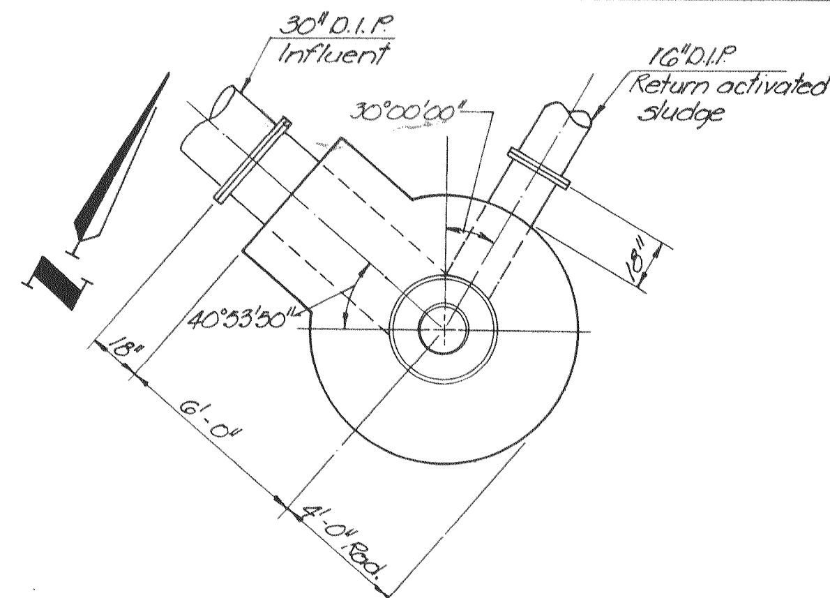
FINAL CLARIFIER NO. 2 FOUNDATION PLAN Scale: 1/4" = 1'-0"
