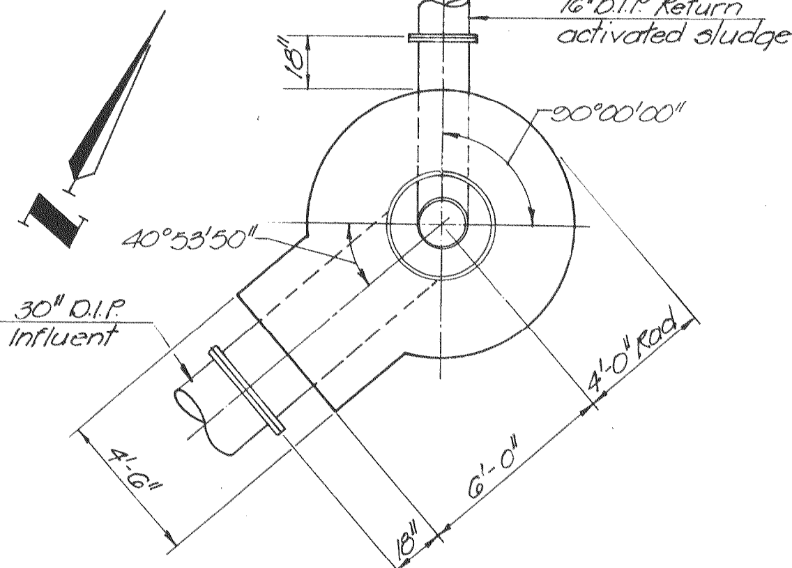
FINAL CLARIFIER NO. 1 FOUNDATION PLAN Scale: 1/4" = 1'-0"
