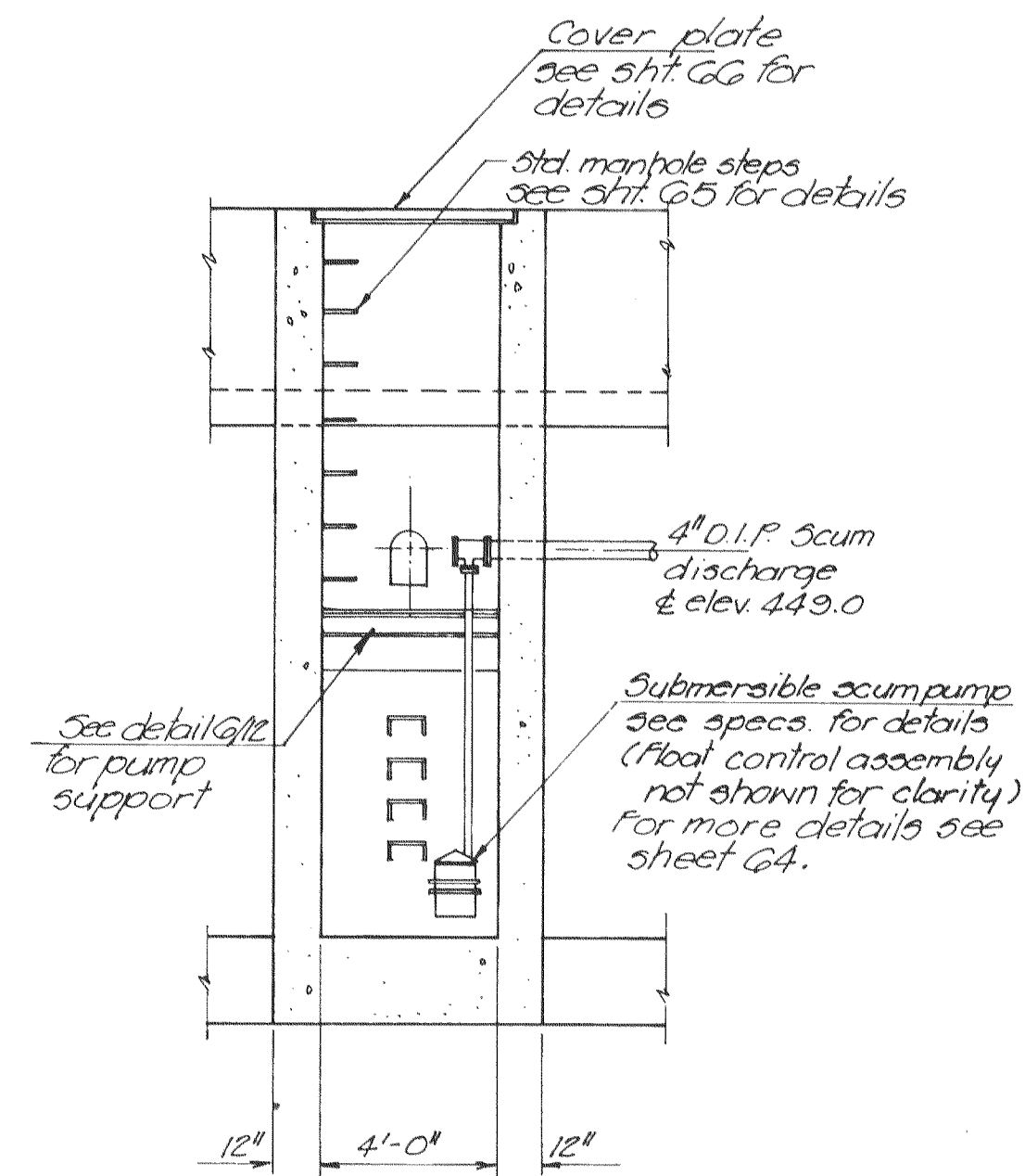
SECTION 3 Scale: 1/4" = 1'-0" (41) (Re. sht. 40)
