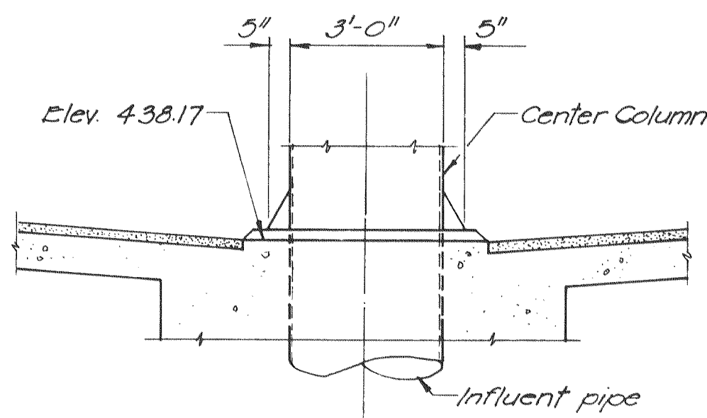
CENTER COLUMN SUPPORT Scale: 1/2" = 1'-0"
