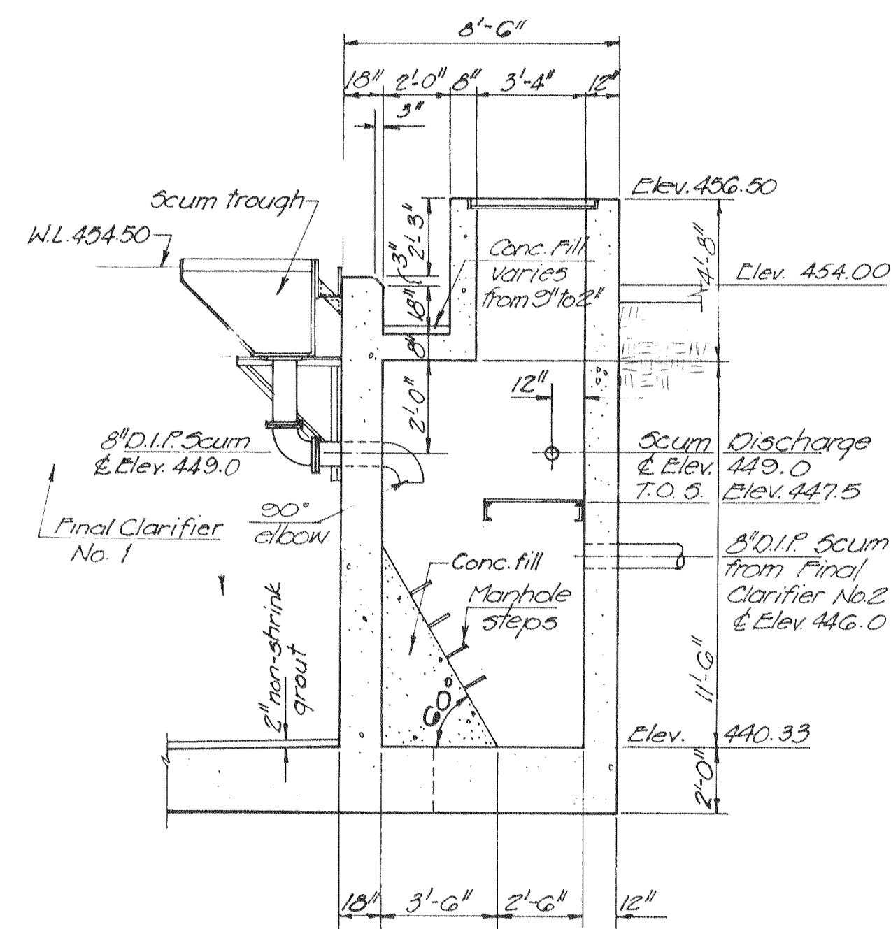
SECTION 2 Scale: 1/4" = 1'-0" (41) (Re. sht. 40)
