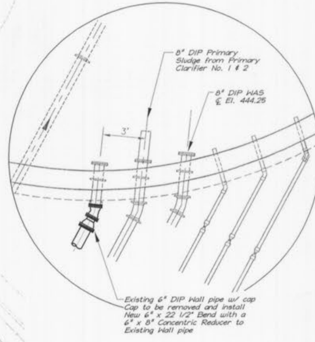
1 60.13 DETAIL SCALE: 1/4" = 1'-0"
