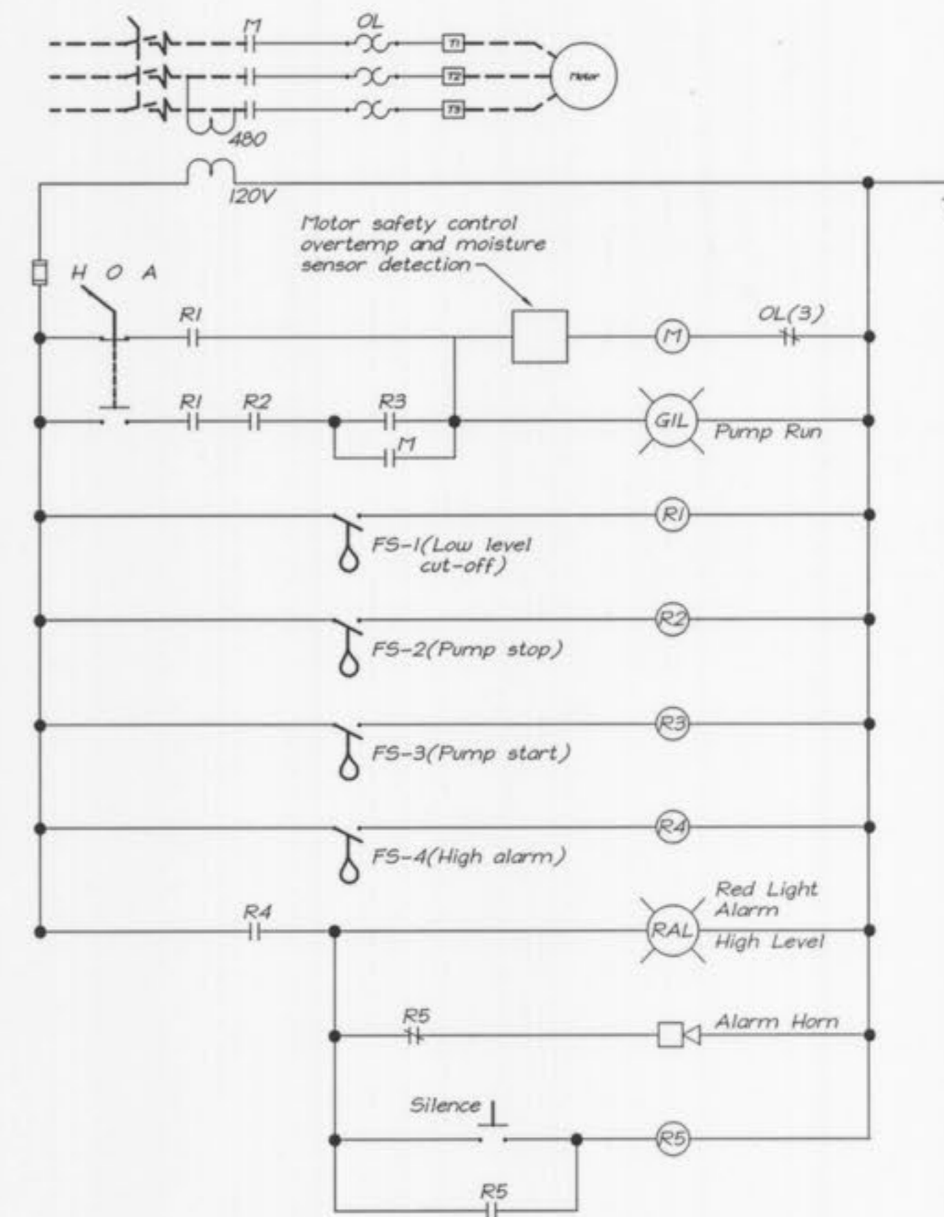
SCUM PUMP CONTROL SCHEMATIC NO SCALE
