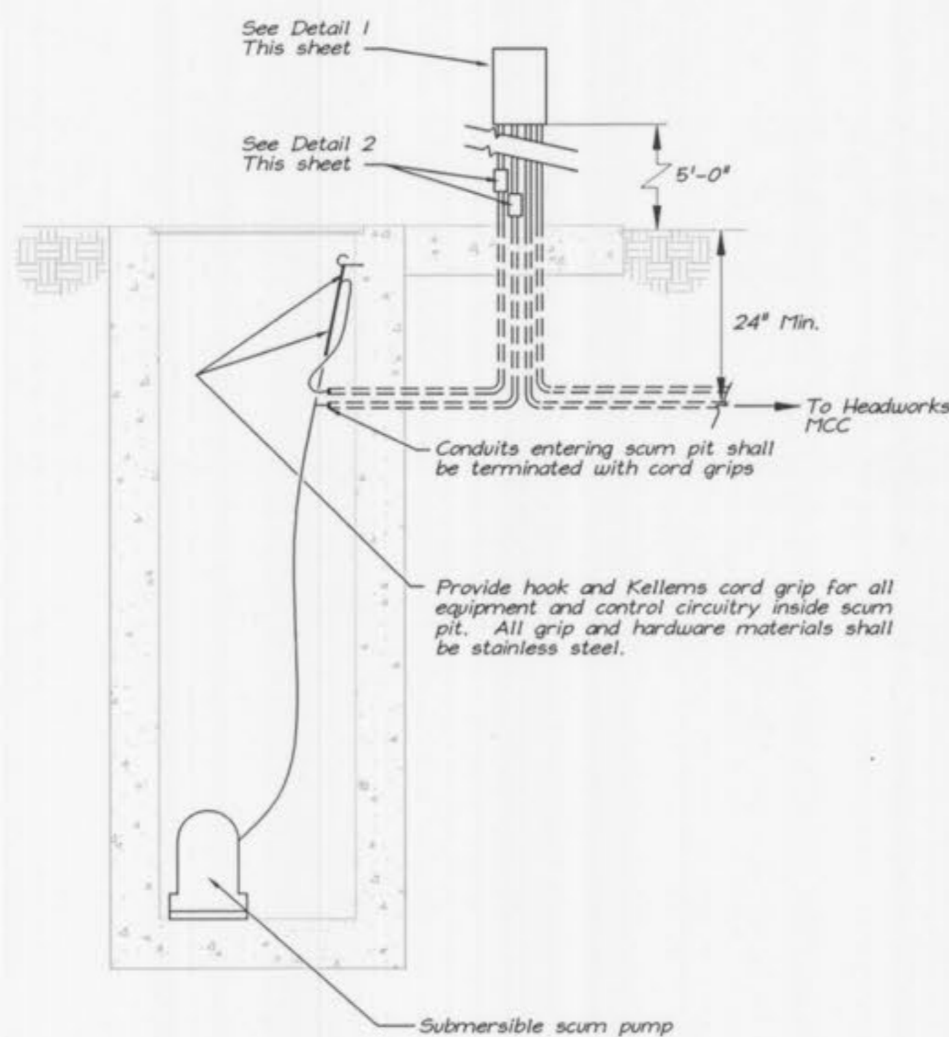
EQUIPMENT INSTALLATION SECTION - SCUM PITS 3 & 4 (PIT 3 IS EXISTING FOR RETROFIT, PIT 4 IS NEW)
