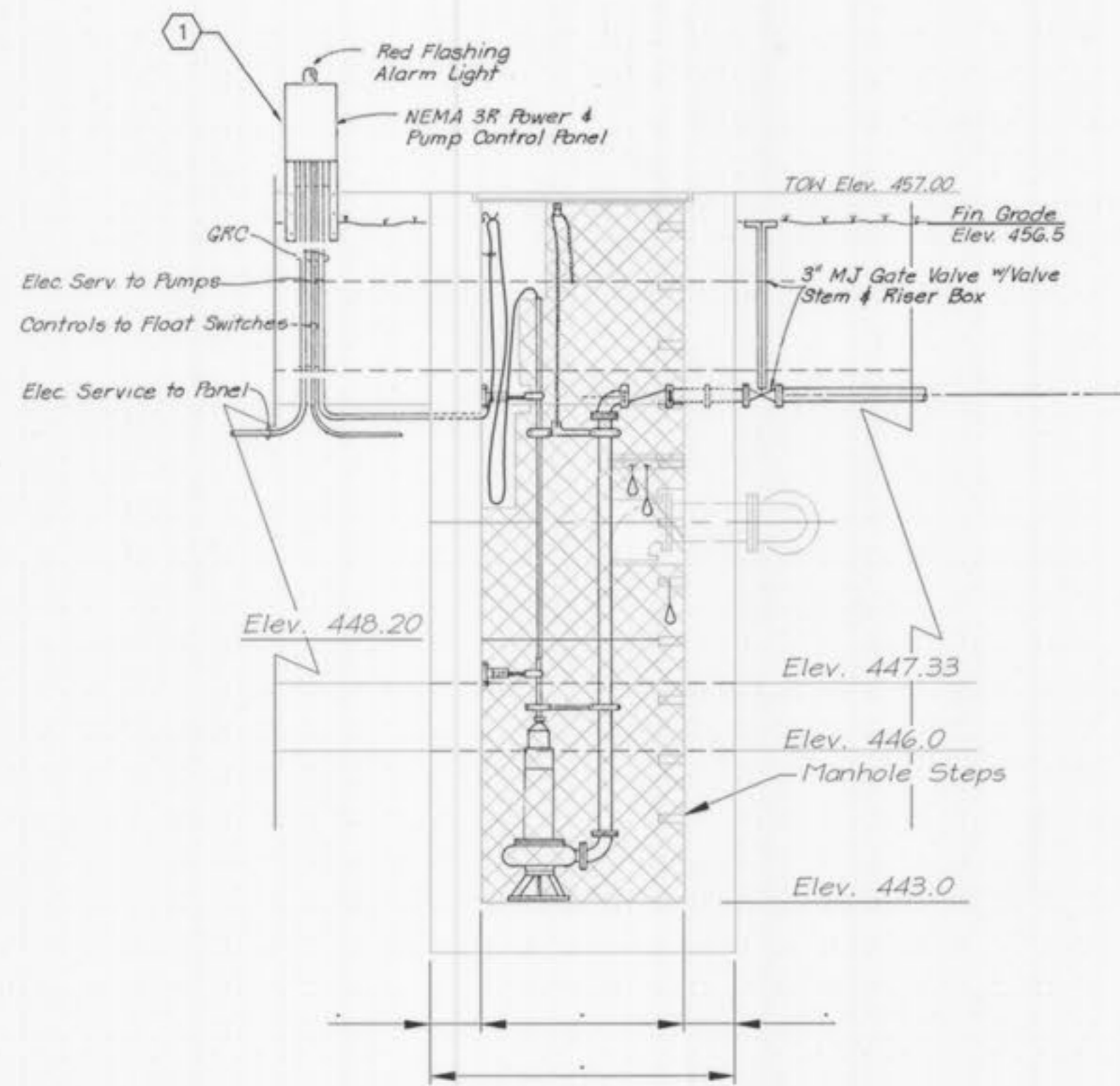
DEMOLITION SECTION - SCUM PIT 3 (PRIMARY CLARIFIER 3 SCUM PIT) SCALE 3/8" = 1'-0" (Piping and equipment locations shown out of rotation. Exact locations vary slightly from that shown.)
