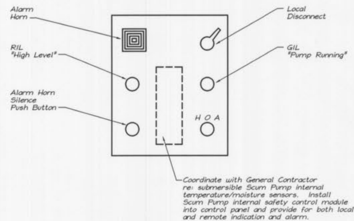
DETAIL 1 SCUM PUMP CONTROL PANEL (TYP.) NO SCALE
