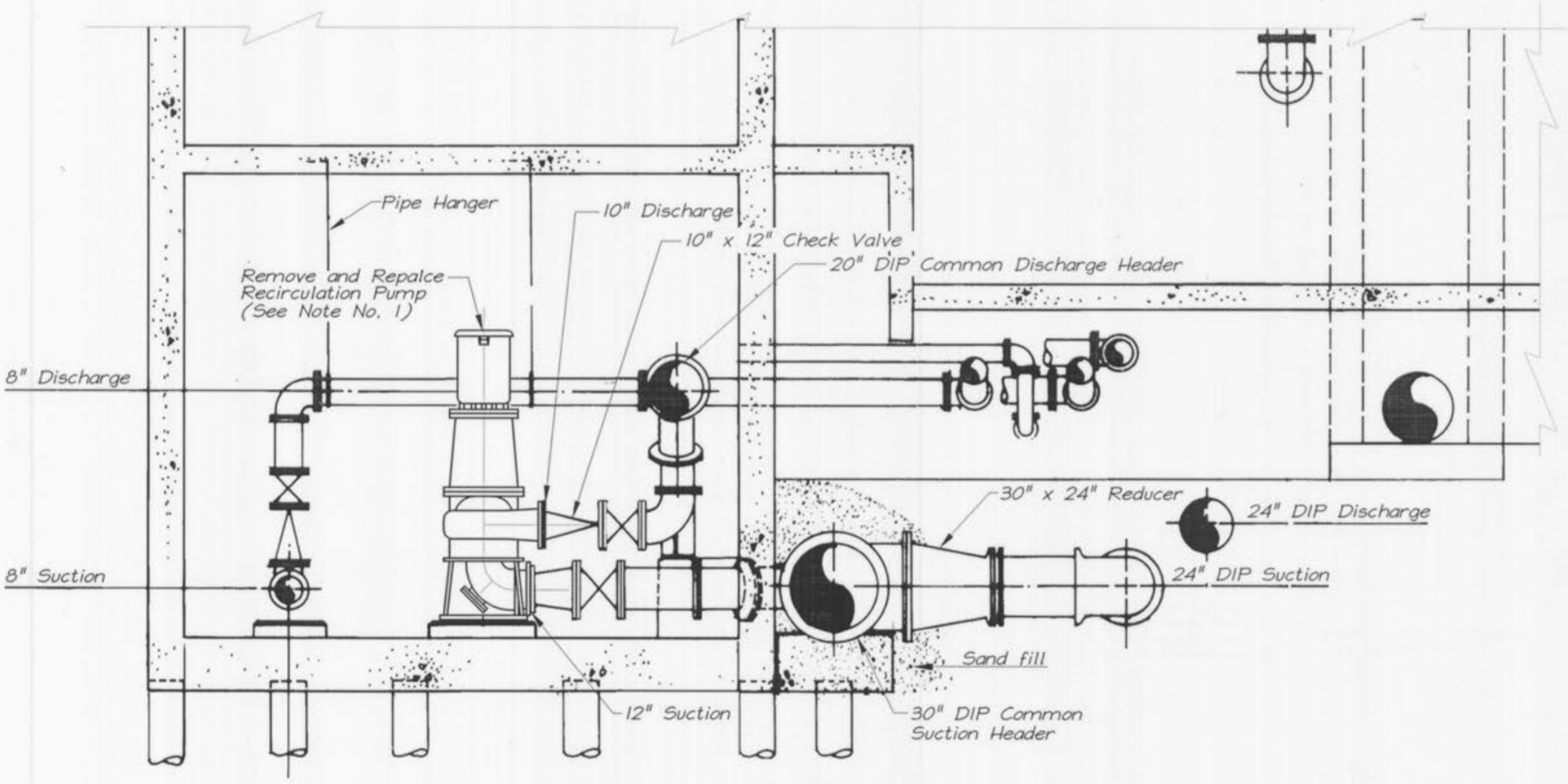
SECTION 1 SCALE : 3/8" = 1'-0"
