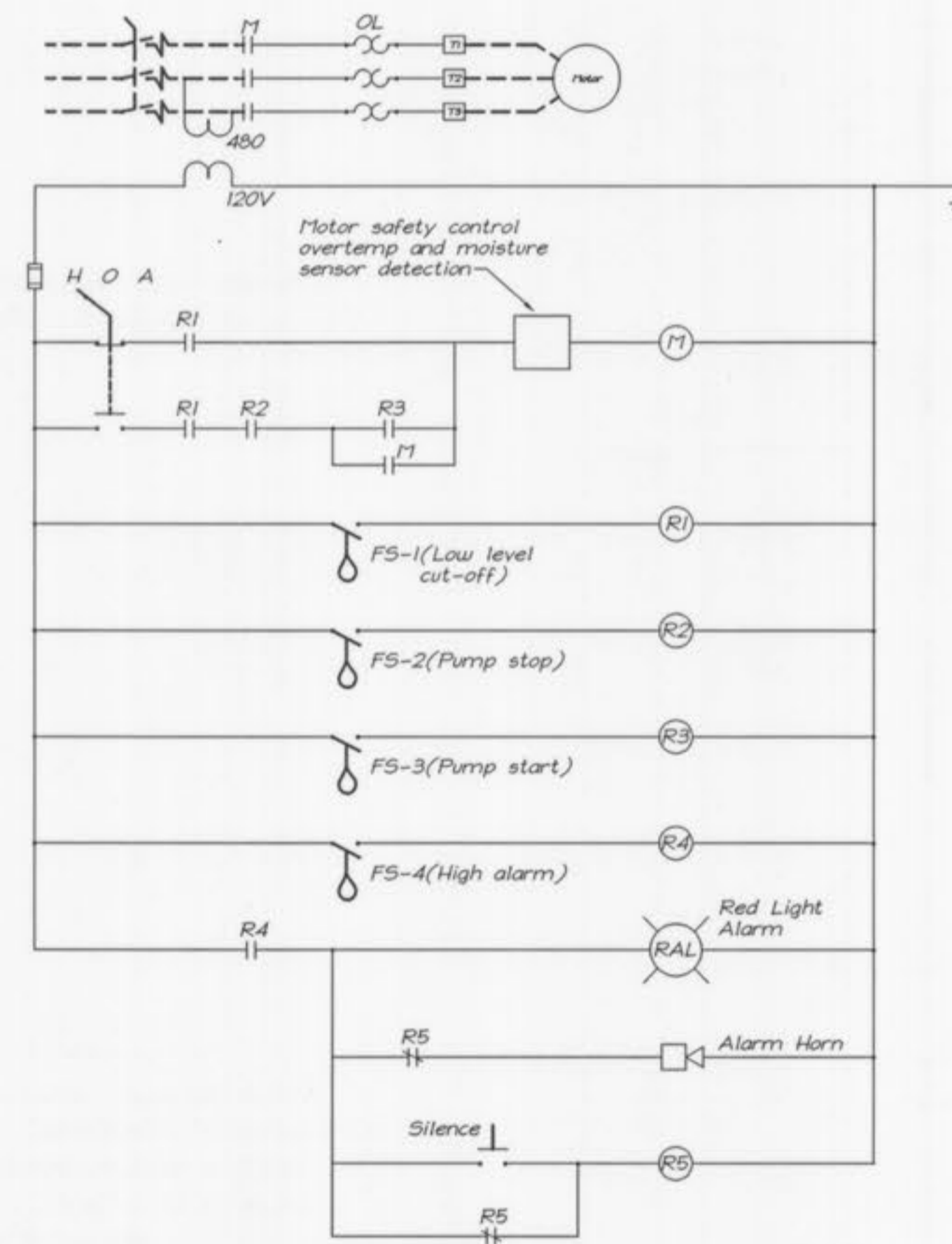
SCUM PUMP CONTROL SCHEMATIC NO SCALE
