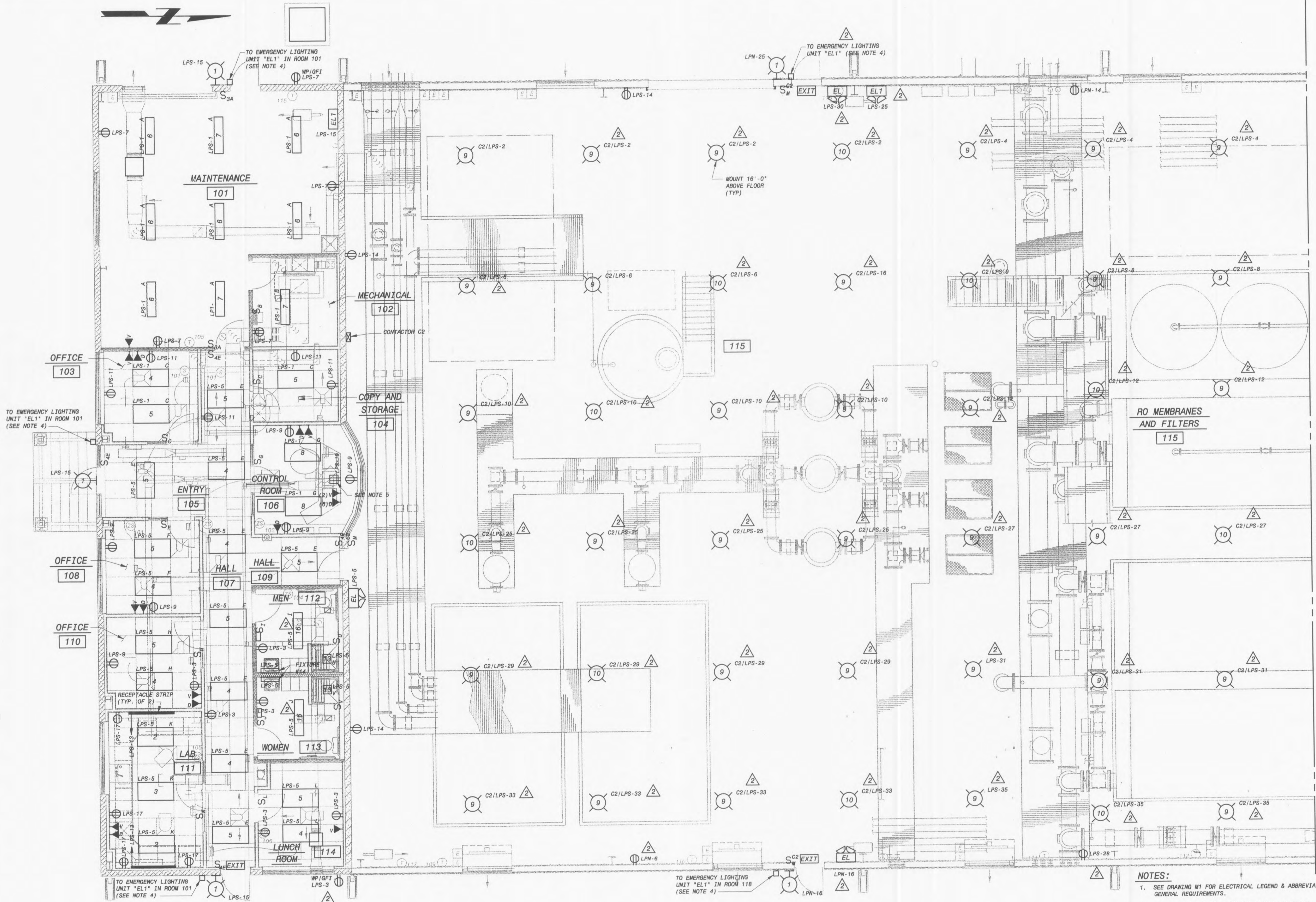
PARTIAL LIGHTING PLAN 3/16" = 1'-0"
