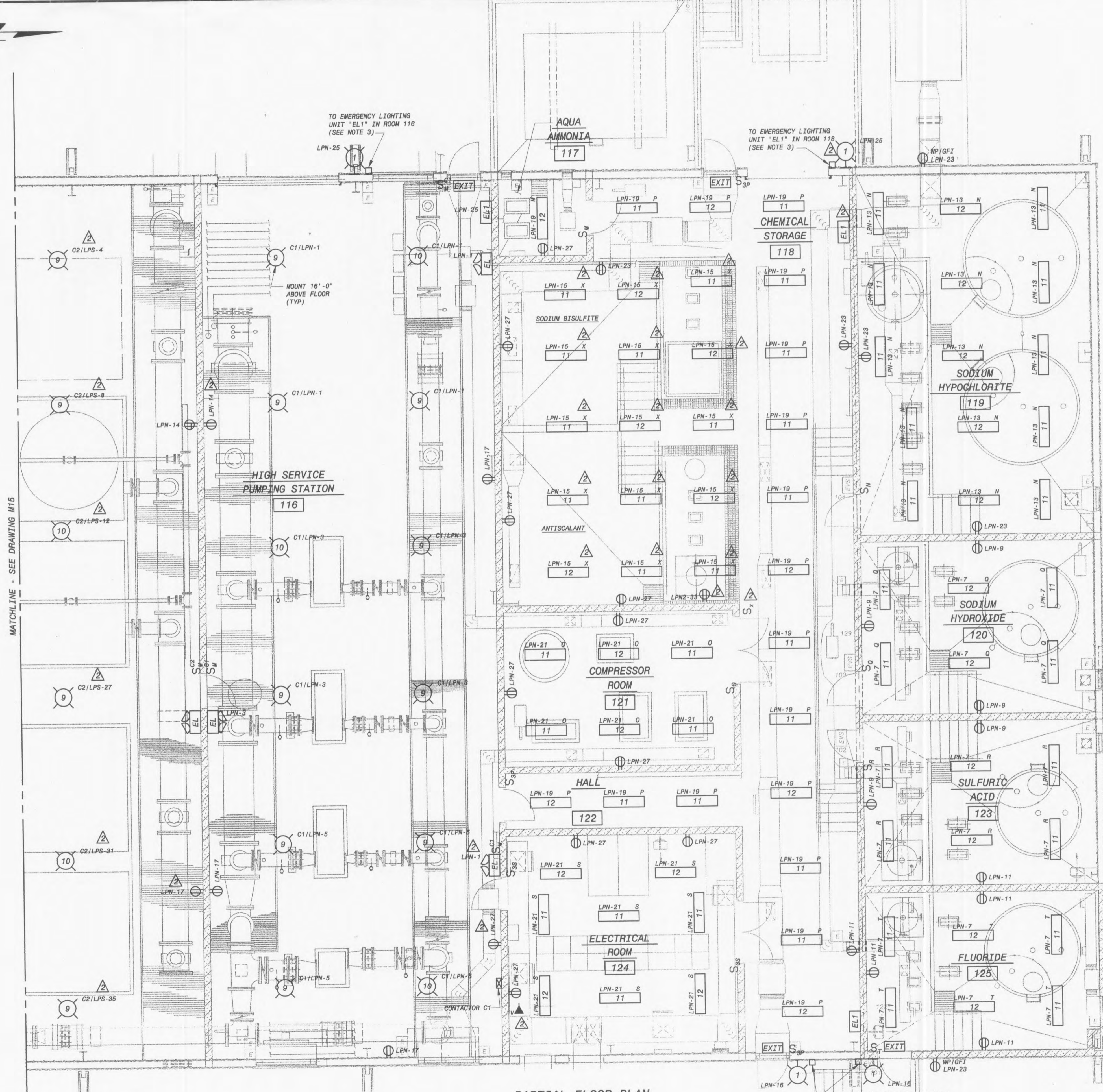
PARTIAL FLOOR PLAN 3/16" = 1' - 0"
