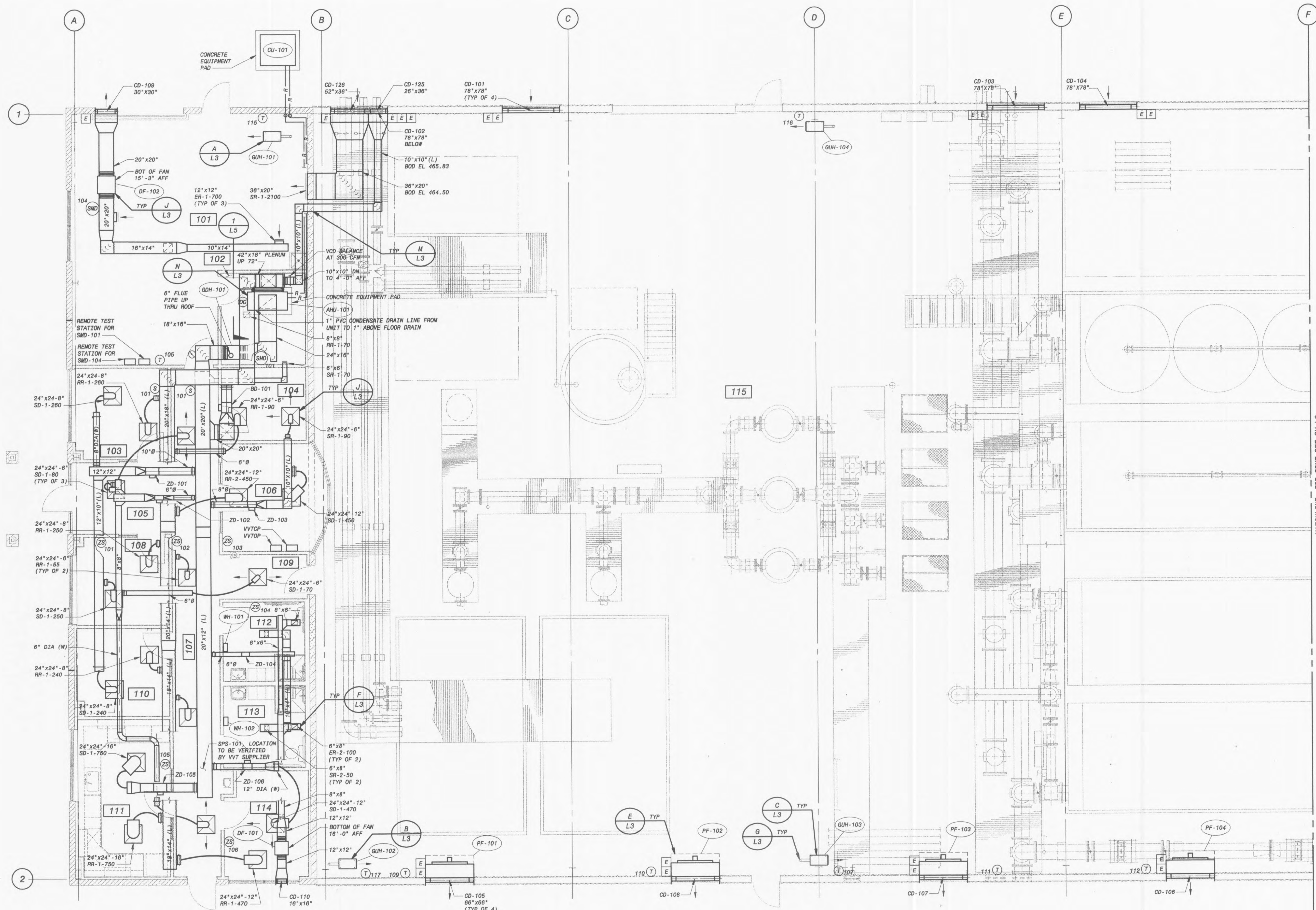
PARTIAL OPERATIONS BUILDING FLOOR PLAN - SOUTH 3/16" = 1'-0"
