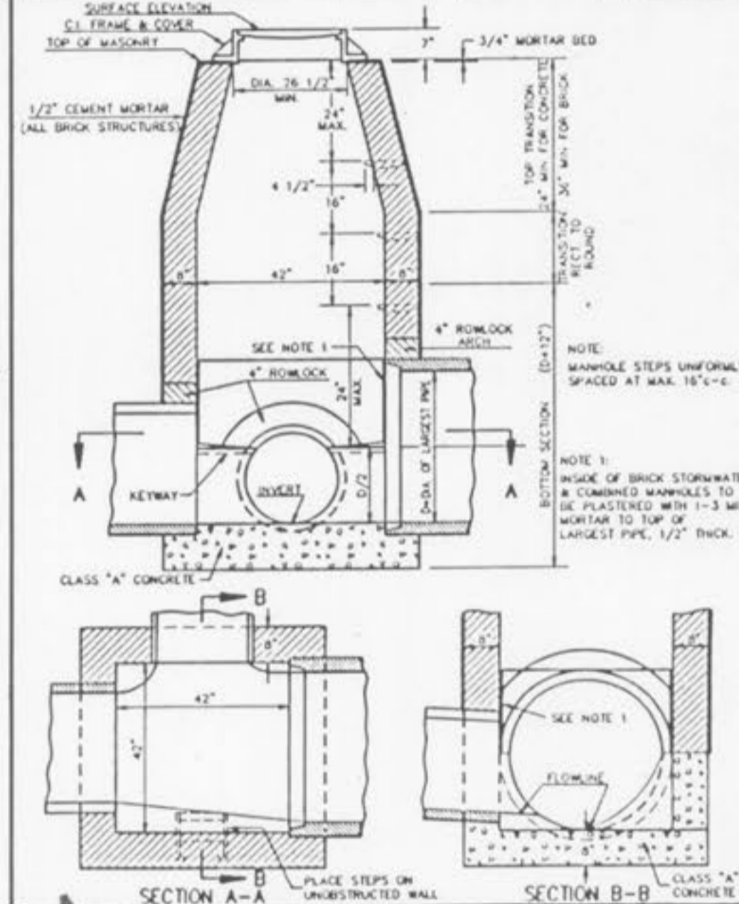
TYPICAL LINE MANHOLE ON PIPE SEWER 27" THRU 36" DIA. METROPOLITAN ST. LOUIS SEWER DISTRICT Standard Details of Sewer Construction Dr. W.S.H. Ch. J.C.K. 1992 SHEET 9
