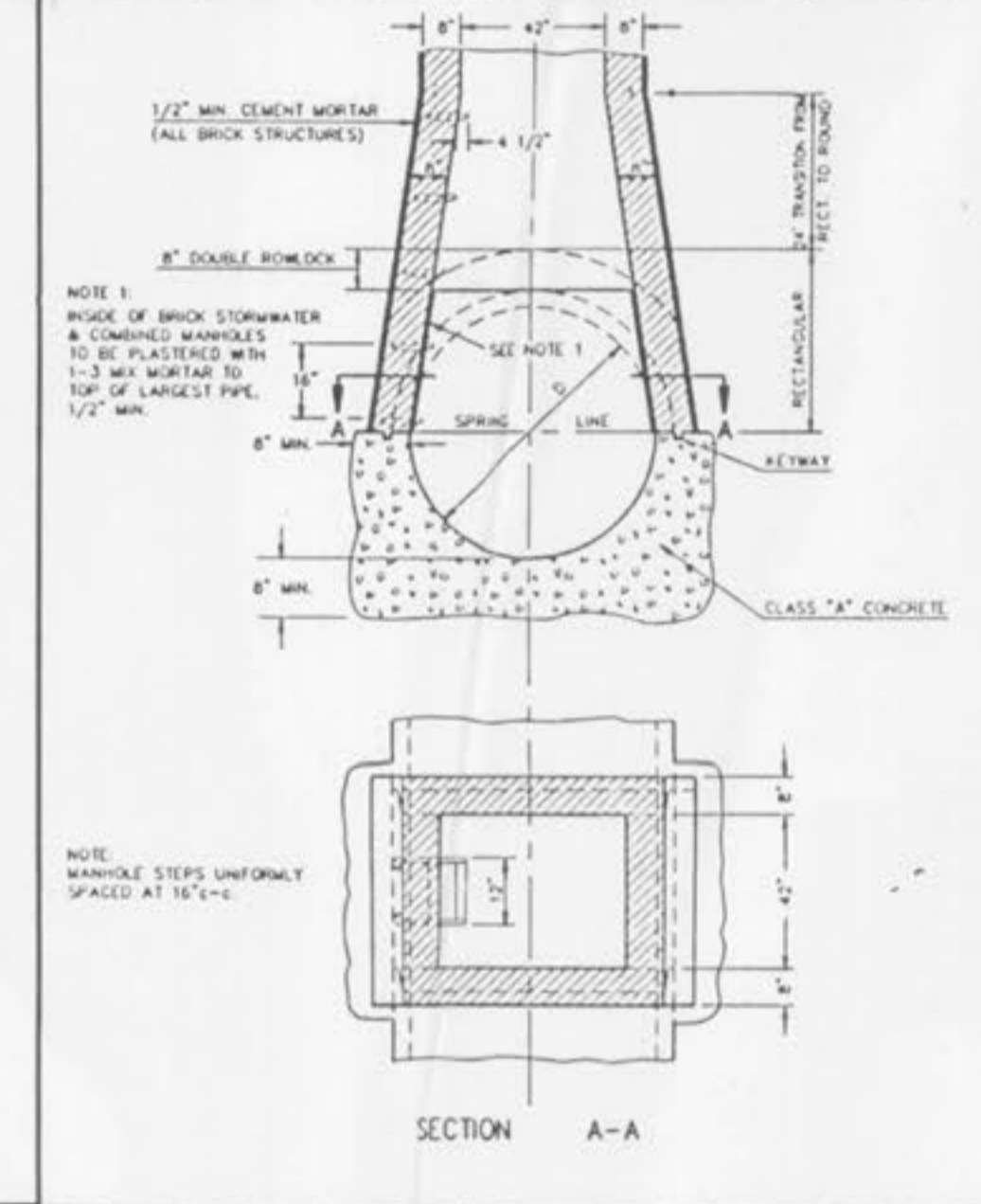
MANHOLE ON CONCRETE PIPE SEWERS 39" THRU 54" DIA. METROPOLITAN ST. LOUIS SEWER DISTRICT Standard Details of Sewer Construction Dr. W.S.H. Ch. J.C.K. 1992 SHEET 11
