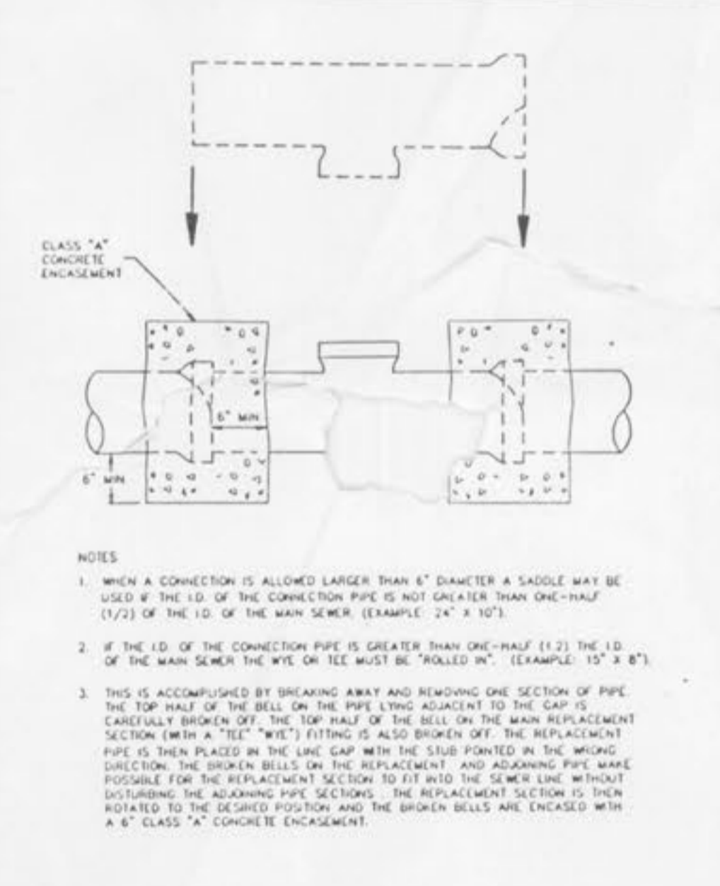
"RIROLL-IN" (FOR EXISTING CLAY OR CONCRETE PIPE) METROPOLITAN ST. LOUIS SEWER DISTRICT Standard Details of Sewer Construction Dr. D.A.B. Ch. J.C.K. 1992 SHEET 63
