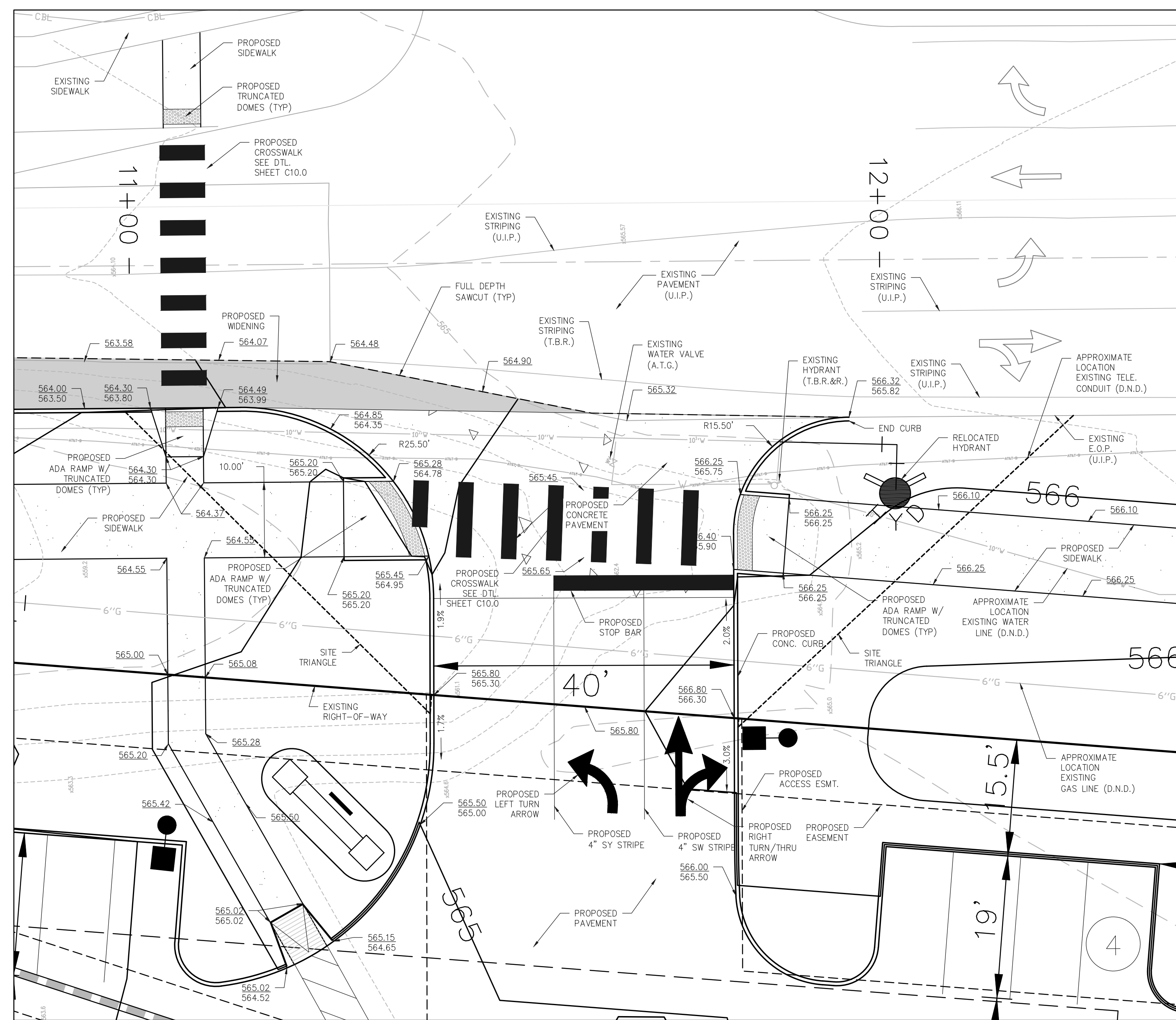
SOUTH ENTRANCE - PLAN VIEW SCALE: 1" = 10'
