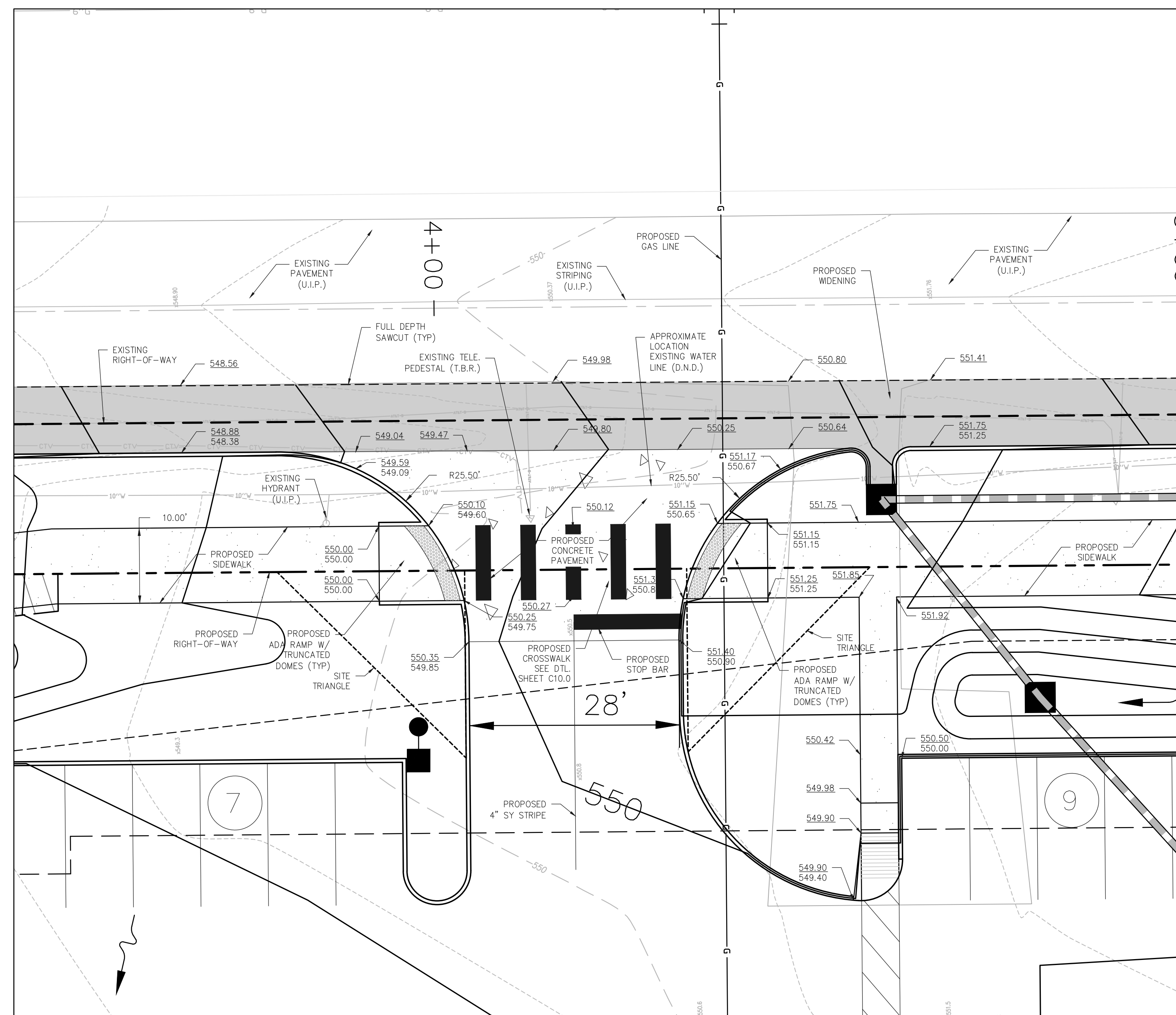
NORTH ENTRANCE - PLAN VIEW SCALE: 1" = 10'
