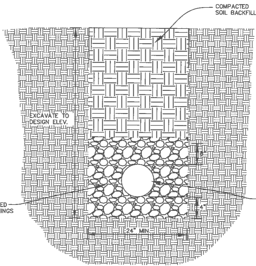
FRENCH DRAIN OUTLET PIPE DETAIL N.T.S.
