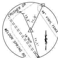
CONTROL POINT NO. 3 SET IRON ROD N: 1051259.669 E: 761418.486 EL: 543.13
