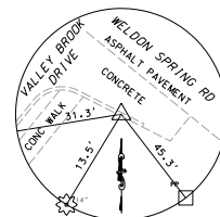
CONTROL POINT NO. 4 CROSS N: 1051799.354 E: 761083.544 EL: 507.59
