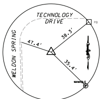
CONTROL POINT NO. 1 IRON PIPE W/CAP N: 1050091.169 E: 762059.895 EL: 565.74
