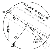
CONTROL POINT NO. 2 CROSS N: 1050753.790 E: 761615.541 EL: 560.00
