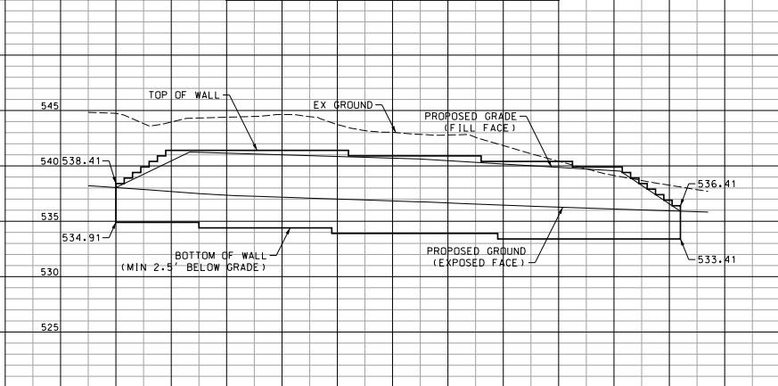
RETAINING WALL 2 PROFILE LENGTH = 102.00' AREA = 660.00 SF
