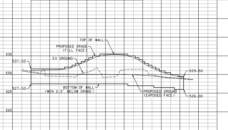
RETAINING WALL 3 PROFILE LENGTH = 82.00' AREA = 467.50 SF
