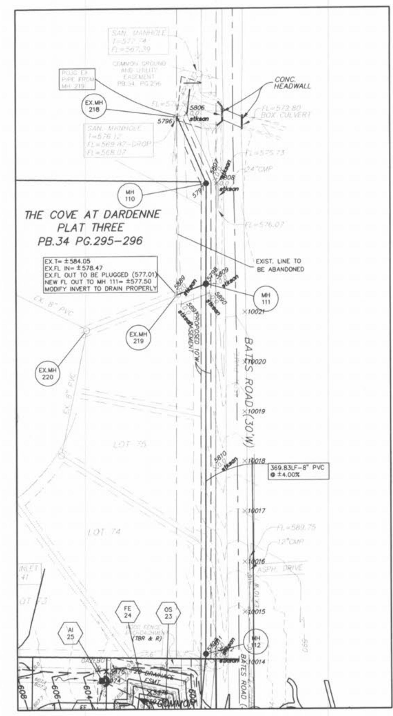
OFFSITE SANITARY SEWER
