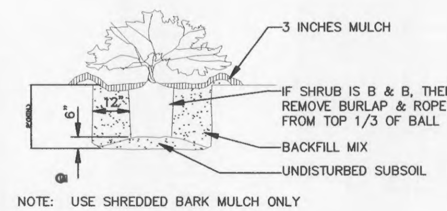
SHRUB PLANTING N.T.S.
