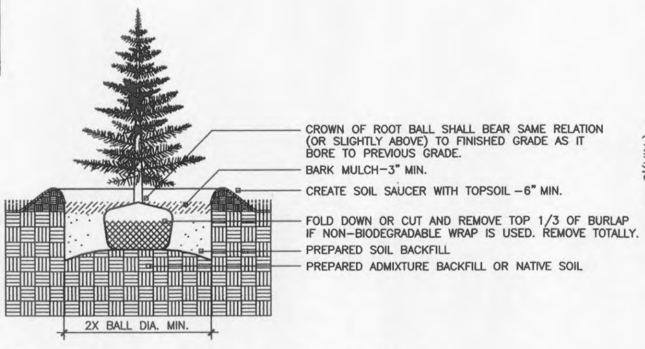
EVERGREEN TREE PLANTING N.T.S.
