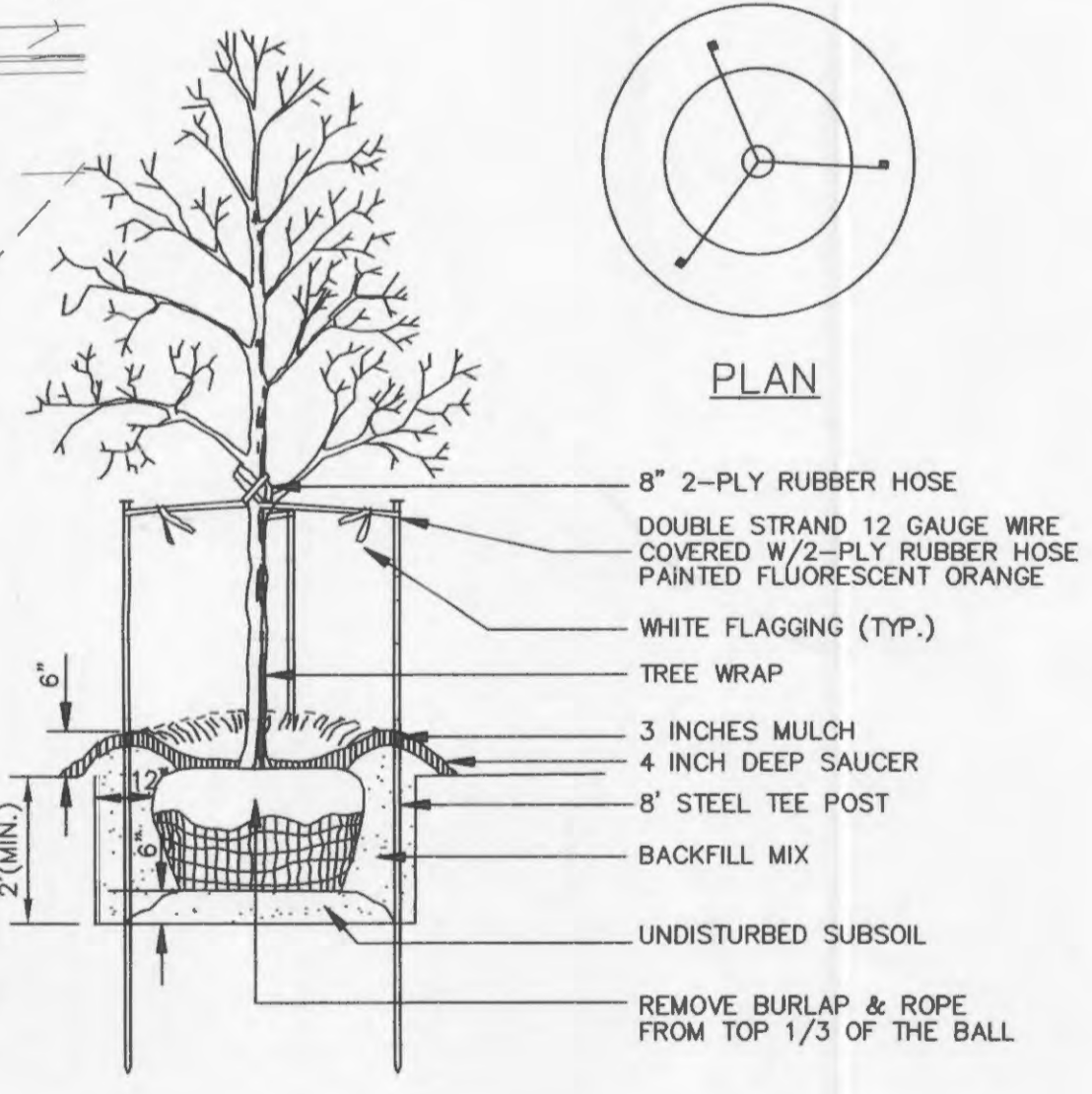
DECIDUOUS TREE PLANTING N.T.S.
