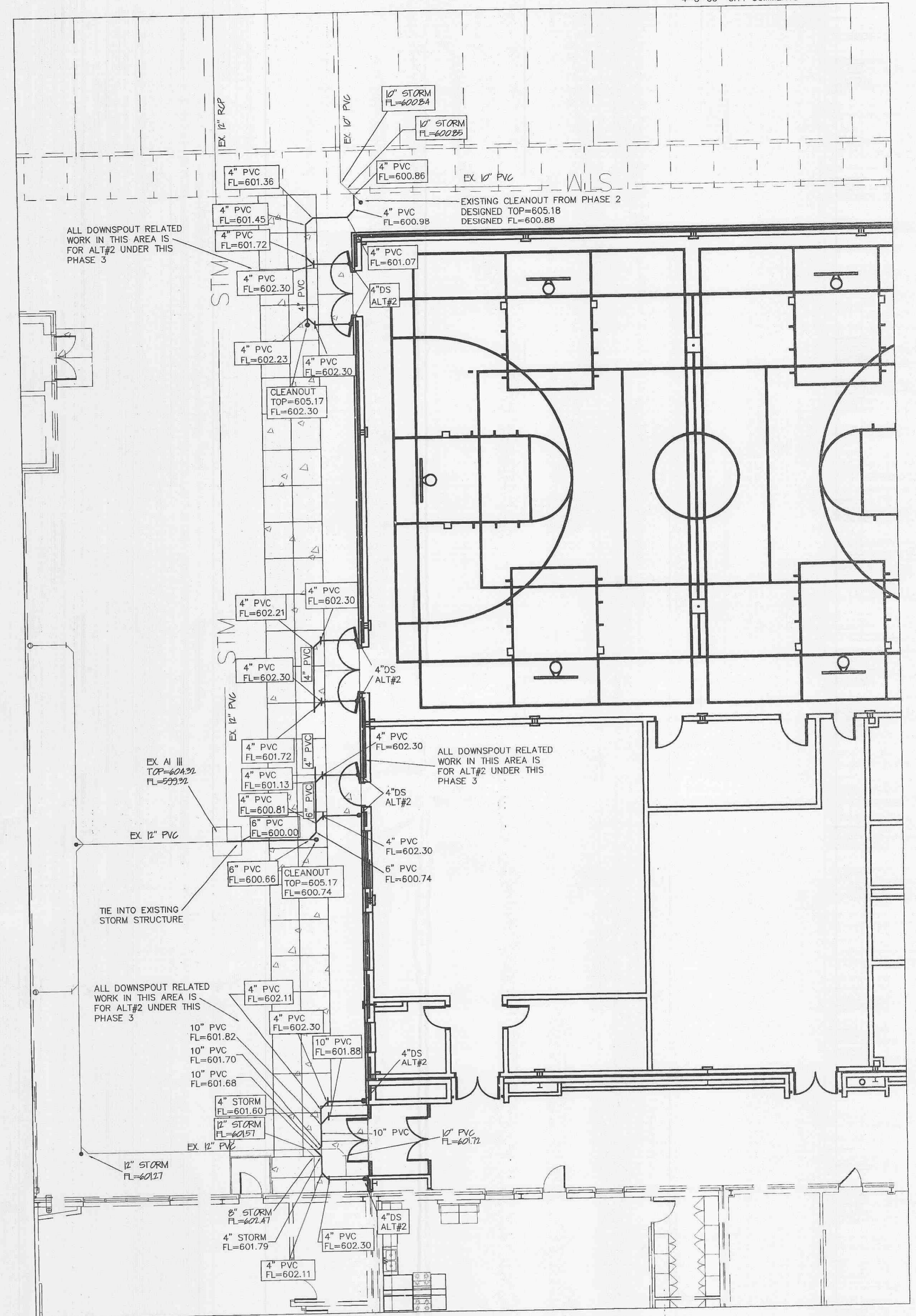
DOWNSPOUT DETAILS NORTHWEST ADDITION ALT#2 SCALE: 1"=10'
