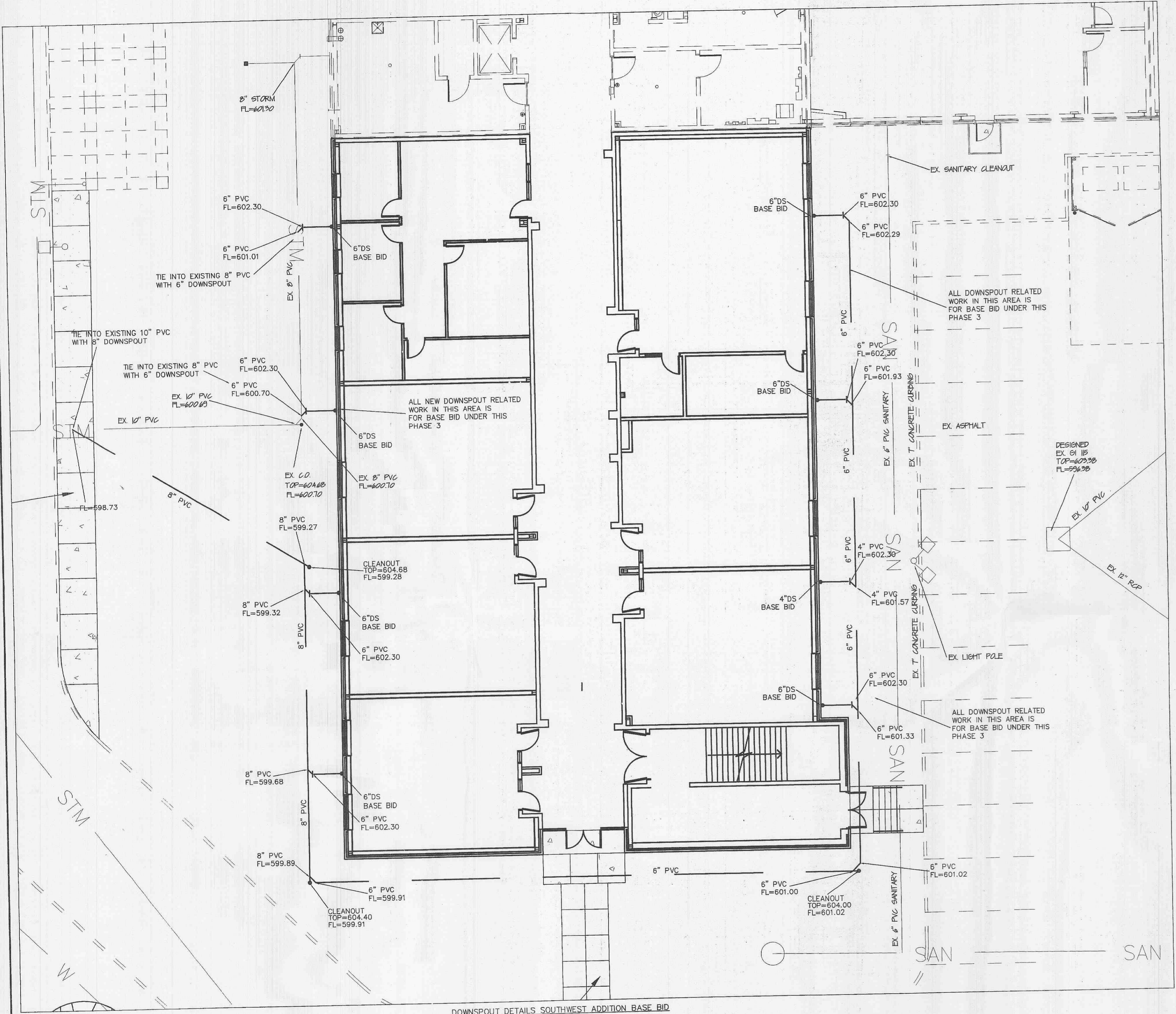
DOWNSPOUT DETAILS SOUTHWEST ADDITION BASE BID SCALE: 1"=10'
