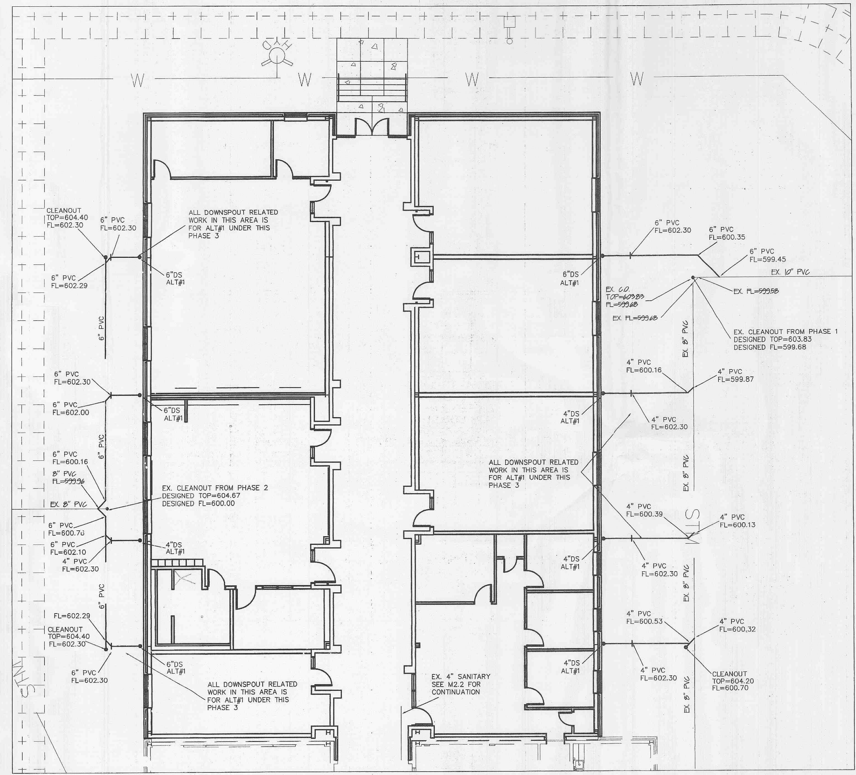
DOWNSPOUT DETAILS NORTHEAST ADDITION ALT#1 SCALE: 1"=10'
