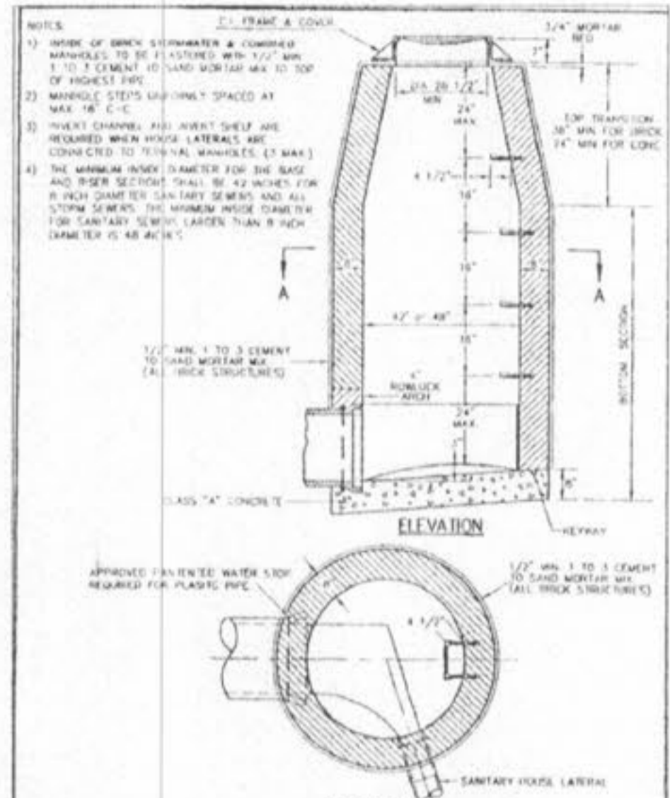
TERMINAL MANHOLE METROPOLITAN ST. LOUIS SEWER DISTRICT Standard Details of Sewer Construction SHEET 20
