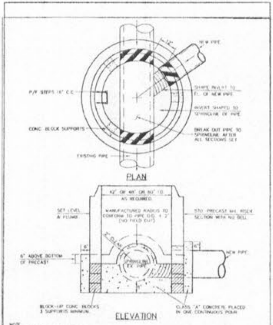
PRECAST MANHOLE ON EXIST. PIPE W/CONTINUOUS FLOW ONLY METROPOLITAN ST. LOUIS SEWER DISTRICT Standard Details of Sewer Construction SHEET 22
