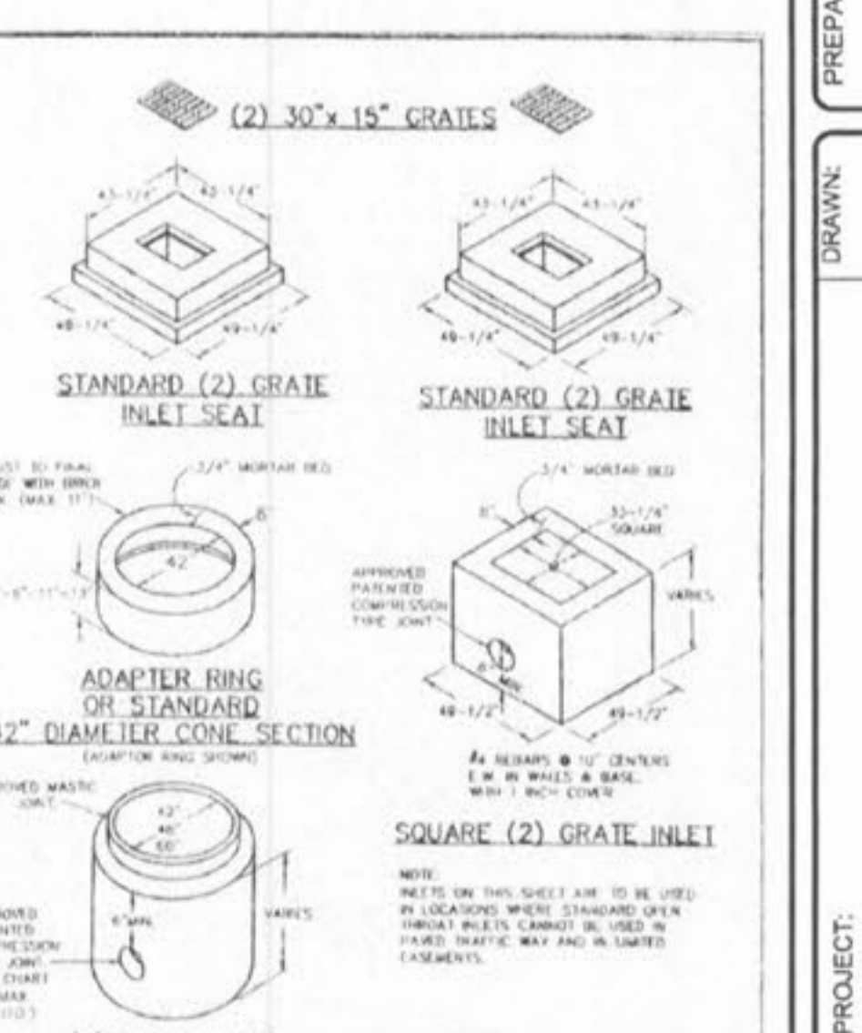
2 GRATE INLETS PRECAST CONCRETE METROPOLITAN ST. LOUIS SEWER DISTRICT Standard Details of Sewer Construction SHEET 36
