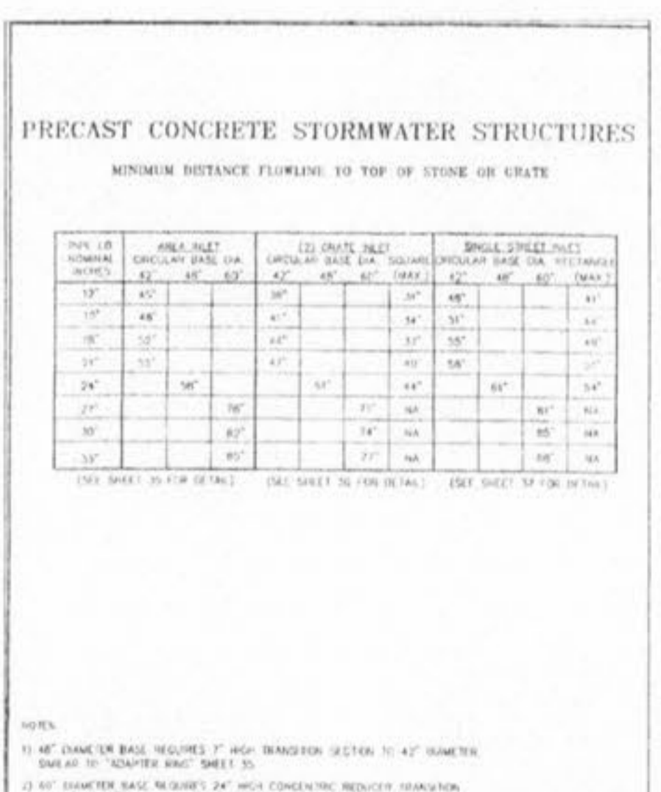
PRECAST CONCRETE STORMWATER STRUCTURES METROPOLITAN ST. LOUIS SEWER DISTRICT Standard Details of Sewer Construction SHEET 34
