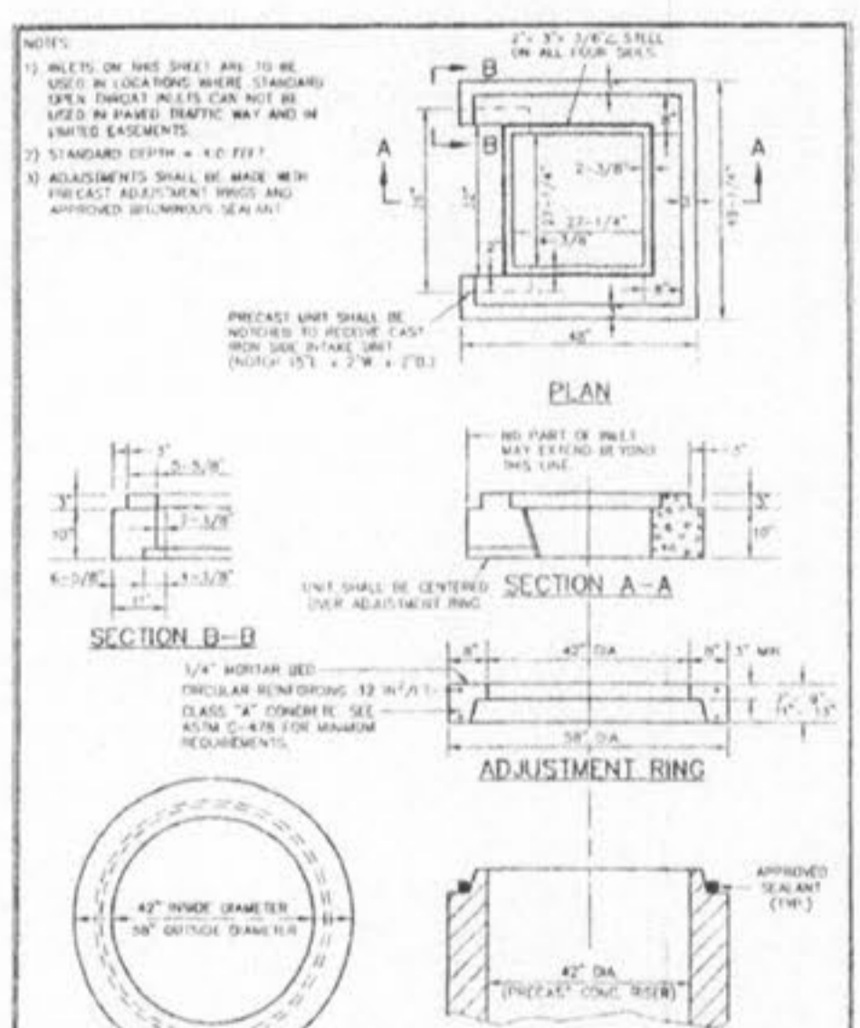
GRATE SEAT FOR 2 GRATE WITH SIDE INTAKE METROPOLITAN ST. LOUIS SEWER DISTRICT Standard Details of Sewer Construction SHEET 33
