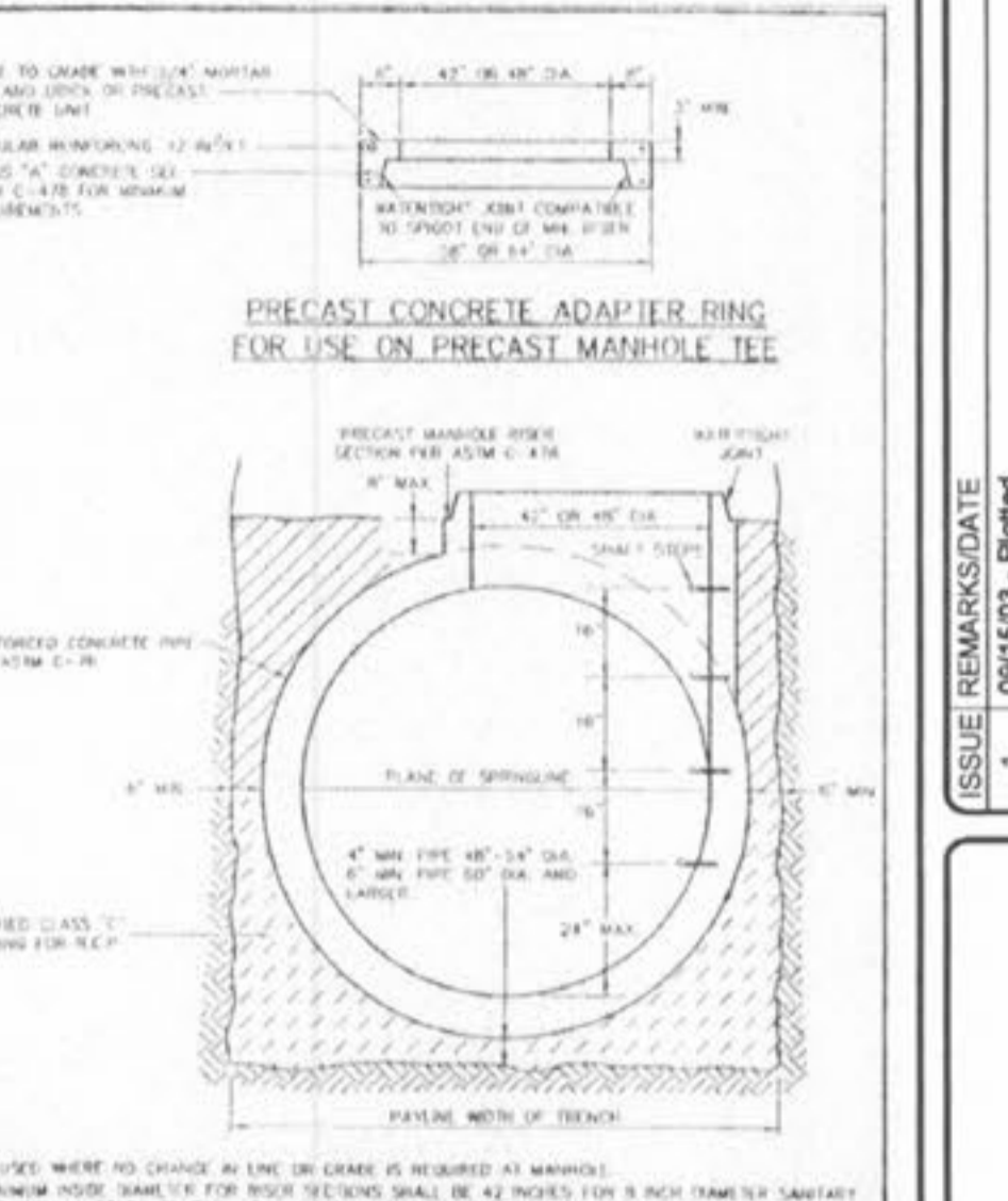
PRECAST CONCRETE ADAPTER RING FOR USE ON PRECAST MANHOLE TEE METROPOLITAN ST. LOUIS SEWER DISTRICT Standard Details of Sewer Construction SHEET 24
