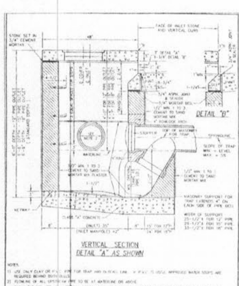
TRAPPED STREET INLET BRICK CONSTRUCTION METROPOLITAN ST. LOUIS SEWER DISTRICT Standard Details of Sewer Construction SHEET 26
