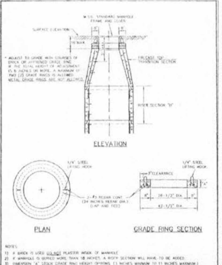
ADJUST TO GRADE METROPOLITAN ST. LOUIS SEWER DISTRICT Standard Details of Sewer Construction SHEET 23
