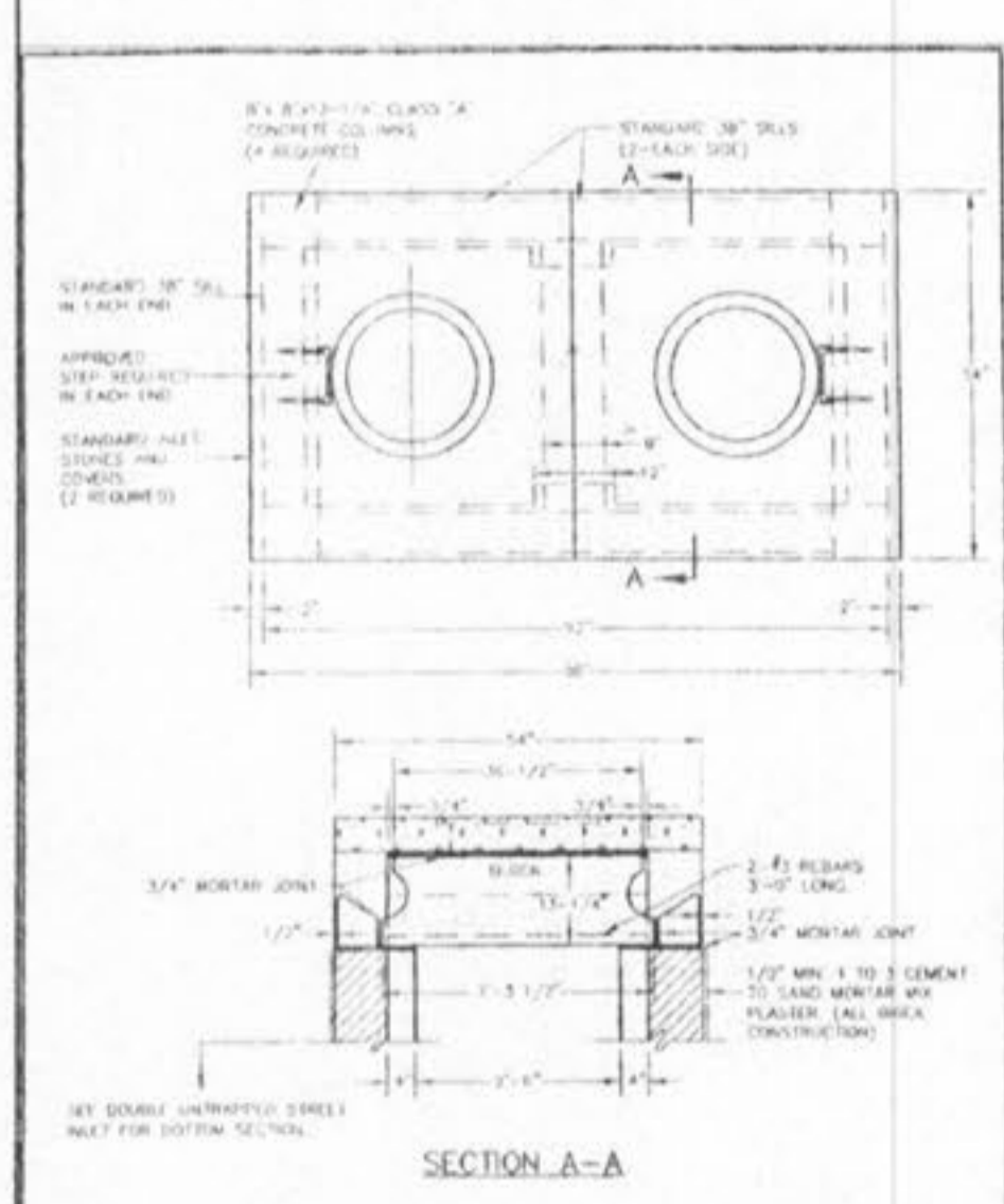
DOUBLE AREA INLET OPEN 4 SIDES BRICK CONSTRUCTION METROPOLITAN ST. LOUIS SEWER DISTRICT Standard Details of Sewer Construction SHEET 31
