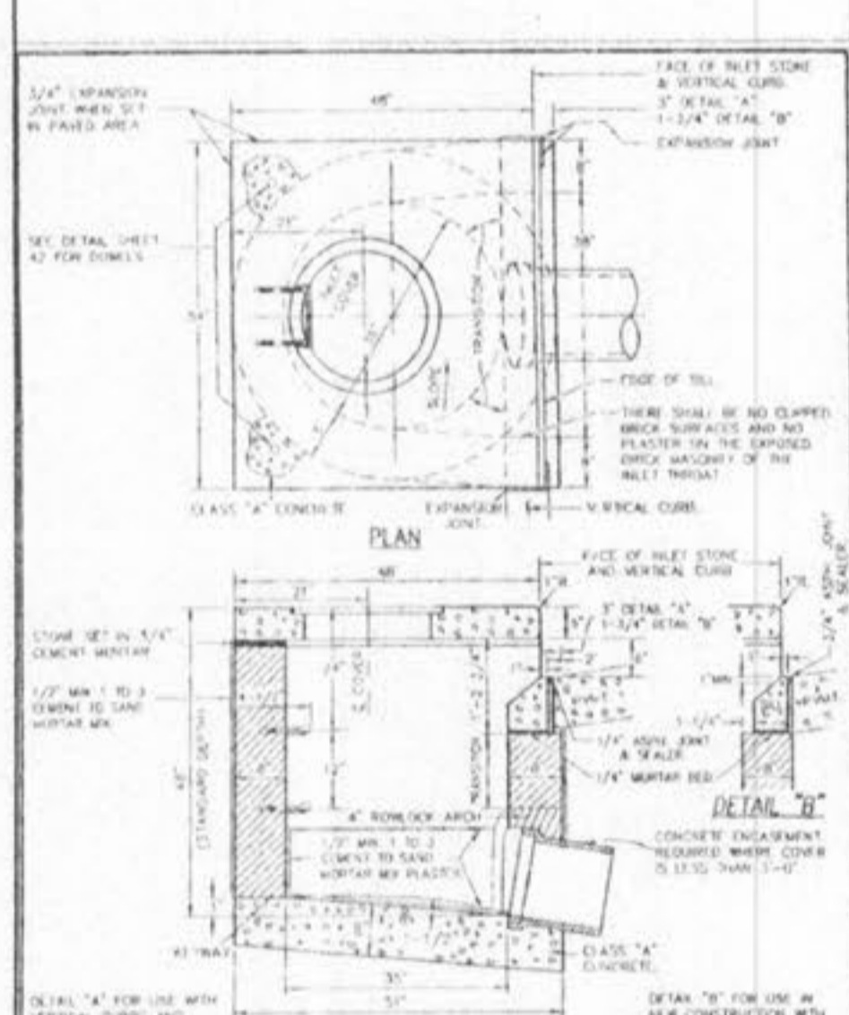
UNTRAPPED STREET INLET BRICK CONSTRUCTION METROPOLITAN ST. LOUIS SEWER DISTRICT Standard Details of Sewer Construction SHEET 25
