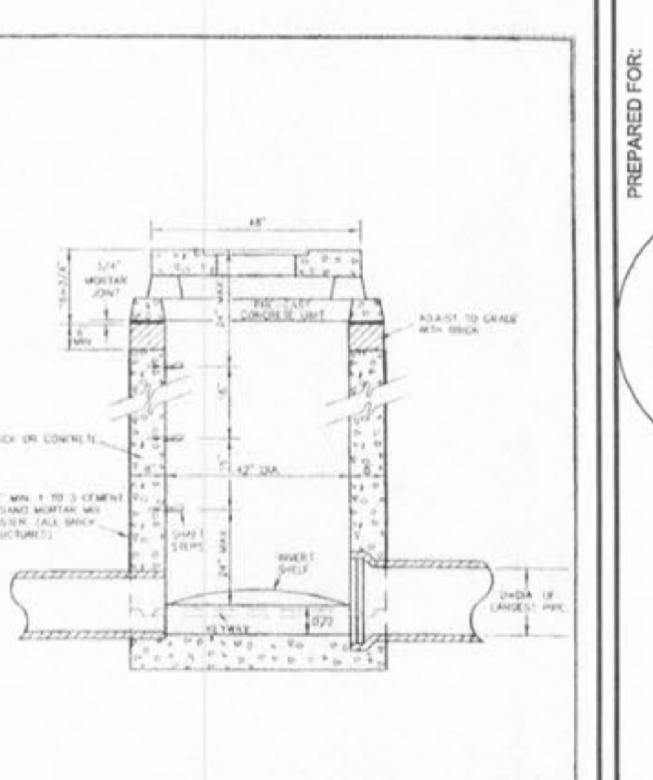
AREA INLET MANHOLE (12" THRU 24") METROPOLITAN ST. LOUIS SEWER DISTRICT Standard Details of Sewer Construction SHEET 30
