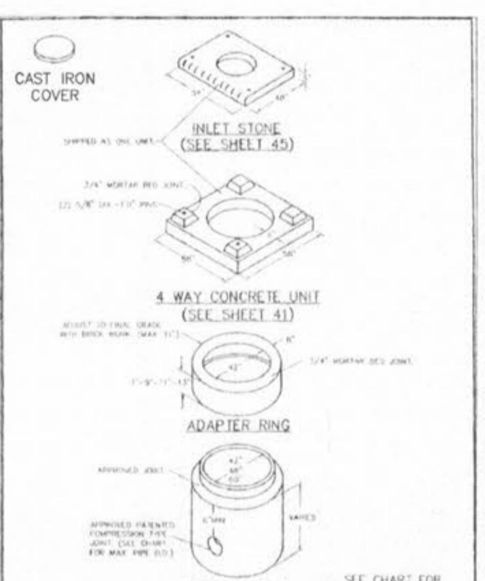
CAST IRON COVER METROPOLITAN ST. LOUIS SEWER DISTRICT Standard Details of Sewer Construction SHEET 35
