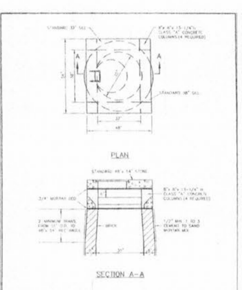
AREA INLET OPEN 4 SIDES BRICK CONSTRUCTION METROPOLITAN ST. LOUIS SEWER DISTRICT Standard Details of Sewer Construction SHEET 29
