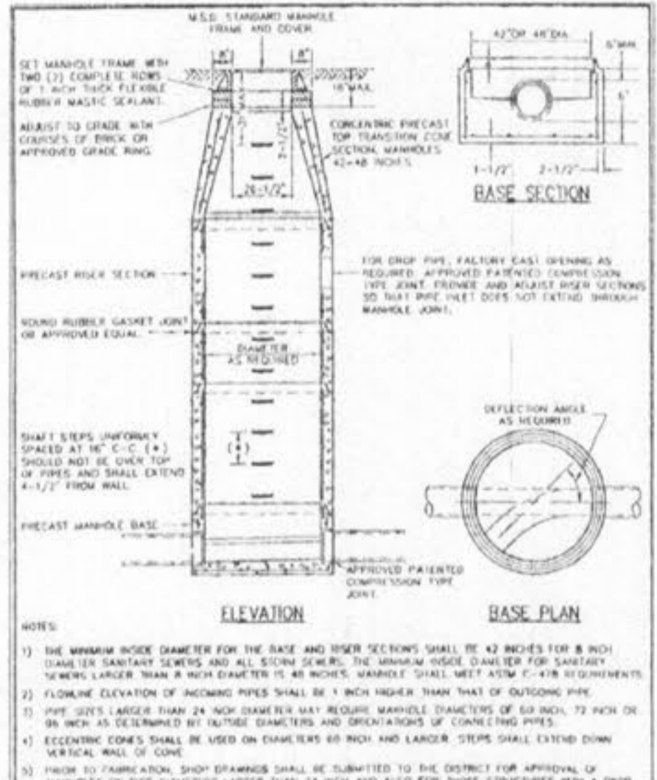
PRECAST CONCRETE MANHOLE METROPOLITAN ST. LOUIS SEWER DISTRICT Standard Details of Sewer Construction SHEET 21
