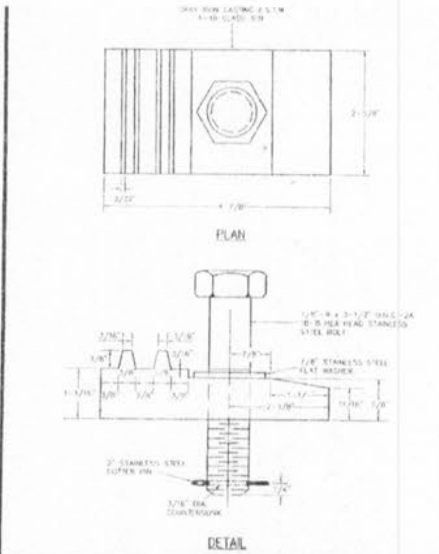
LOCKING DEVICE FOR TYPE "T" LOCK TYPE MANHOLE COVER METROPOLITAN ST. LOUIS SEWER DISTRICT Standard Details of Sewer Construction DR. ROR/SAM CH. J.C.K. 2000 SHEET 55
