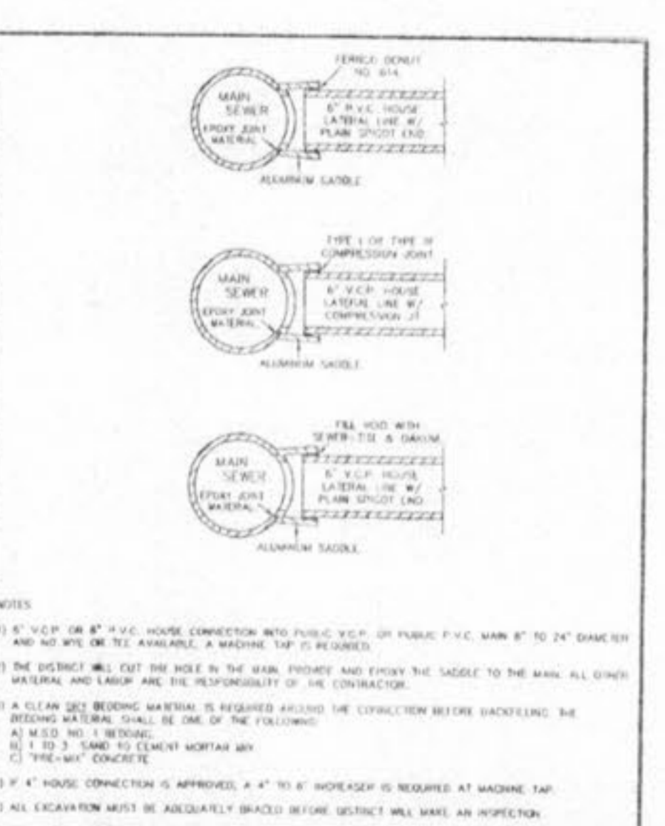
MACHINE TAP METROPOLITAN ST. LOUIS SEWER DISTRICT Standard Details of Sewer Construction DR. W.H./SAM CH. J.C.K. 2000 SHEET 64
