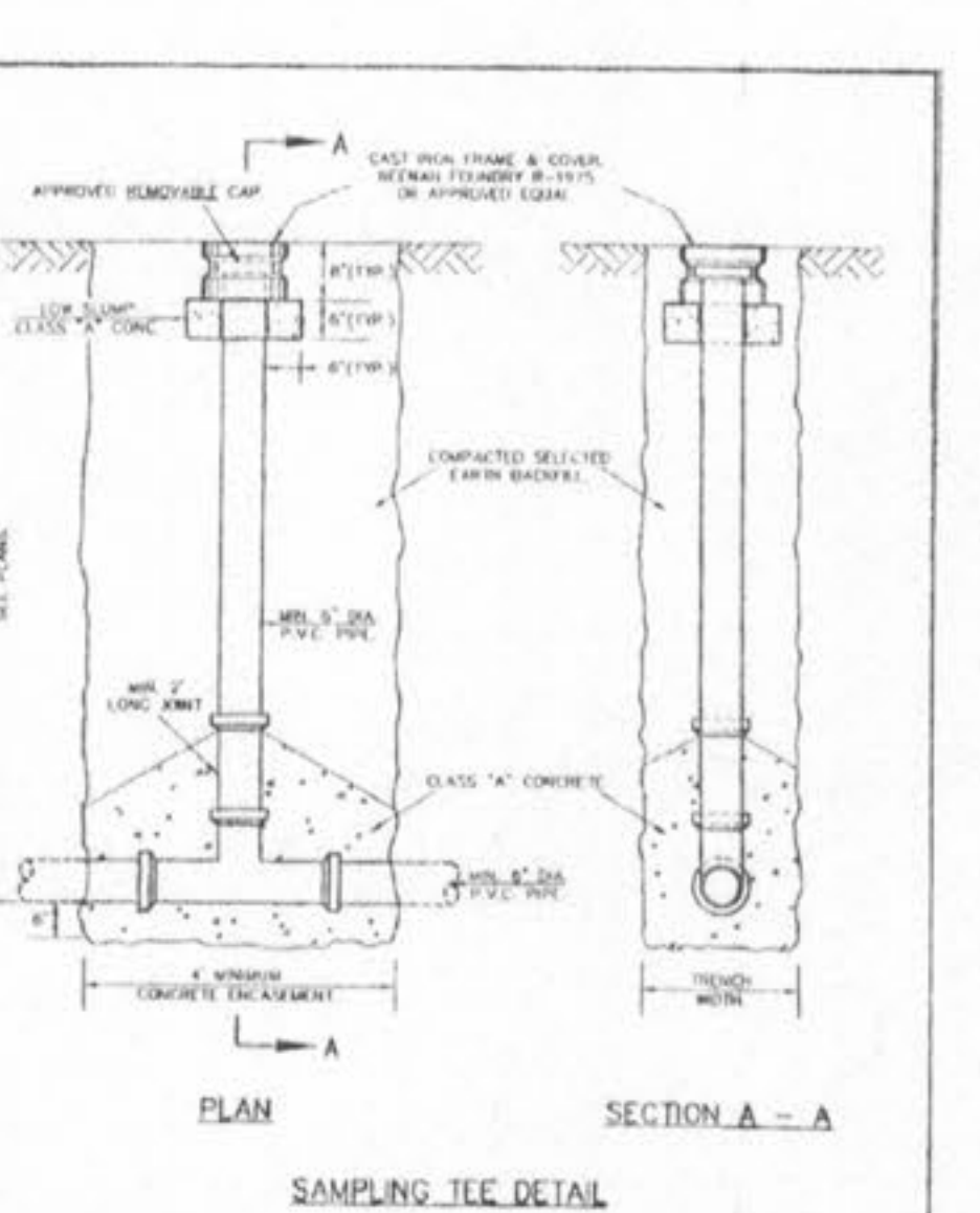
SAMPLING TEE METROPOLITAN ST. LOUIS SEWER DISTRICT Standard Details of Sewer Construction DR. S.A.M. CH. P.W.S. 2000 SHEET 69
