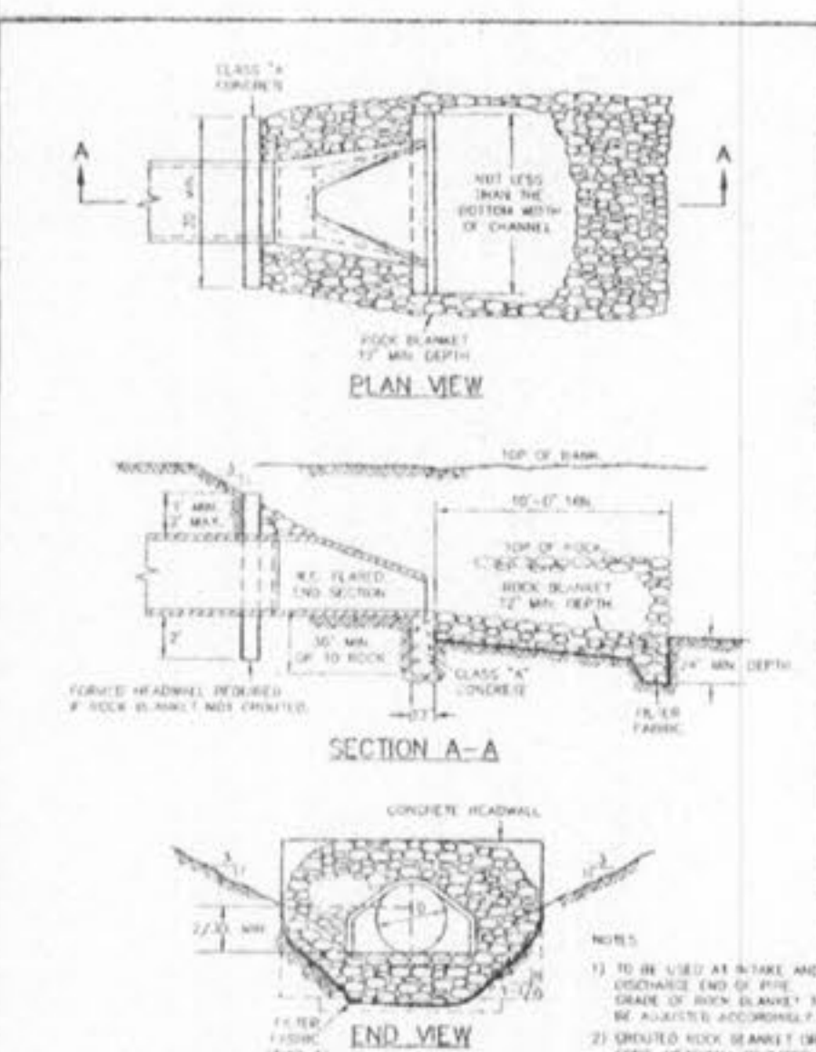
FLARED END SECTION METROPOLITAN ST. LOUIS SEWER DISTRICT Standard Details of Sewer Construction DR. W.H./SAM CH. J.C.K. 2000 SHEET 61
