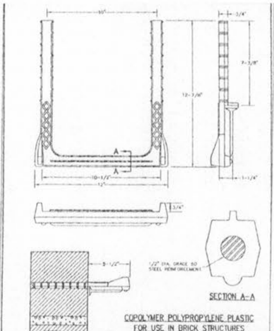
PSI-B MANHOLE STEP INTO JOINT METROPOLITAN ST. LOUIS SEWER DISTRICT Standard Details of Sewer Construction DR. W.S./AM CH. J.C.K. 2000 SHEET 57
