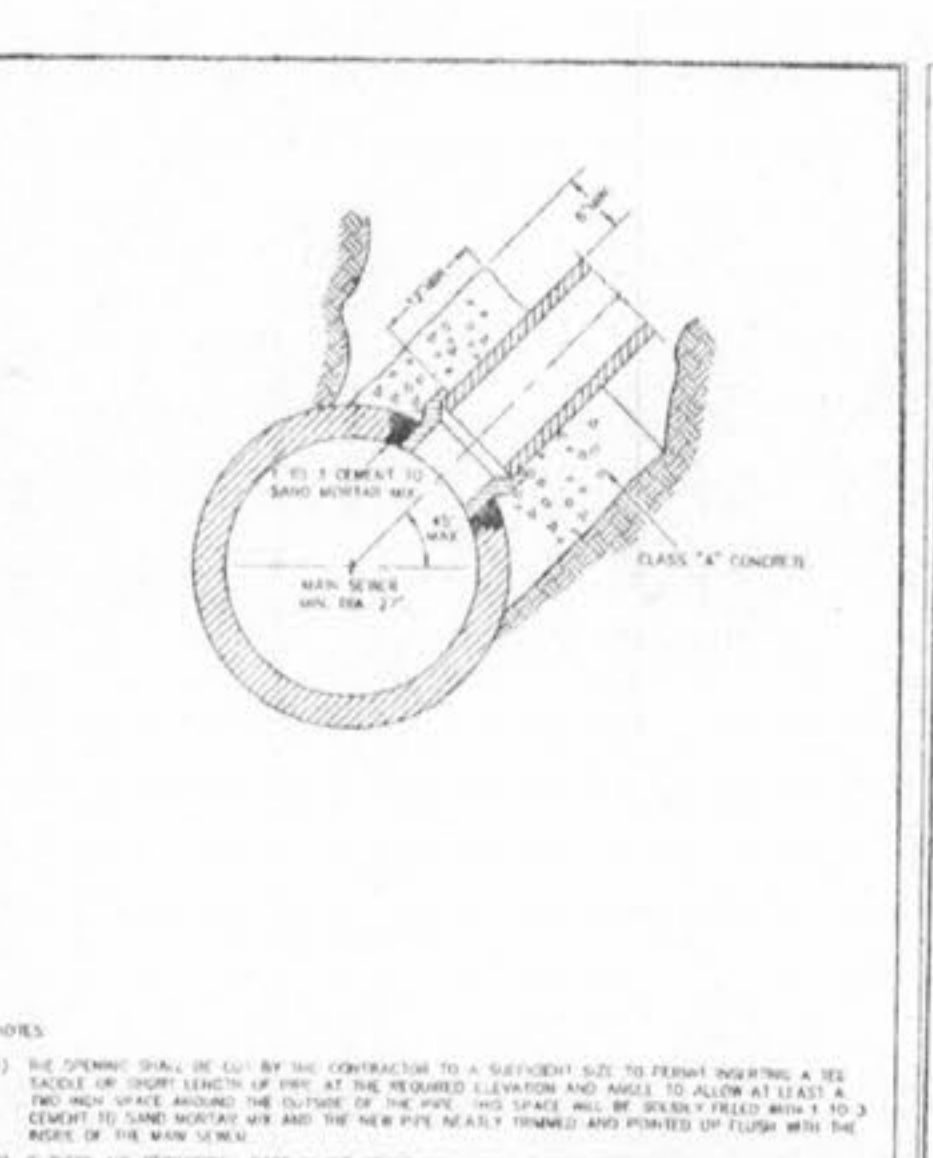
HOUSE CONNECTIONS ALLOWED BY TEE SADDLE METROPOLITAN ST. LOUIS SEWER DISTRICT Standard Details of Sewer Construction DR. D.A.B./SAM CH. J.C.K. 2000 SHEET 65
