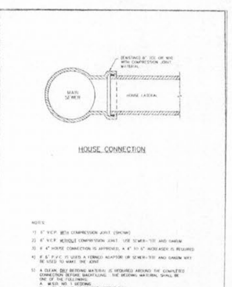
HOUSE CONNECTION TO EXISTING TEE OR WYE METROPOLITAN ST. LOUIS SEWER DISTRICT Standard Details of Sewer Construction DR. L.A.B./SAM CH. J.C.K. 2000 SHEET 63
