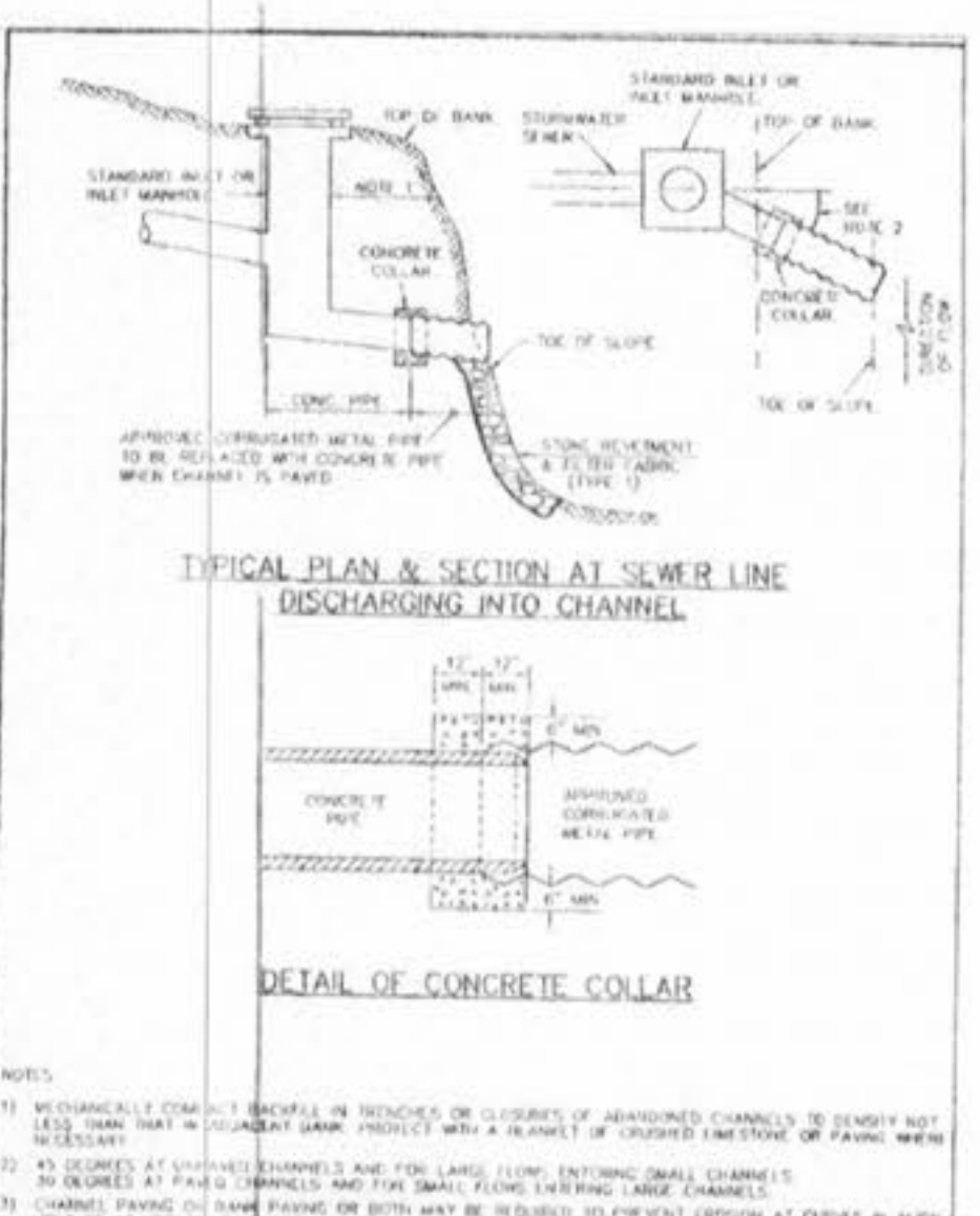
TYPICAL PLAN & SECTION AT SEWER LINE DISCHARGING INTO CHANNEL METROPOLITAN ST. LOUIS SEWER DISTRICT Standard Details of Sewer Construction DR. ROR/SAM CH. J.C.K. 2000 SHEET 62
