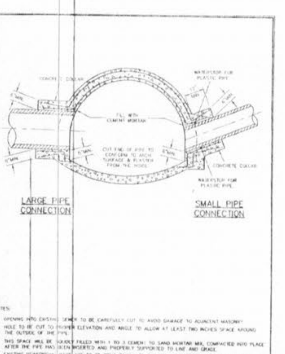
CONNECTIONS TO LARGE SEWERS METROPOLITAN ST. LOUIS SEWER DISTRICT Standard Details of Sewer Construction DR. W.H./SAM CH. J.C.K. 2000 SHEET 68
