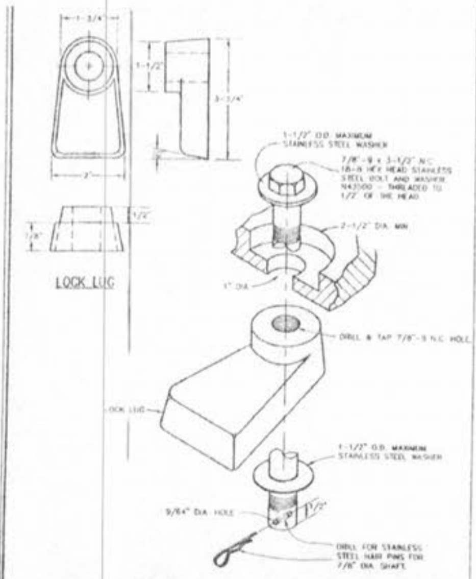
LOCKING DEVICE FOR TYPE "T" LOCK TYPE MANHOLE COVER METROPOLITAN ST. LOUIS SEWER DISTRICT Standard Details of Sewer Construction DR. J.D./SAM CH. J.C.K. 2000 SHEET 56
