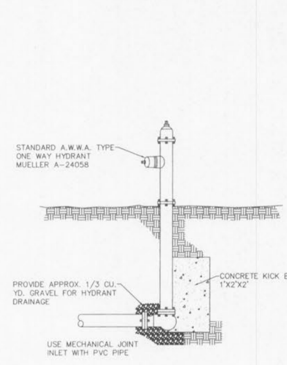
FLUSHING HYDRANT NOT TO SCALE
