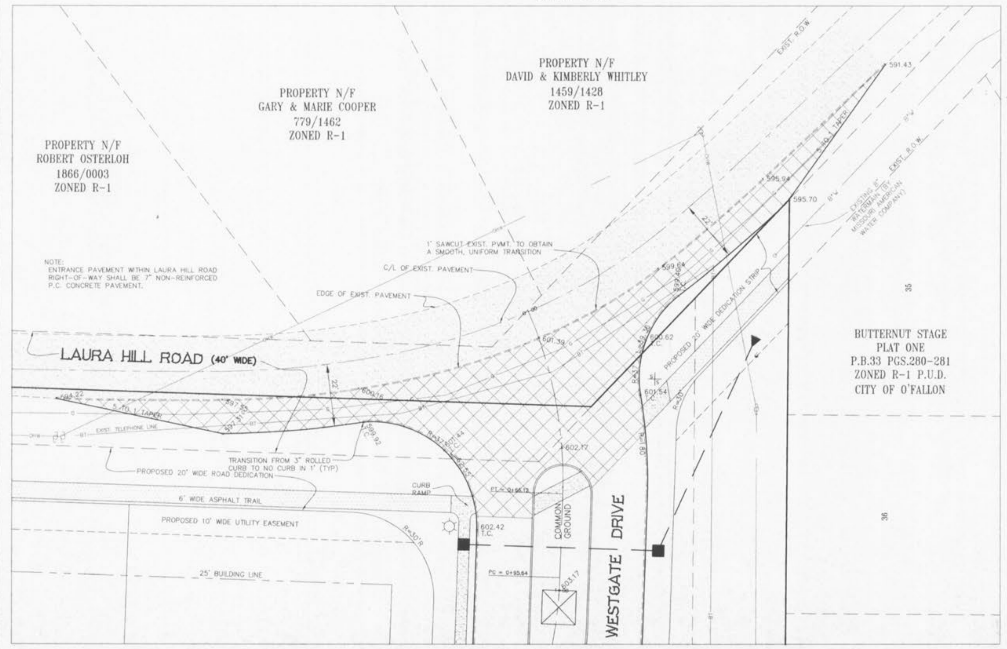
ENTRANCE DETAIL SCALE: 1" = 20'
