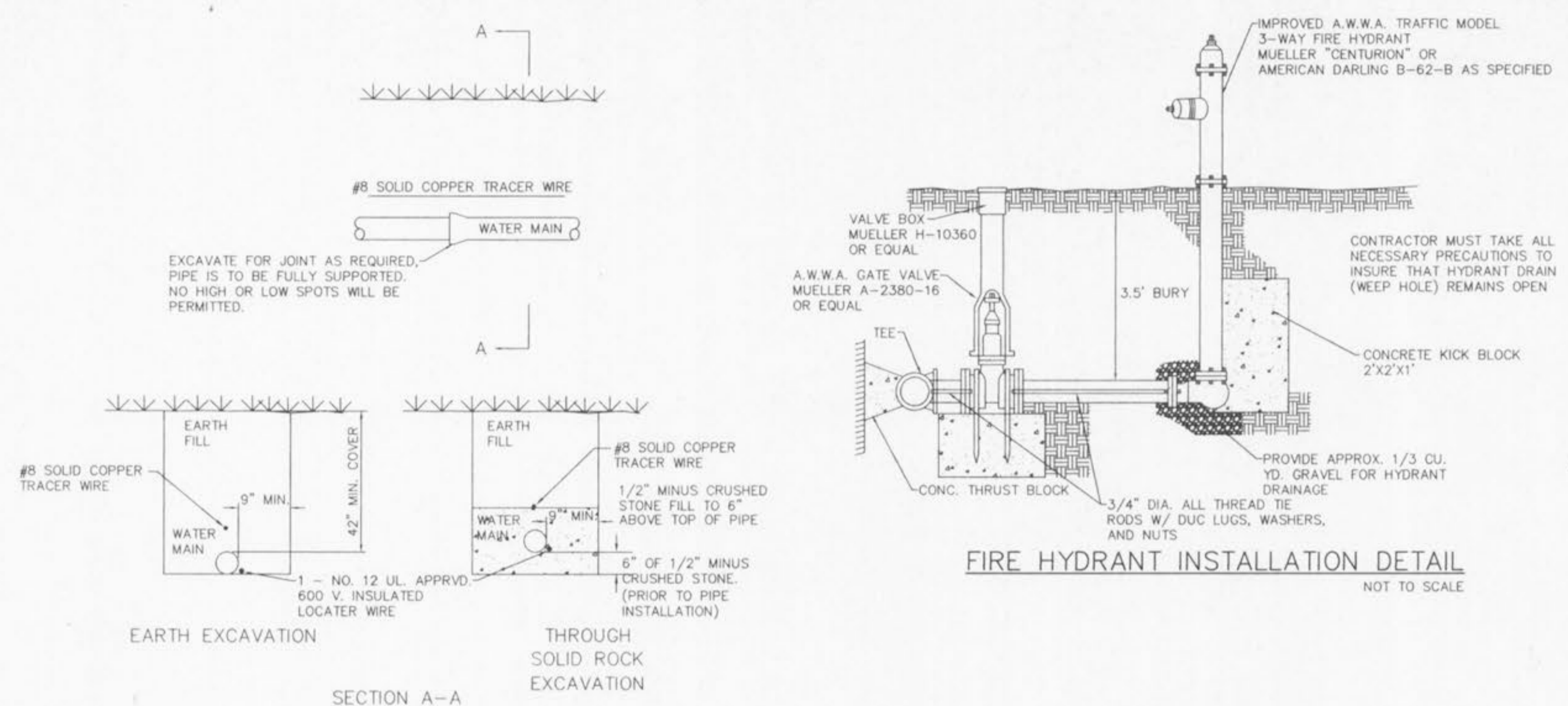
TYPICAL WATER MAIN INSTALLATION DETAILS NOT TO SCALE
