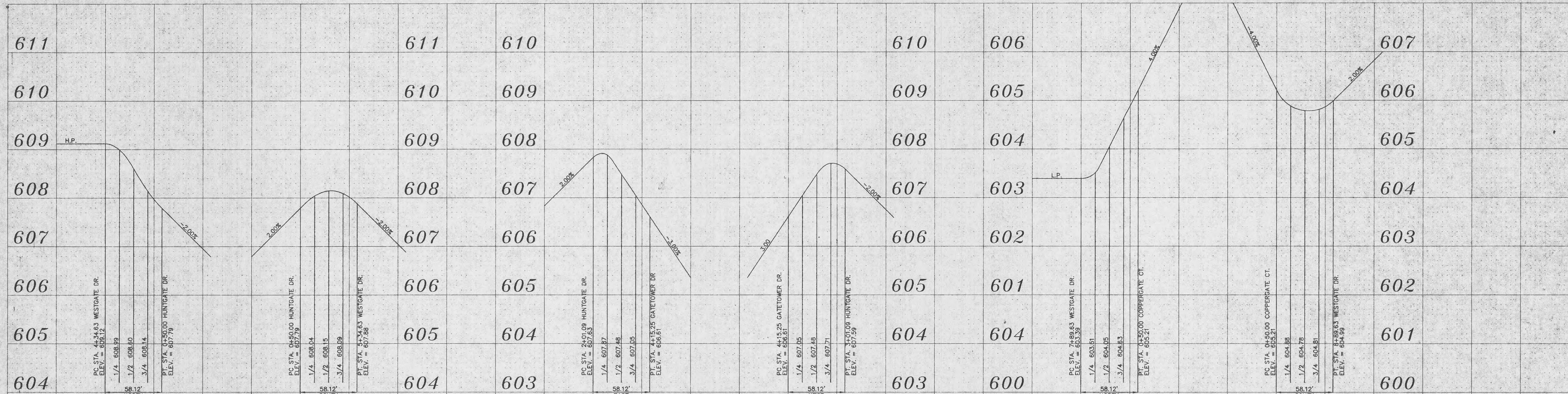
WESTGATE DRIVE & HUNTCATE DRIVE TOP OF CURB ELEVATION
