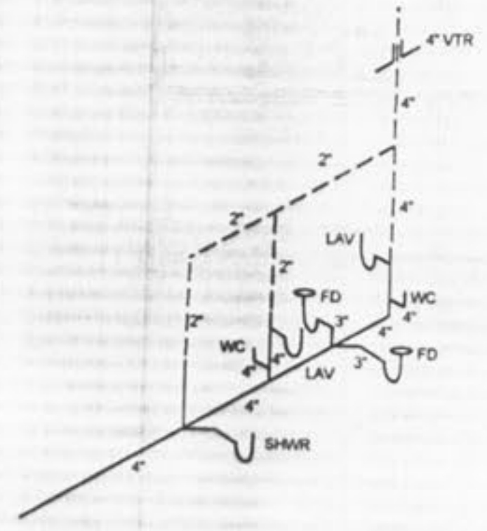
Waste & Vent Riser Diagram No Scale
