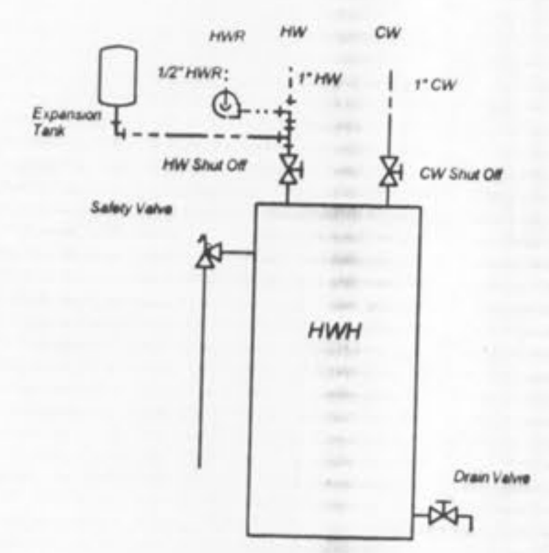
Hot Water Heater Piping Diagram No Scale
