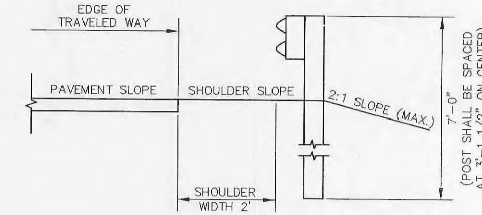
GUARDRAIL DETAIL NOT TO SCALE
