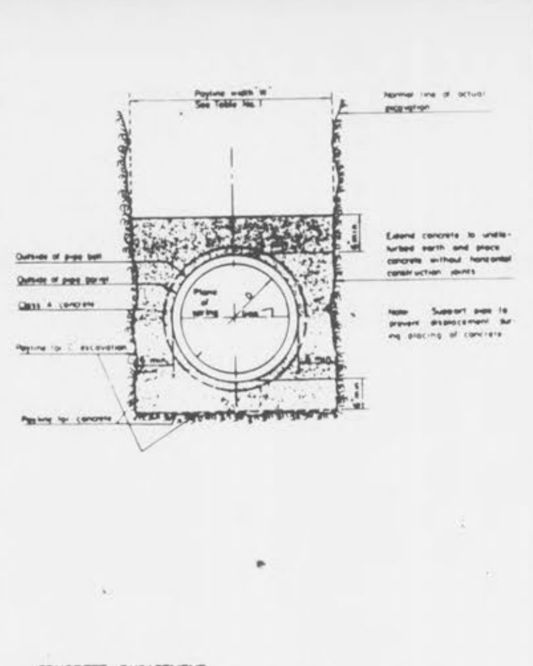
CONCRETE ENCASUREMENT
