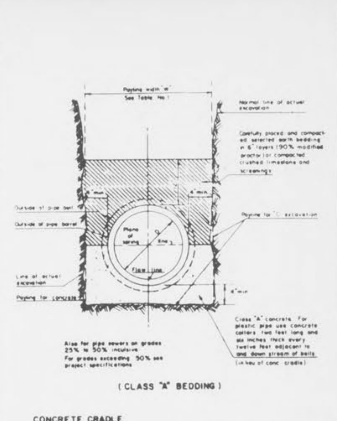
CONCRETE CRADLE
