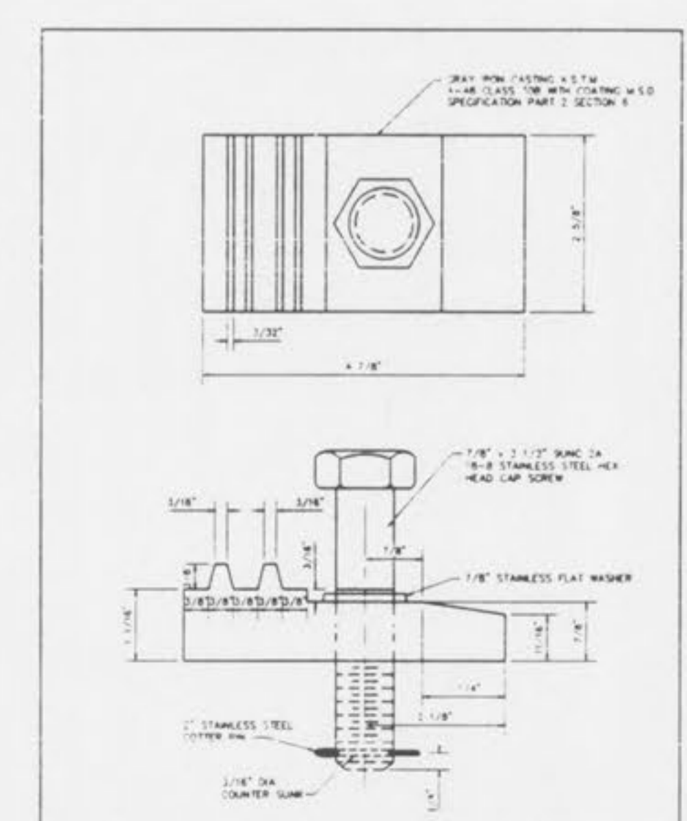
LOCKING DEVICE FOR TYPE 'T' LOCK TYPE MANHOLE COVER METROPOLITAN ST. LOUIS SEWER DISTRICT Standard Details of Sewer Construction
