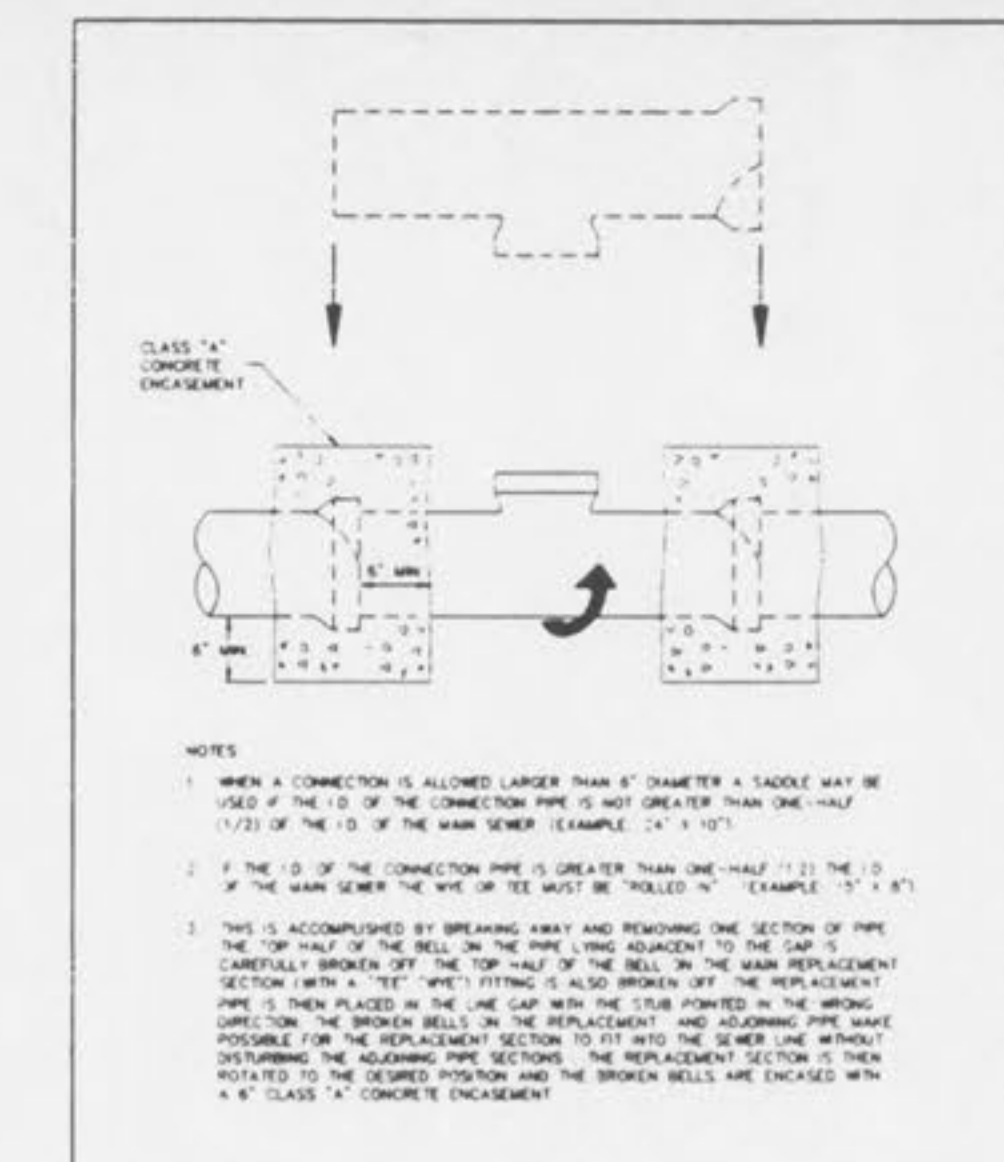
'ROLL-IN' (FOR EXISTING CLAY OR CONCRETE PIPE) METROPOLITAN ST. LOUIS SEWER DISTRICT Standard Details of Sewer Construction
