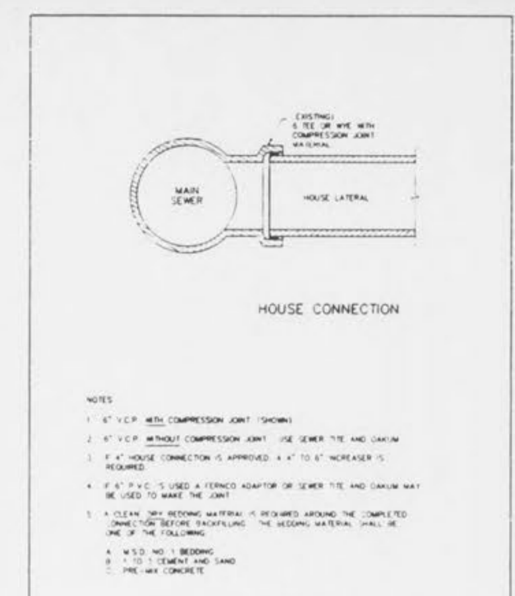
HOUSE CONNECTION TO EXISTING TEE OR WYE METROPOLITAN ST. LOUIS SEWER DISTRICT Standard Details of Sewer Construction
