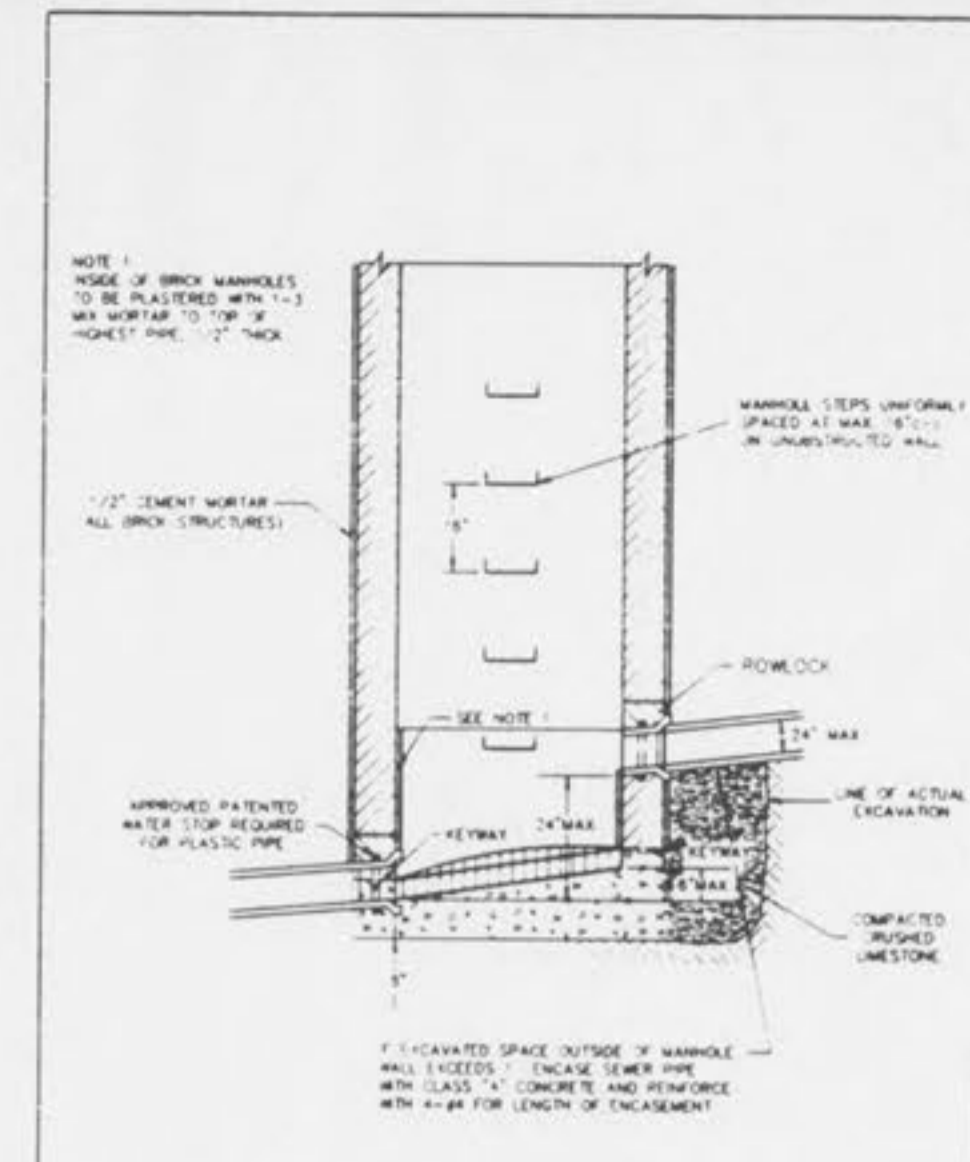
INSIDE FOULWATER DROP MANHOLE (FOR FREE-FALL) METROPOLITAN ST. LOUIS SEWER DISTRICT Standard Details of Sewer Construction
