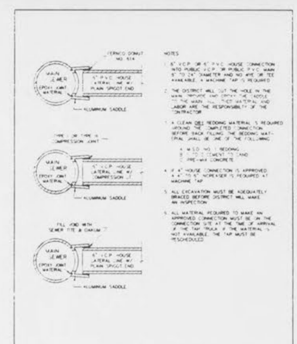
MACHINE TAP METROPOLITAN ST. LOUIS SEWER DISTRICT Standard Details of Sewer Construction
