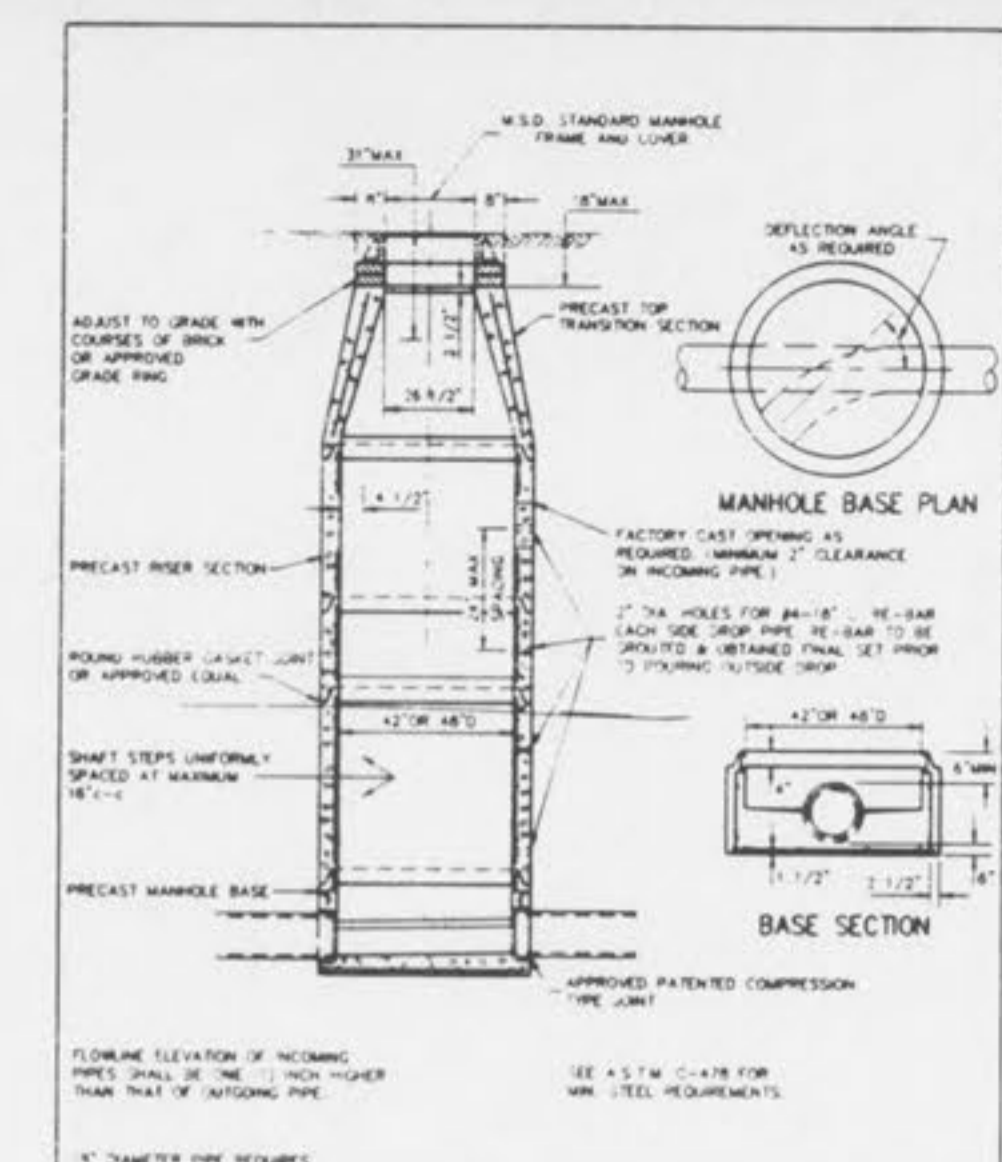
PRE-CAST CONCRETE MANHOLE FOR SEWERS 8" THROUGH 18" METROPOLITAN ST. LOUIS SEWER DISTRICT Standard Details of Sewer Construction
