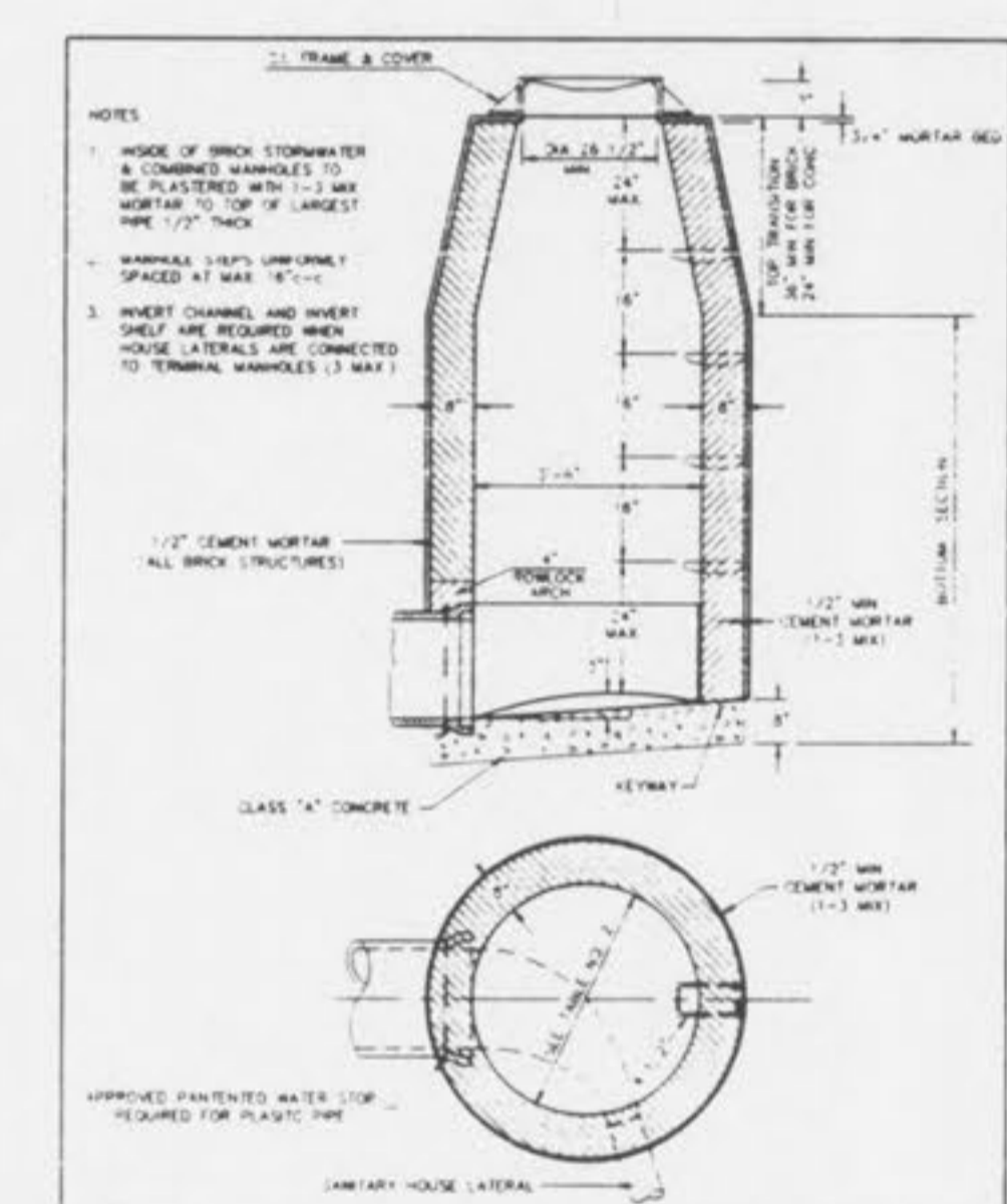
TERMINAL MANHOLE METROPOLITAN ST. LOUIS SEWER DISTRICT Standard Details of Sewer Construction
