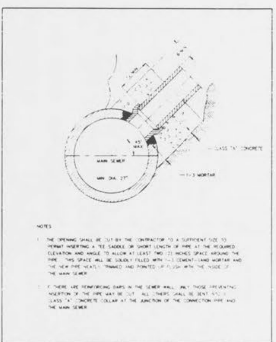
HOUSE CONNECTIONS ALLOWED BY TEE SADDLE METROPOLITAN ST. LOUIS SEWER DISTRICT Standard Details of Sewer Construction
