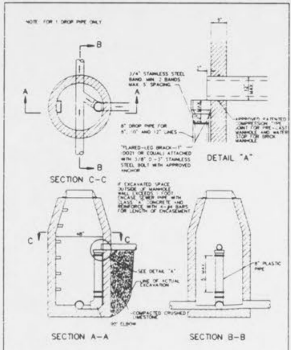
INSIDE FOULWATER DROP MANHOLE METROPOLITAN ST. LOUIS SEWER DISTRICT Standard Details of Sewer Construction
