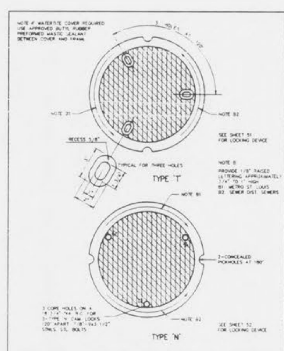
CAST IRON MANHOLE COVERS (LOCK TYPE) METROPOLITAN ST. LOUIS SEWER DISTRICT Standard Details of Sewer Construction
