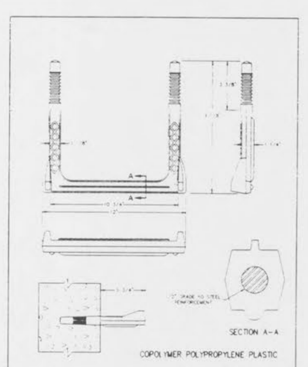
MANHOLE STEP FOR PRECAST MANHOLE METROPOLITAN ST. LOUIS SEWER DISTRICT Standard Details of Sewer Construction
