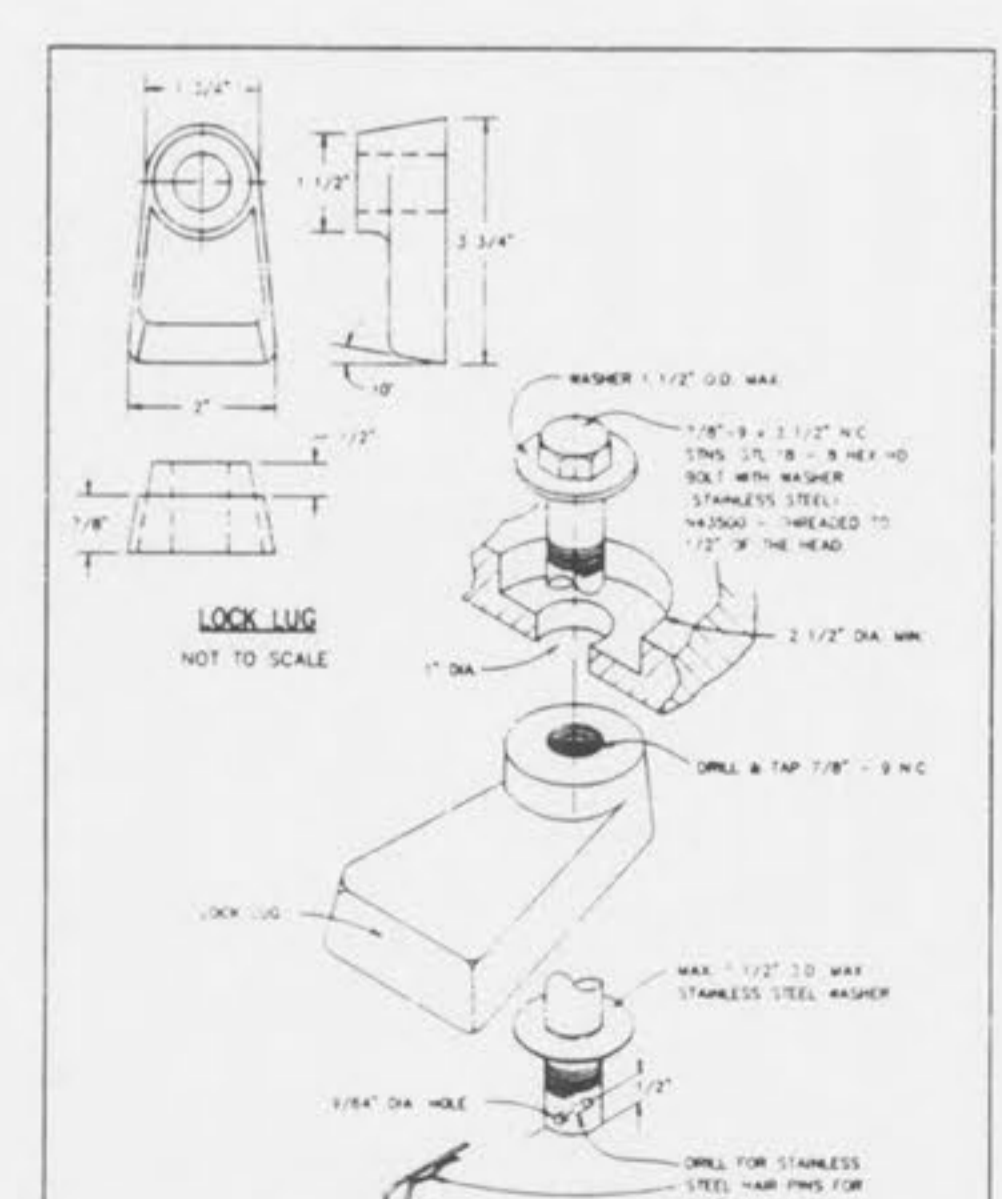
LOCKING DEVICE FOR TYPE 'N' LOCK TYPE MANHOLE COVER METROPOLITAN ST. LOUIS SEWER DISTRICT Standard Details of Sewer Construction
