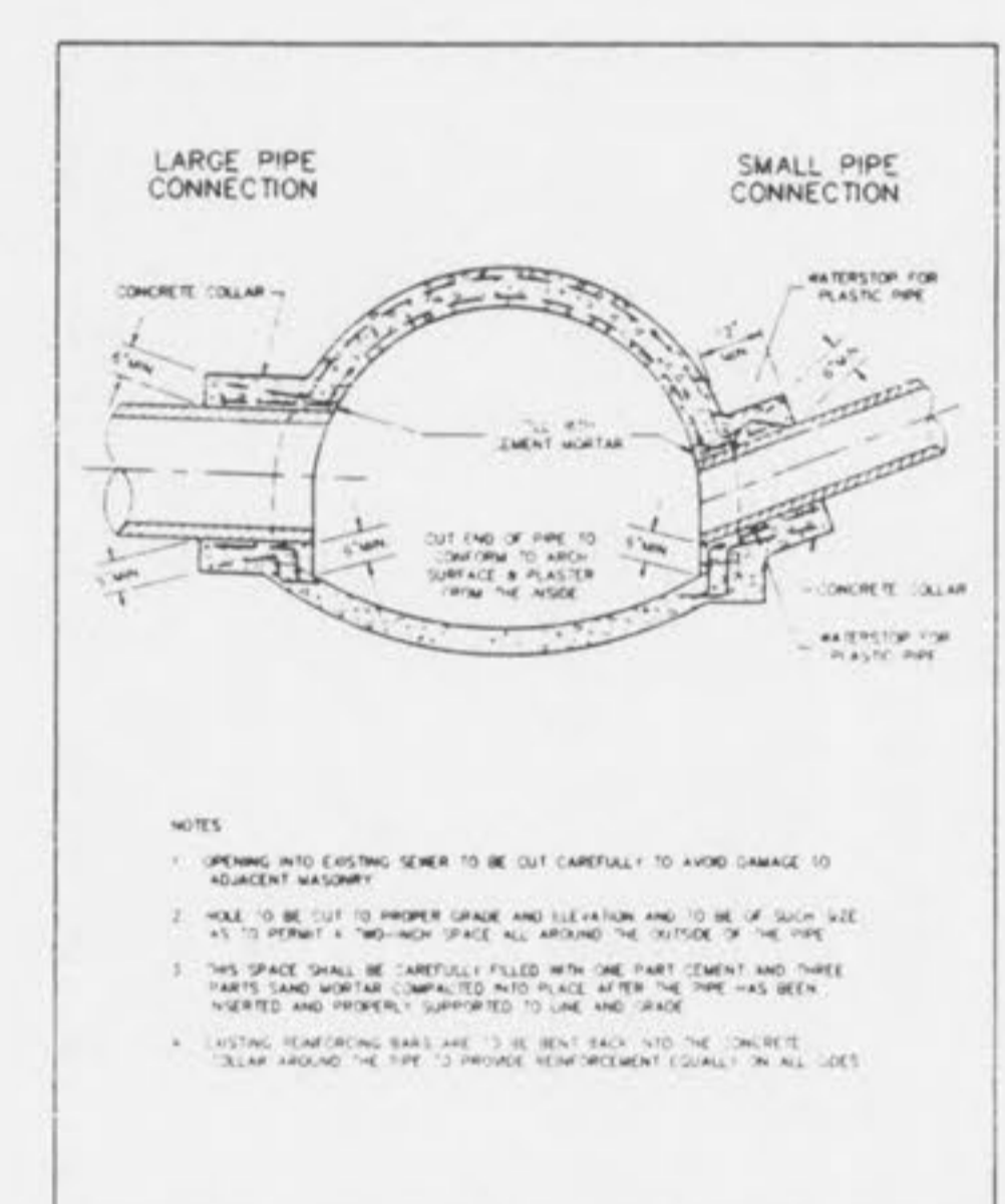
CONNECTIONS TO LARGE SEWERS METROPOLITAN ST. LOUIS SEWER DISTRICT Standard Details of Sewer Construction
