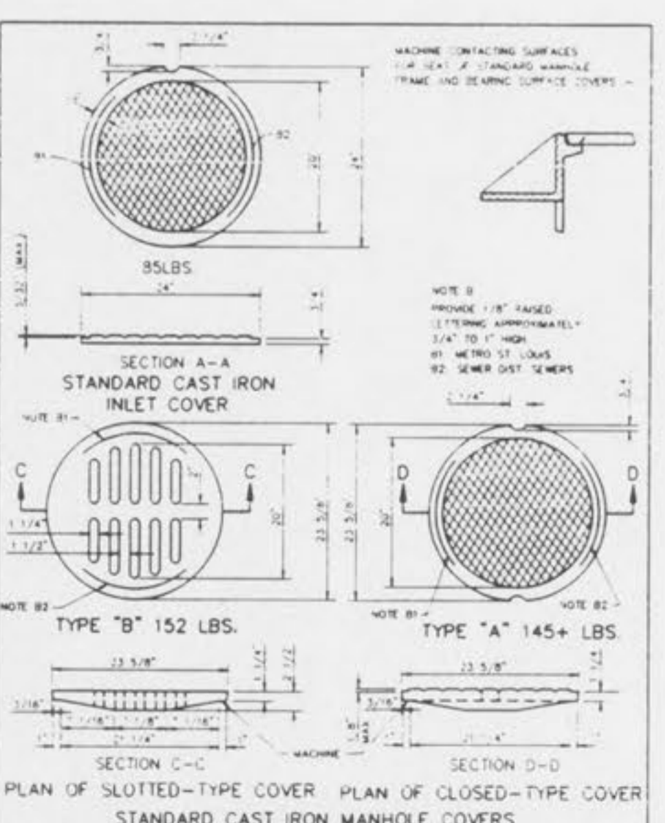
CAST IRON COVERS MANHOLES AND INLETS METROPOLITAN ST. LOUIS SEWER DISTRICT Standard Details of Sewer Construction
