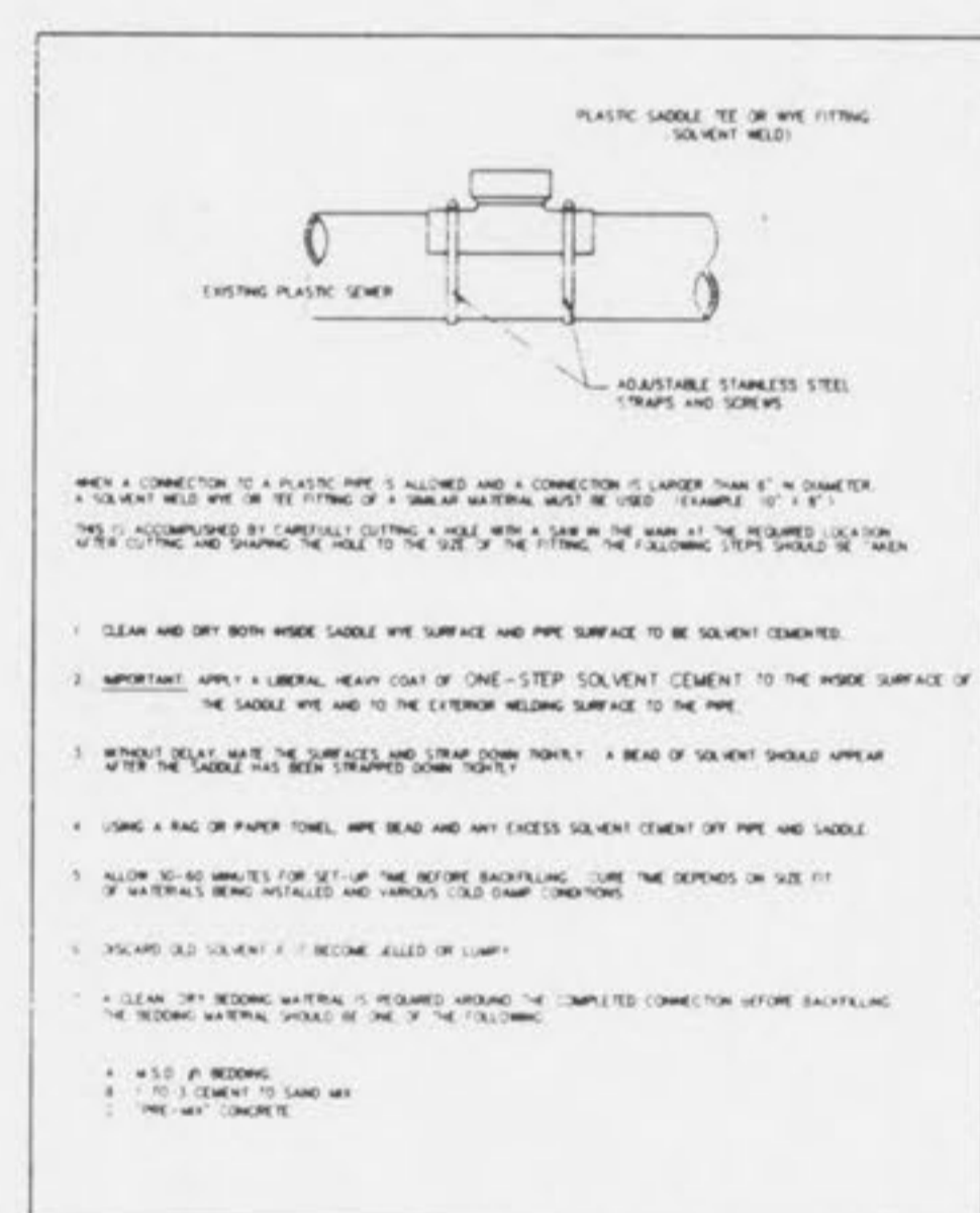
8" (& LARGER) CONNECTION TO PLASTIC MAIN METROPOLITAN ST. LOUIS SEWER DISTRICT Standard Details of Sewer Construction
