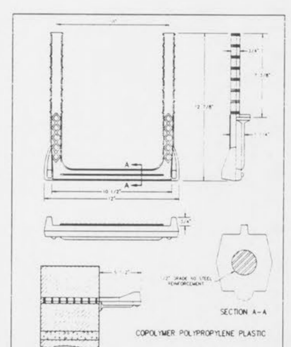
PSI-B MANHOLE STEP INTO JOINT METROPOLITAN ST. LOUIS SEWER DISTRICT Standard Details of Sewer Construction
