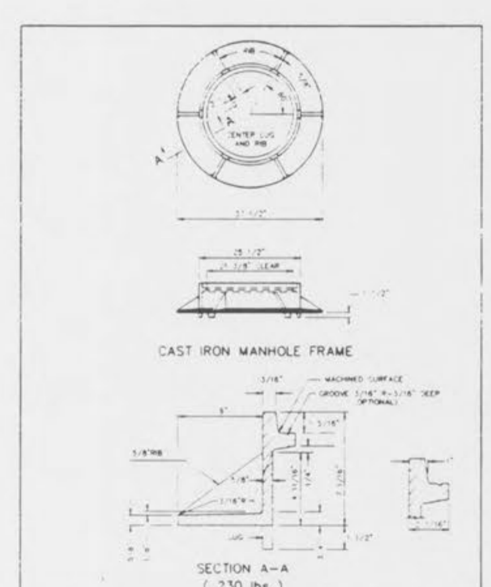
CAST IRON MANHOLE FRAME METROPOLITAN ST. LOUIS SEWER DISTRICT Standard Details of Sewer Construction
