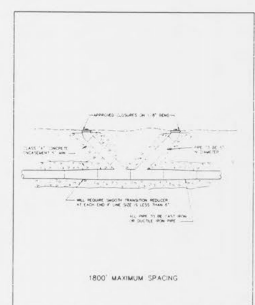
FORCE MAIN CLEANOUT (6" DIA & SMALLER) METROPOLITAN ST. LOUIS SEWER DISTRICT Standard Details of Sewer Construction
