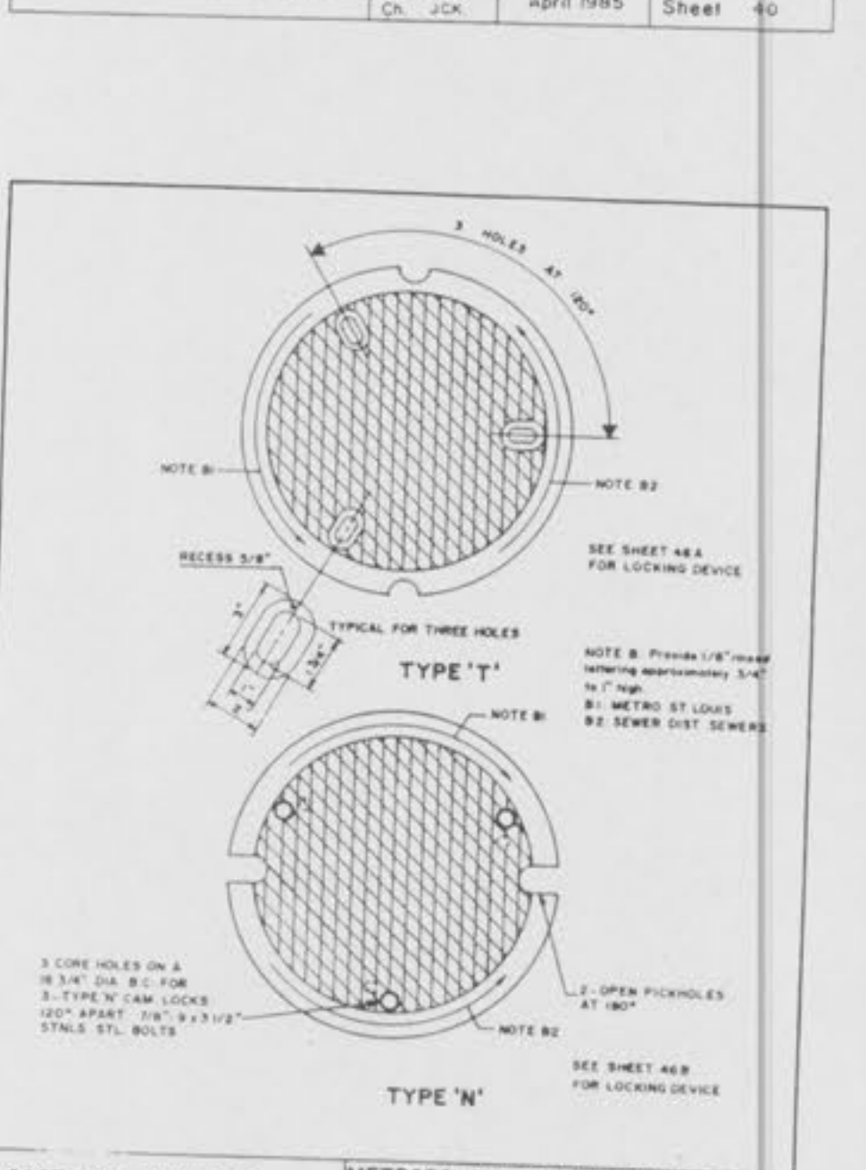
DETAILS OF INLET FRAME AND GRATES METROPOLITAN ST LOUIS SEWER DISTRICT Standard Details of Sewer Construction Dr. R.P.P. April 1985 Sheet 40
