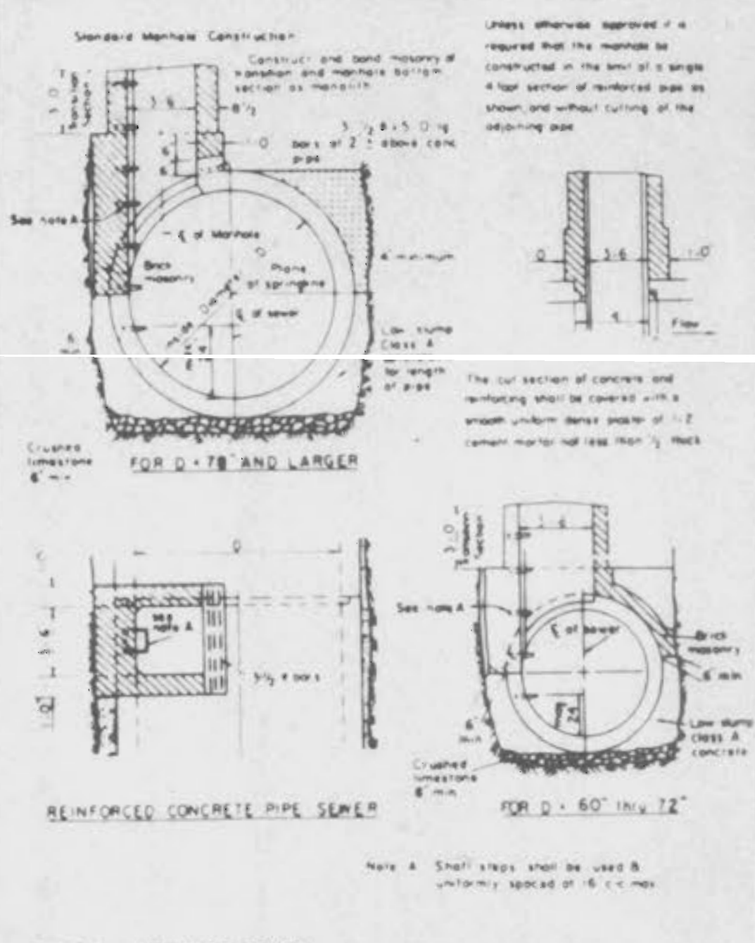
PRE-CAST CONCRETE MANHOLE FOR SEWERS 6" THROUGH 12" IN DIAMETER DETAIL 12
