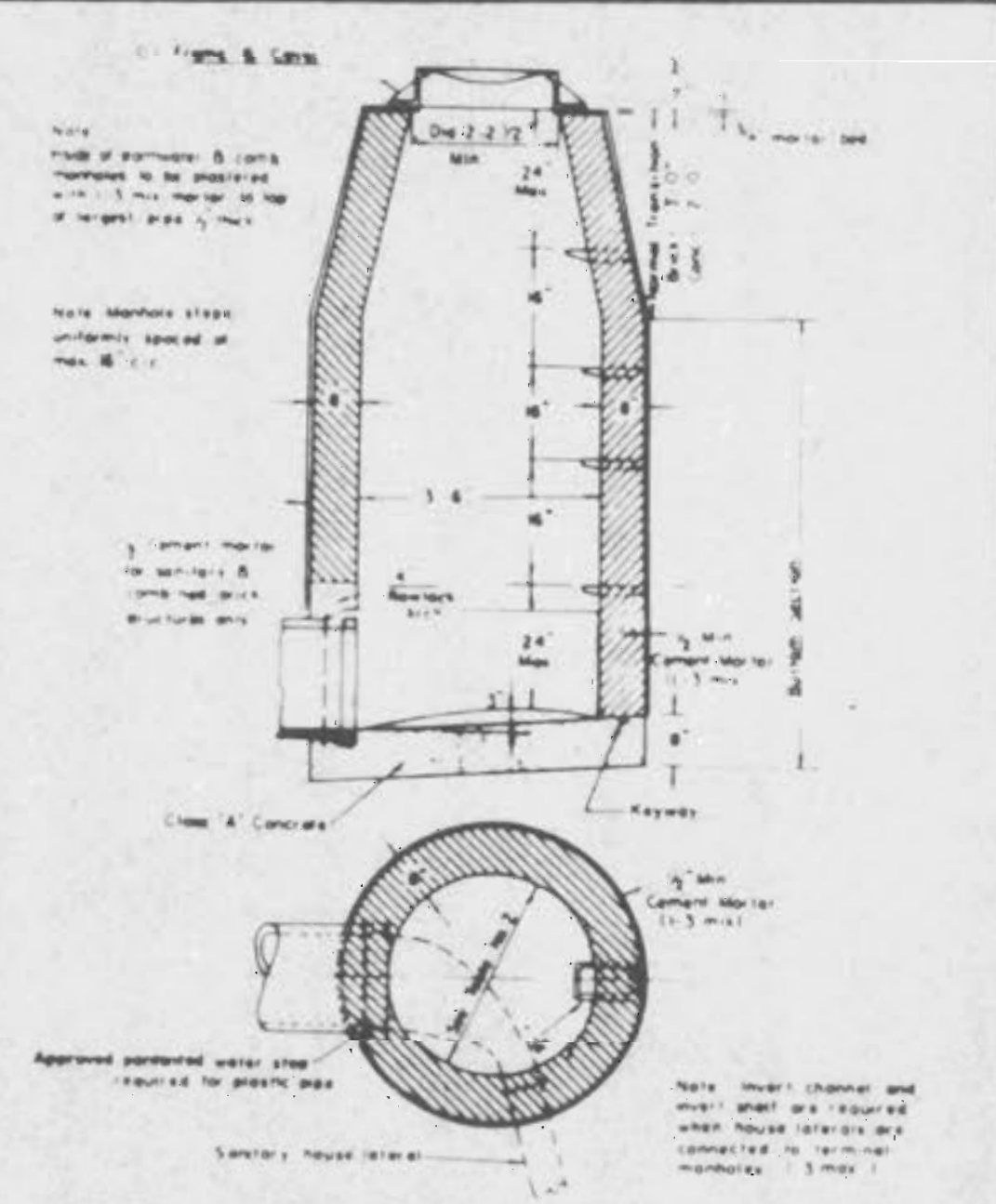
PRE-CAST CONCRETE MANHOLE FOR SEWERS 8" THROUGH 12" IN DIAMETER DETAIL 17
