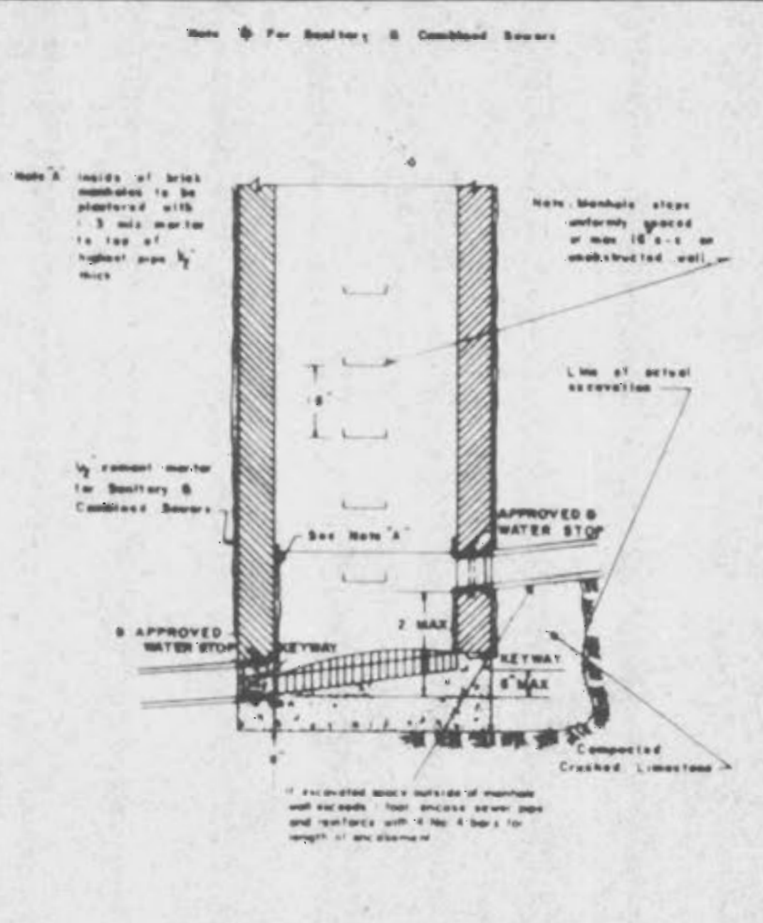
TERMINAL MANHOLE DETAIL 16
