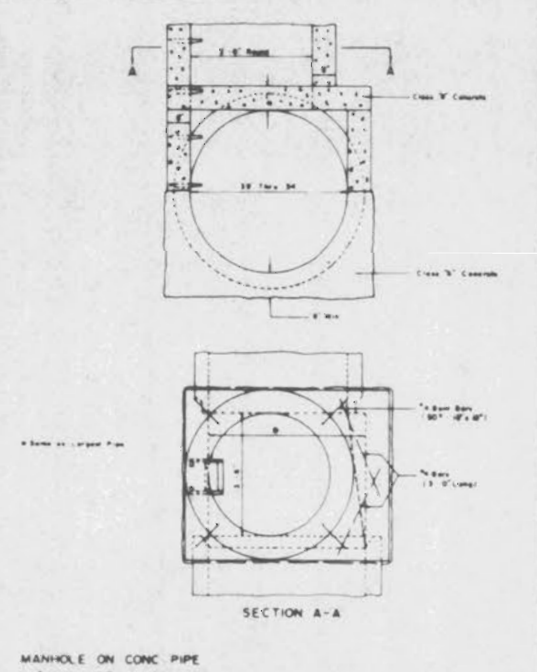
TYPICAL MANHOLE BASE REINFORCED CONCRETE PIPE SEWERS 60" AND LARGER IN DIAMETER DETAIL 11
