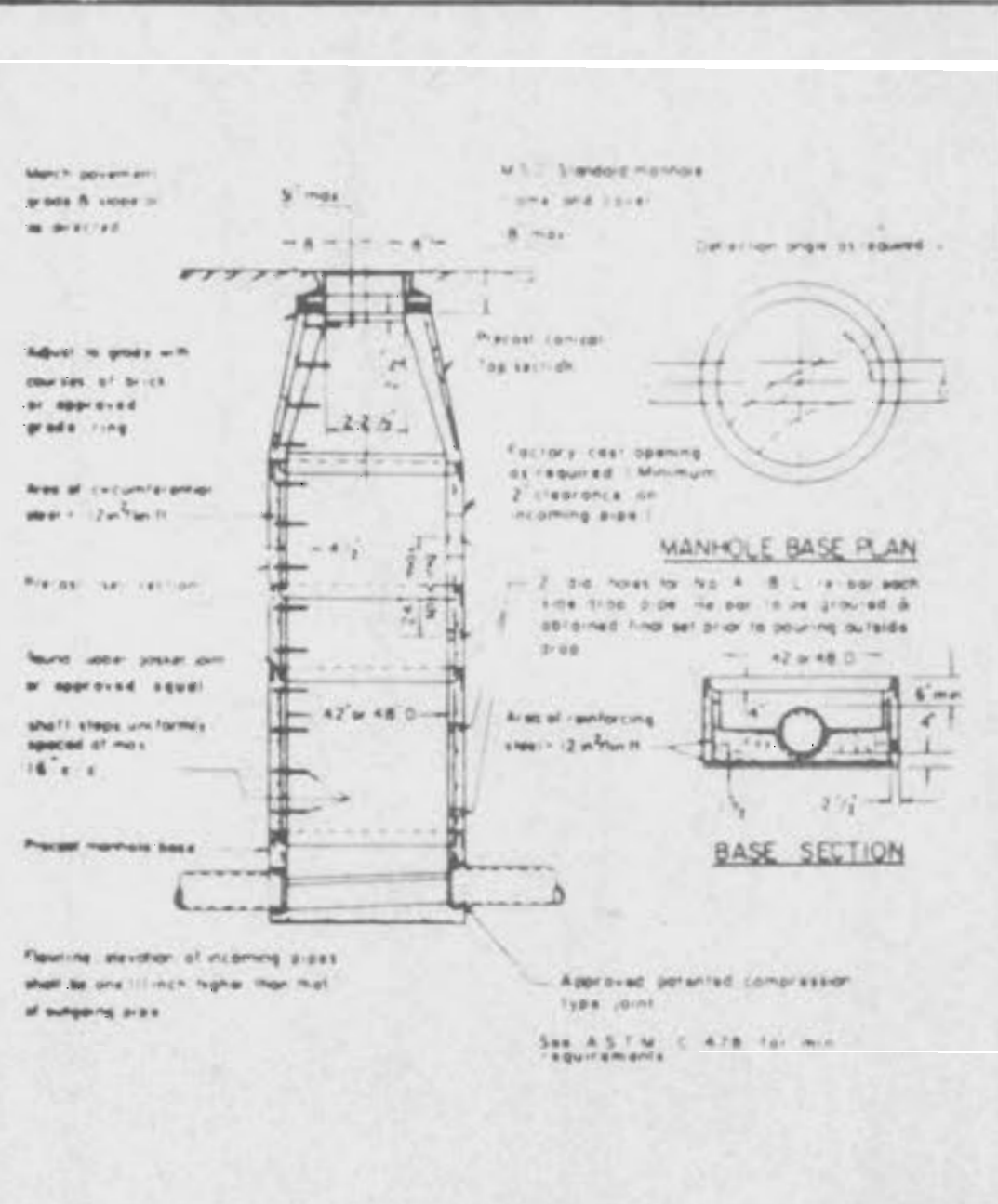
PRE-CAST CONCRETE MANHOLE FOR SEWERS 8" THROUGH 12" IN DIAMETER DETAIL 18
