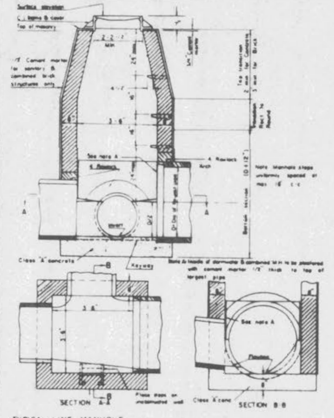
MANHOLE ON CONCRETE PIPE SEWERS 39" THRU 54" DIAMETER DETAIL 8
