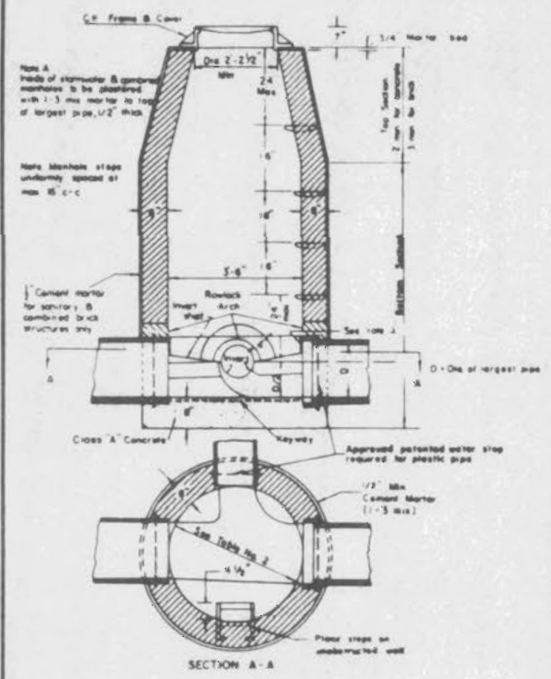
TYPICAL LINE MANHOLE ON PIPE SEWER 27" THRU 36" IN DIAMETER DETAIL 7
