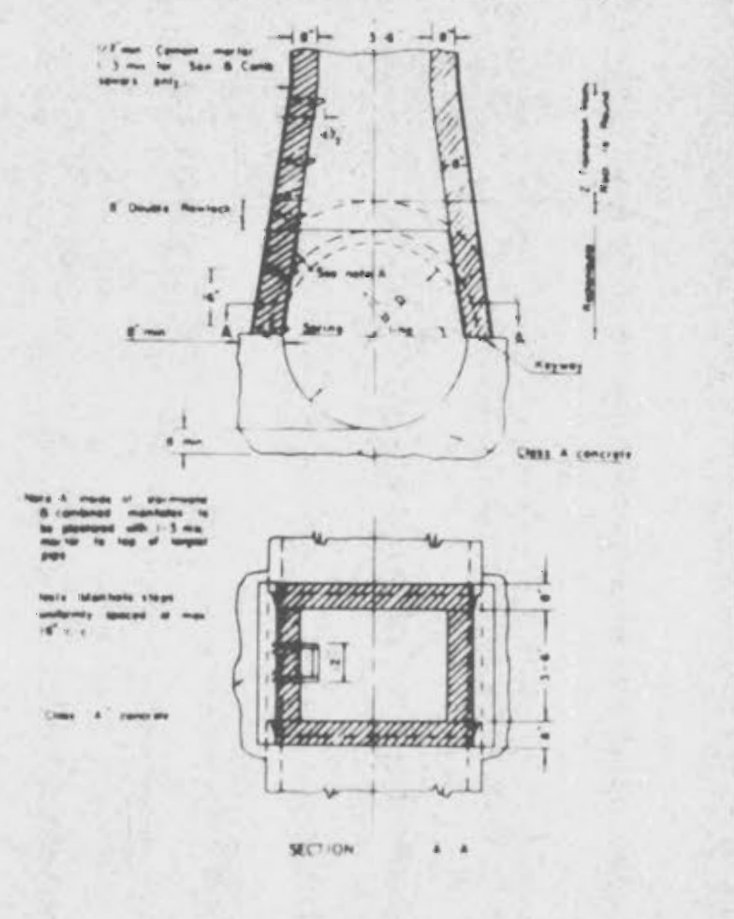
MANHOLE ON CONCRETE PIPE SEWERS 39" THRU 54" DIAMETER (ALTERNATE) DETAIL 10
