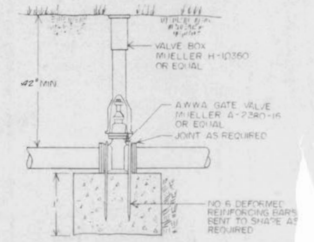
GATE VALVE W / THRUST BLOCK NO SCALE
