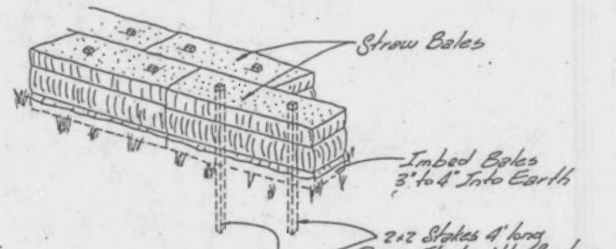
SILTATION CONTROL DETAIL Not to Scale ALTERNATE - SILTATION FABRIC
