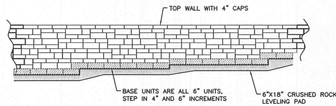
MOSAIC STEP DETAIL NOT TO SCALE
