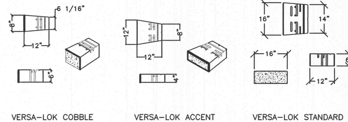
MOSAIC BLOCK DETAIL NOT TO SCALE
