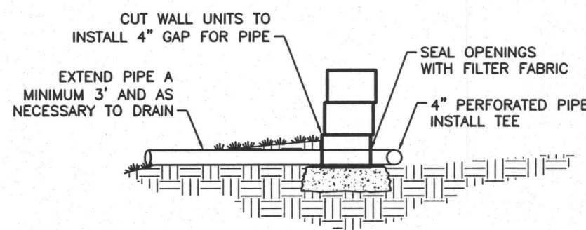
PERFORATED PIPE OUTLET NOT TO SCALE
