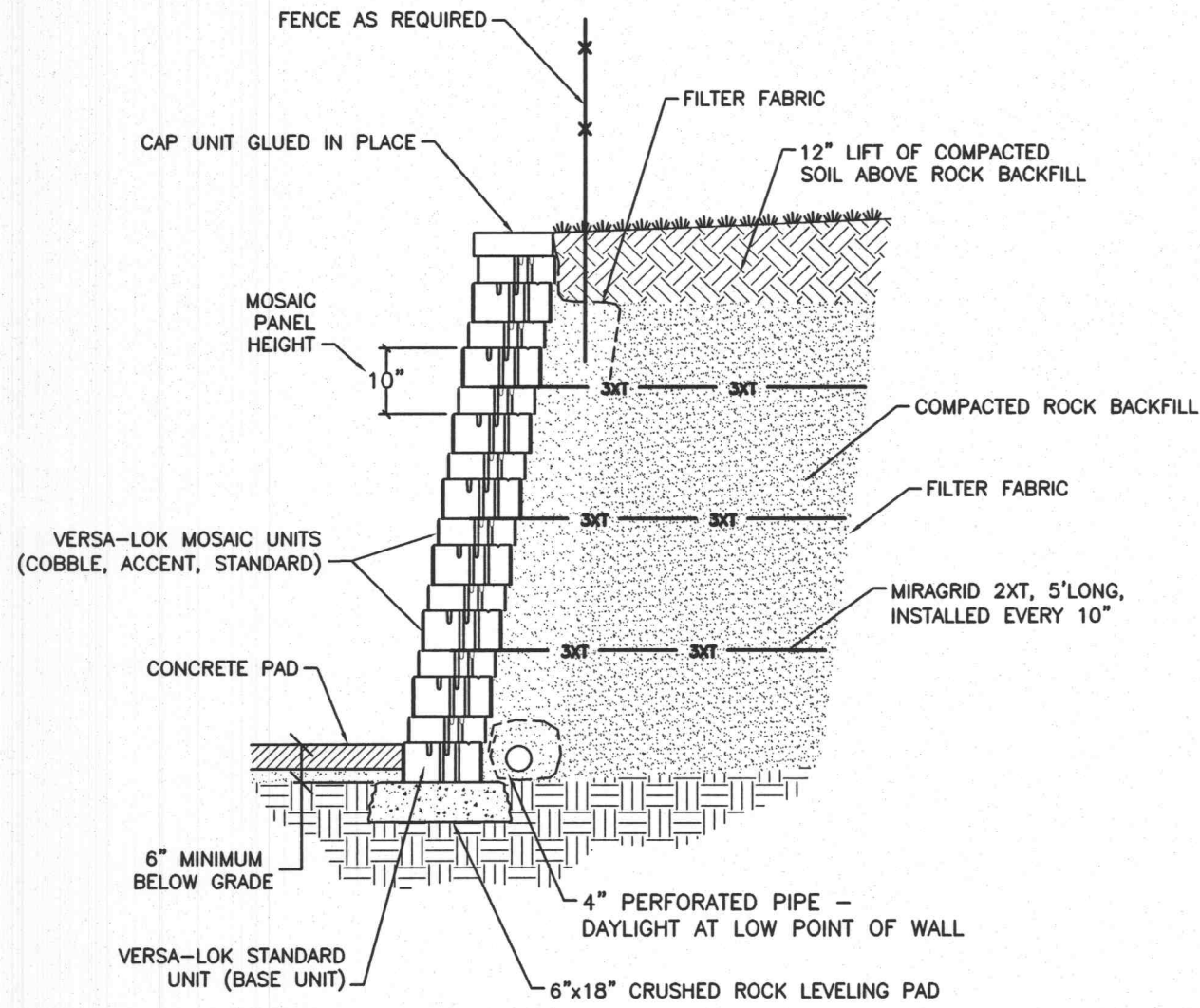
TYPICAL SECTION NOT TO SCALE
