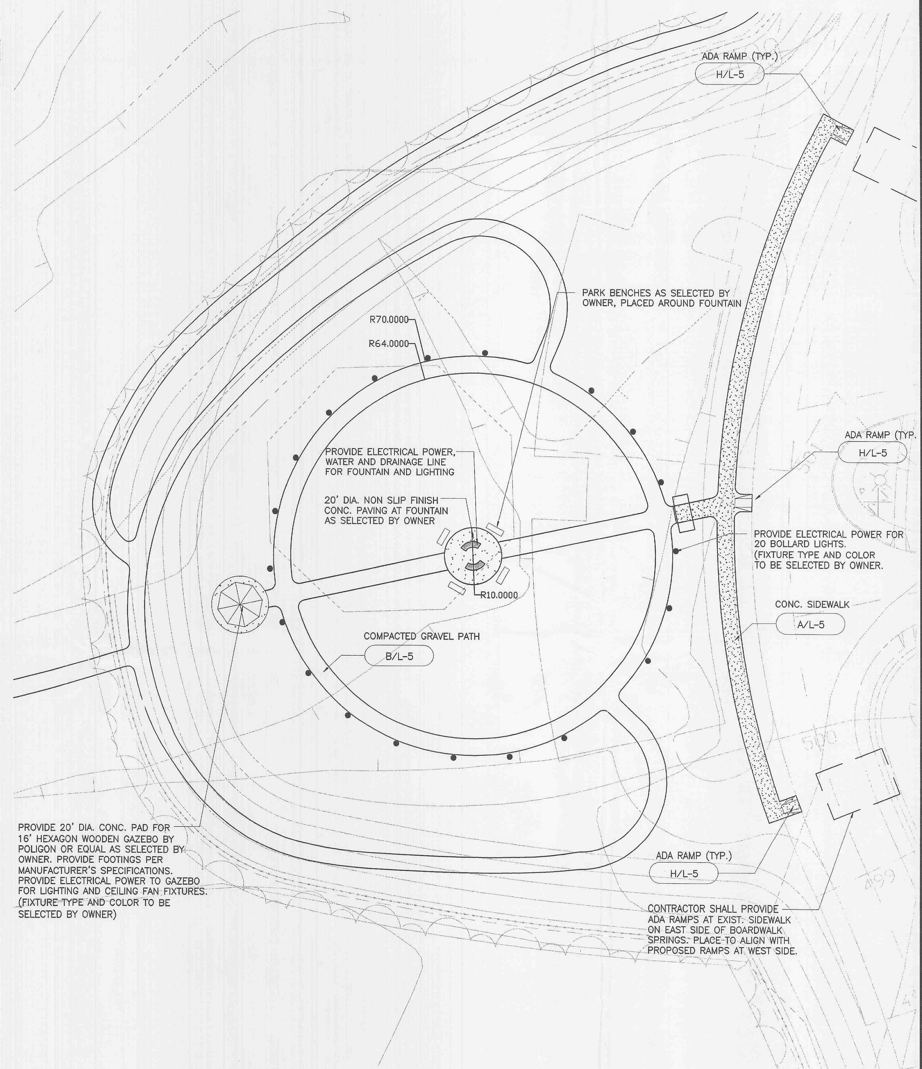
B MISTY MOUNTAIN DRIVE TERMINUS LAYOUT PLAN
