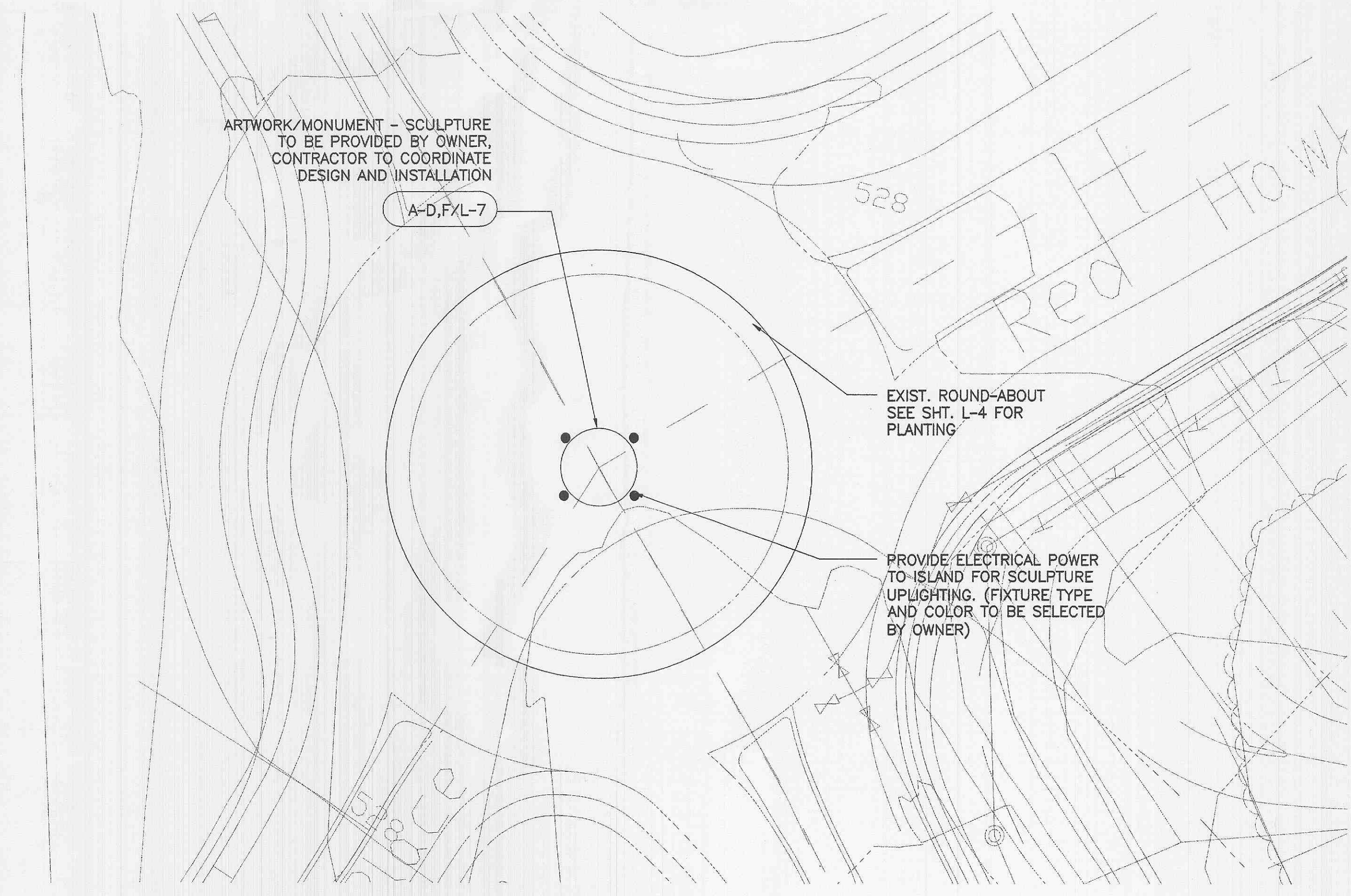
C RED HAWK ROUND-ABOUT LAYOUT PLAN
