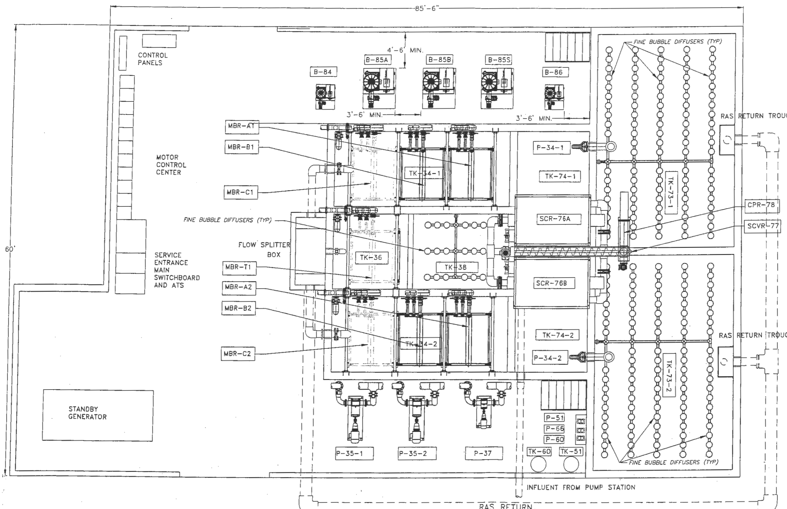
PLAN VIEW (WITHOUT TANK COVERS/CONCRETE TOPS) N.T.S.
