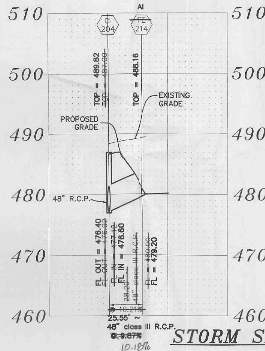
STORM SEWER PROFILES HORIZONTAL SCALE: 1" = 50' VERTICAL SCALE: 1" = 10'
