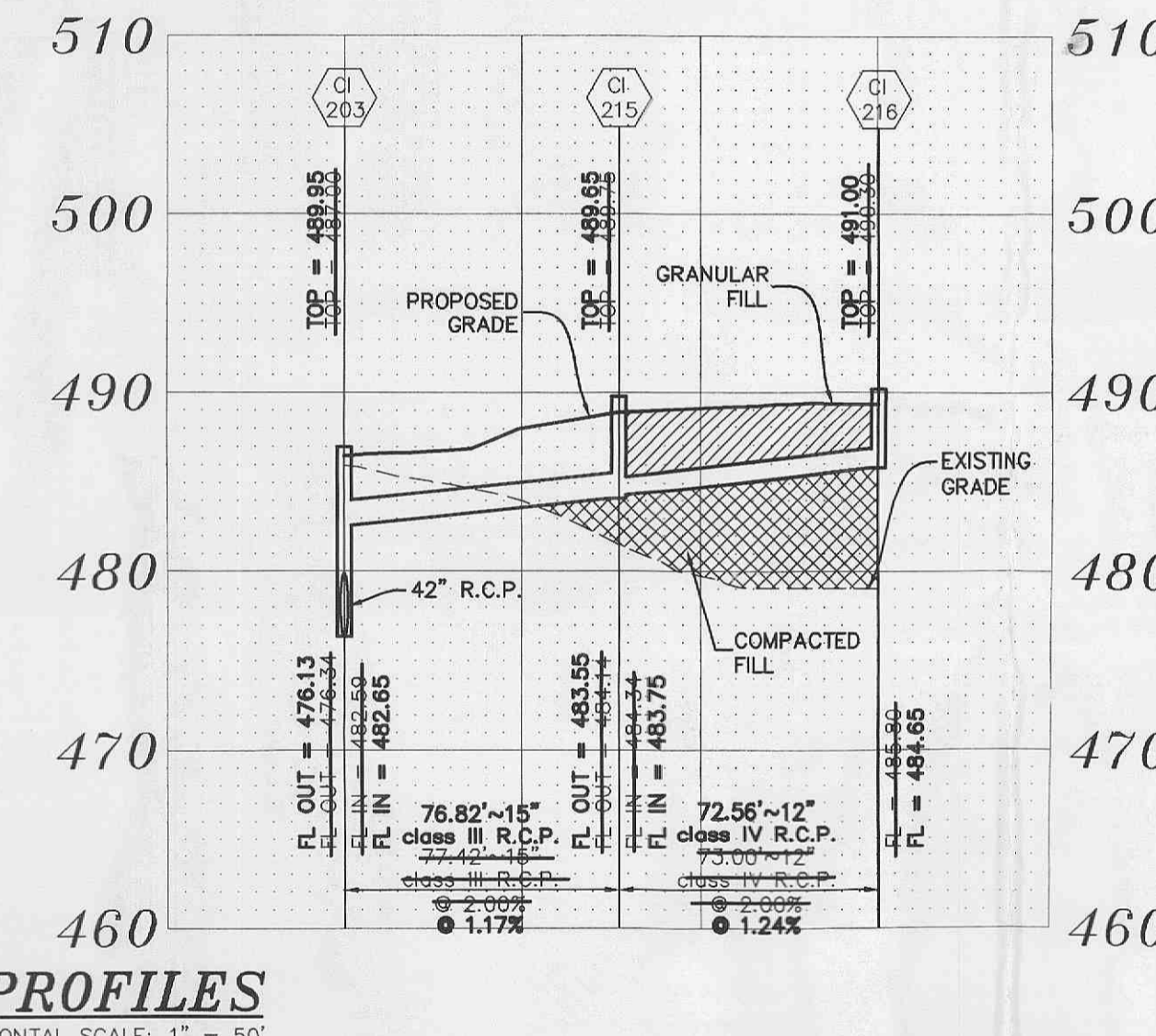
STORM SEWER PROFILES HORIZONTAL SCALE: 1" = 50' VERTICAL SCALE: 1" = 10'
