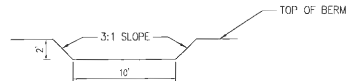
6 EMERGENCY SPILLWAY DETAIL SCALE: REF. DWG.
