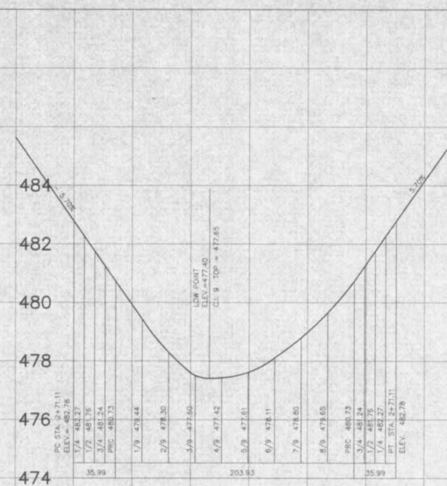
LEXINGTON PASS CUL-DE-SAC WARPING TOP OF CURB ELEVATION
