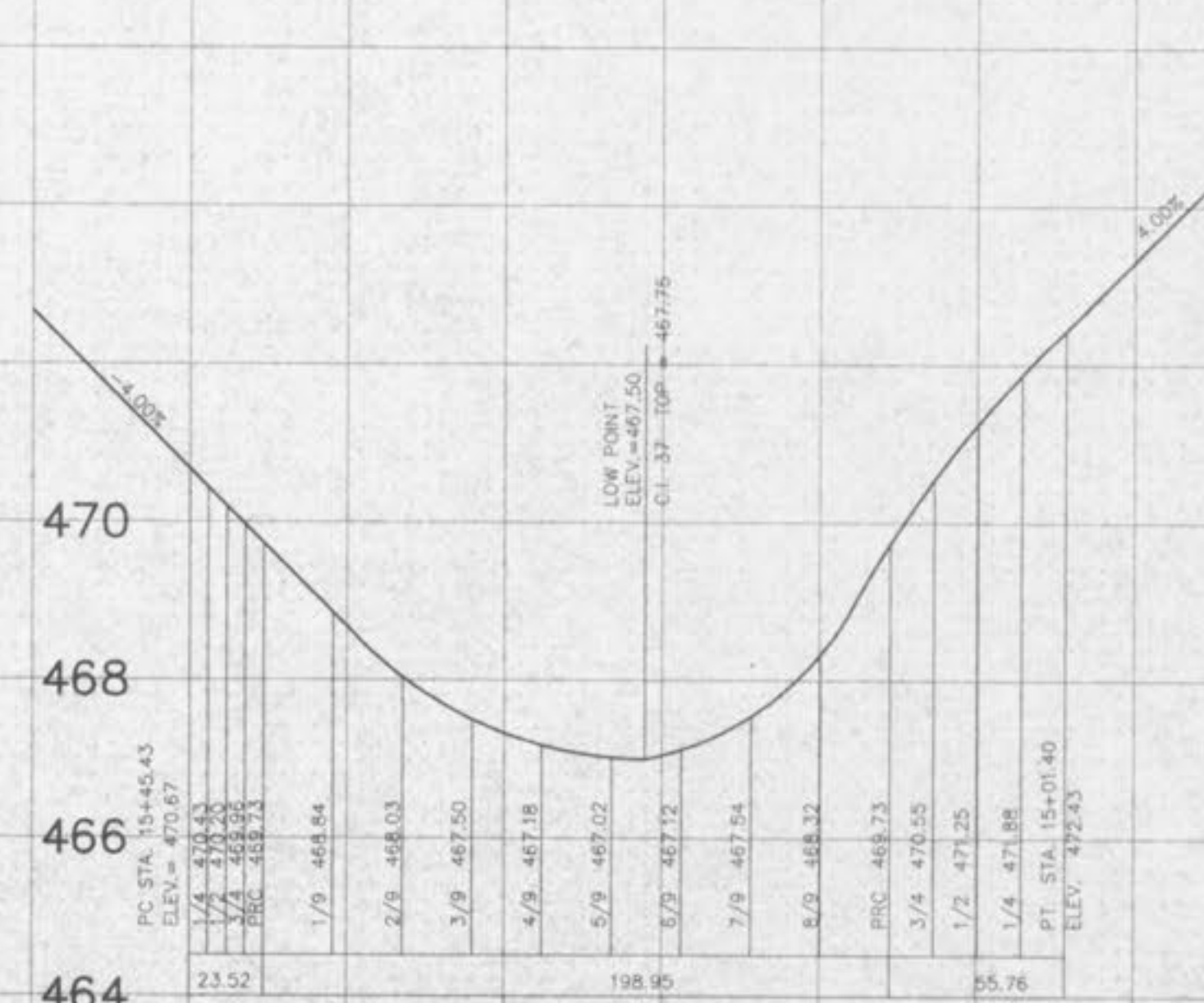
ZUMWALT CROSSING CUL-DE-SAC WARPING TOP OF CURB ELEVATION
