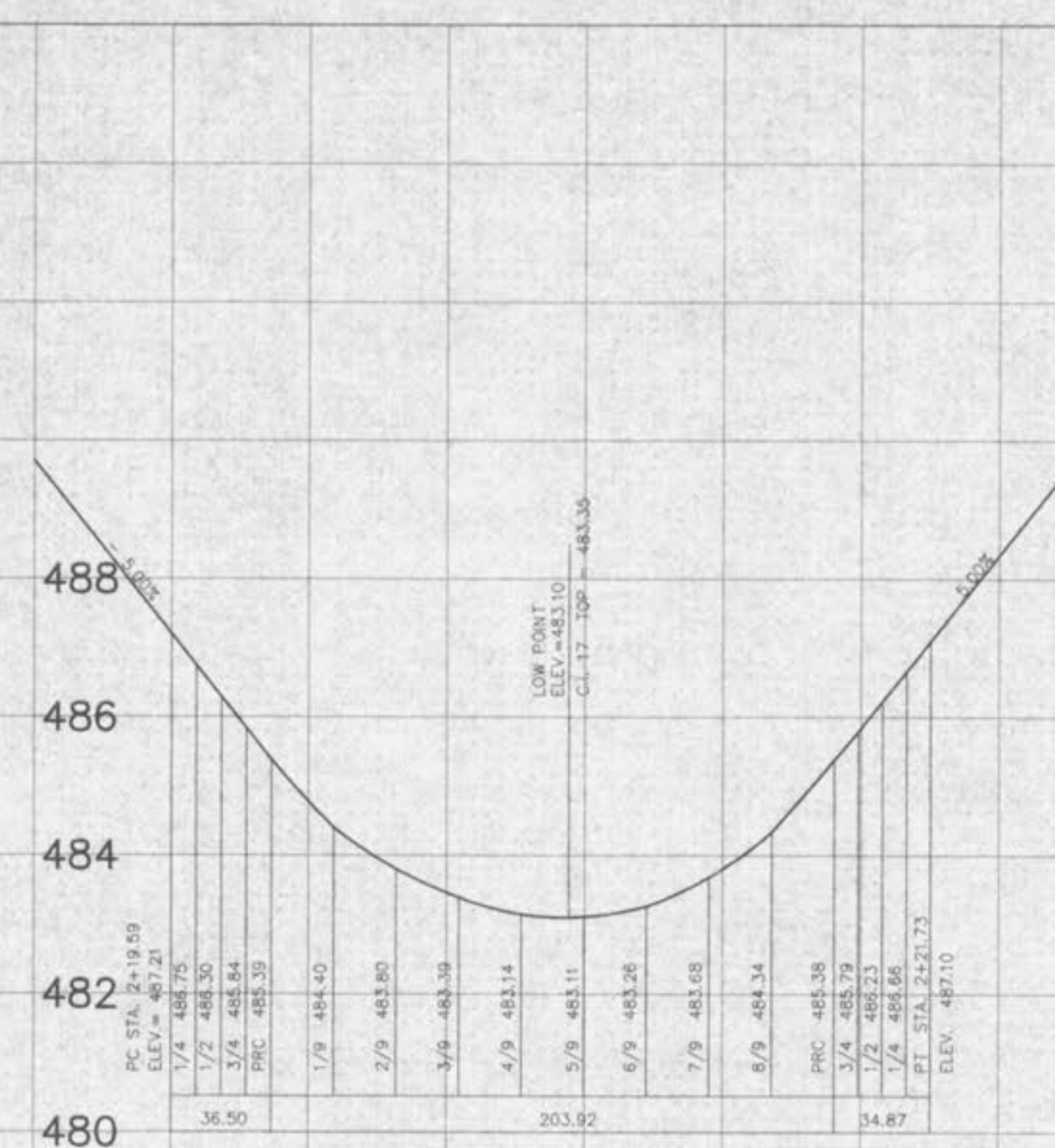
ZUMWALT PASS CUL-DE-SAC WARPING TOP OF CURB ELEVATION
