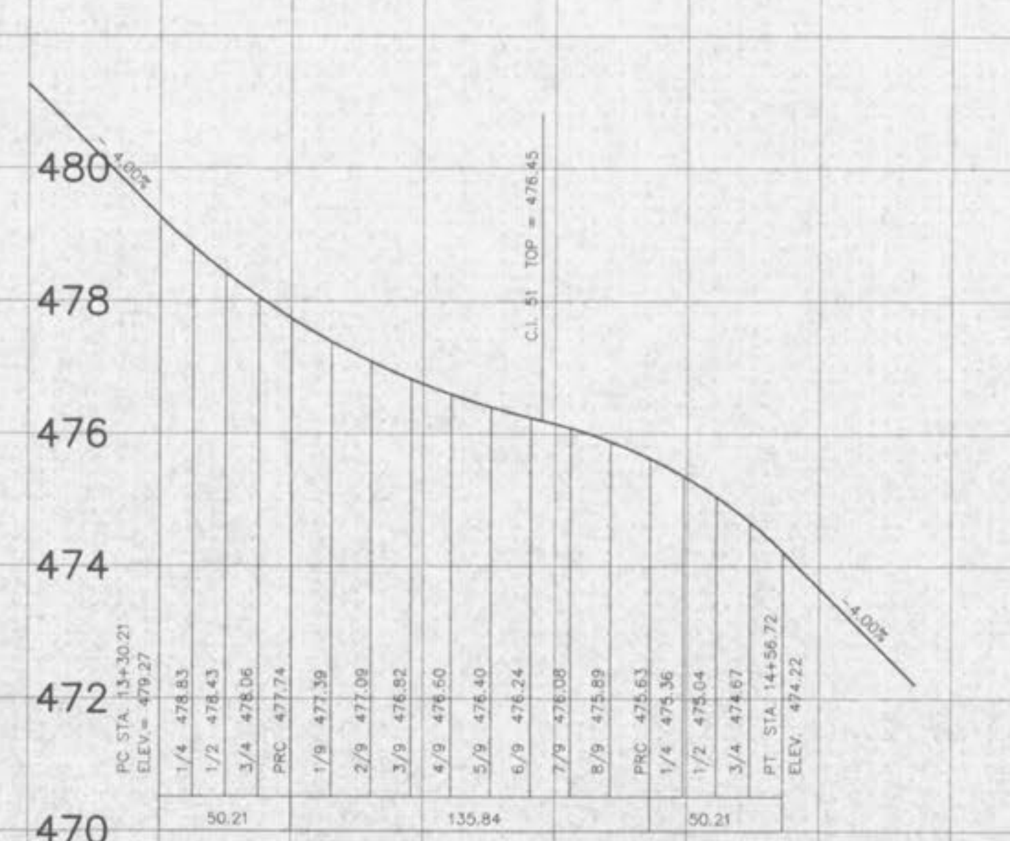
ZUMWALT CROSSING EYEBROW CUL-DE-SAC WARPING TOP OF CURB ELEVATION
