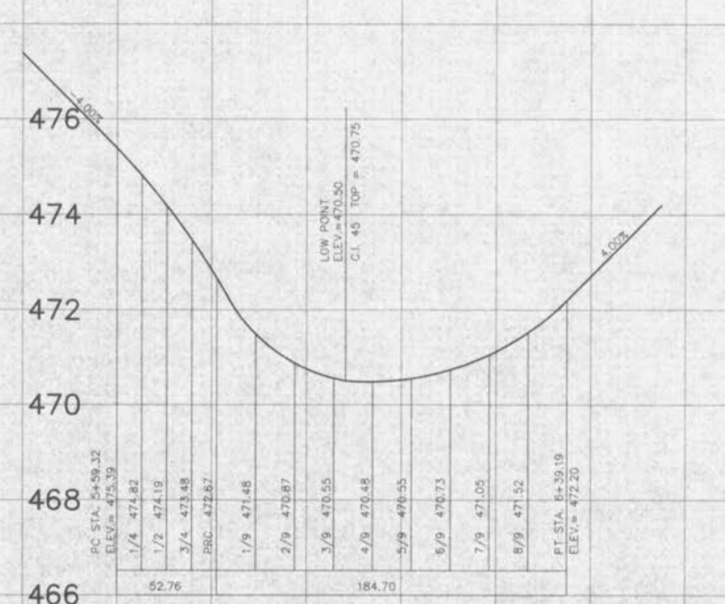
RAINTREE PASS CUL-DE-SAC WARPING TOP OF CURB ELEVATION
