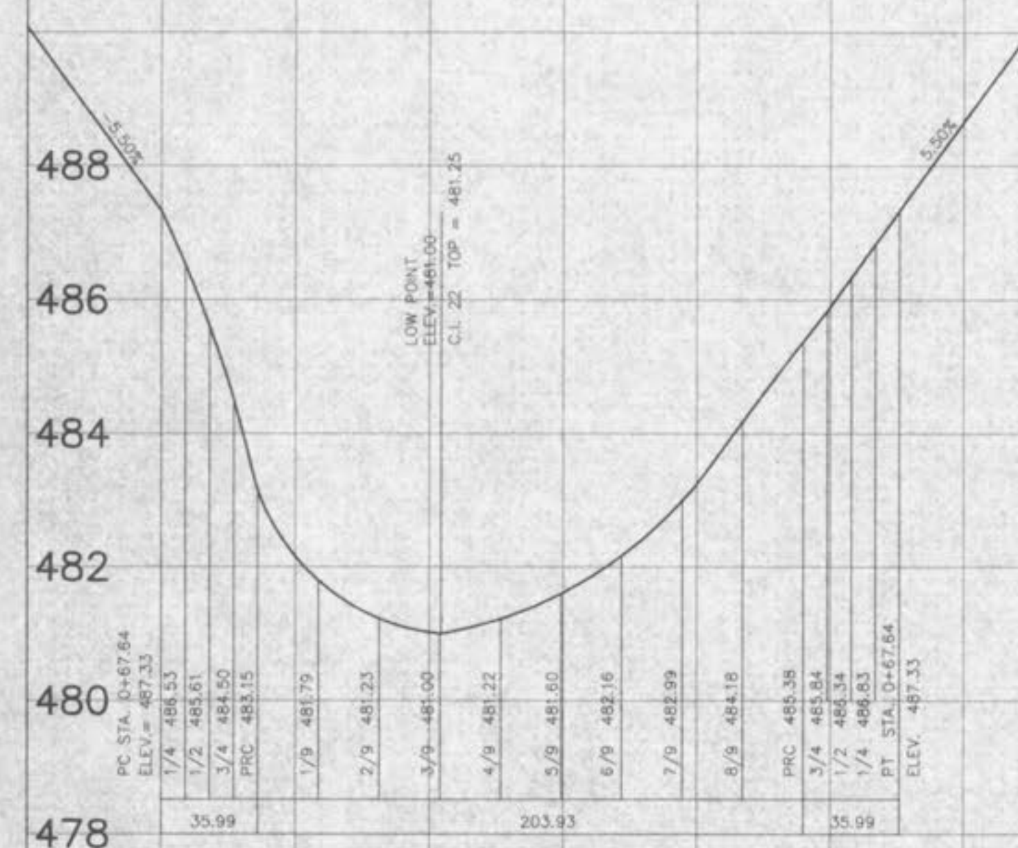
RADFORD PASS CUL-DE-SAC WARPING TOP OF CURB ELEVATION
