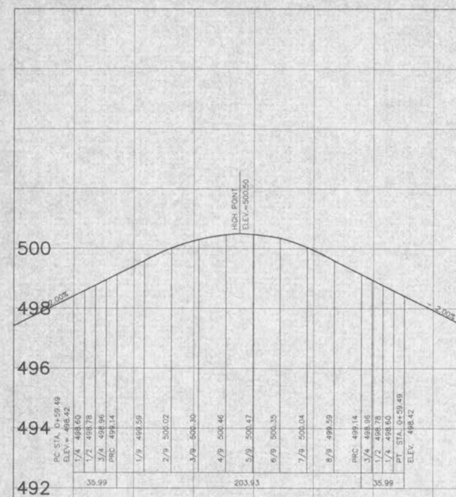
VANTAGE PASS CUL-DE-SAC WARPING TOP OF CURB ELEVATION
