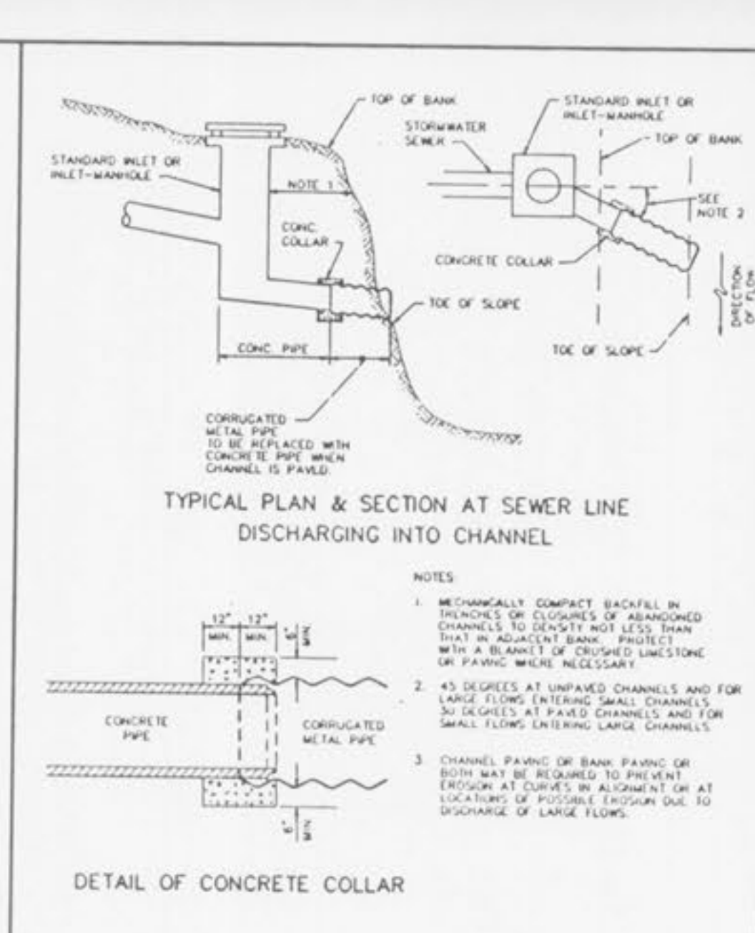
STORMWATER CHANNELS METROPOLITAN ST. LOUIS SEWER DISTRICT Standard Details of Sewer Construction Dr. R.G.W. J.C.K. 1992 SHEET 58
