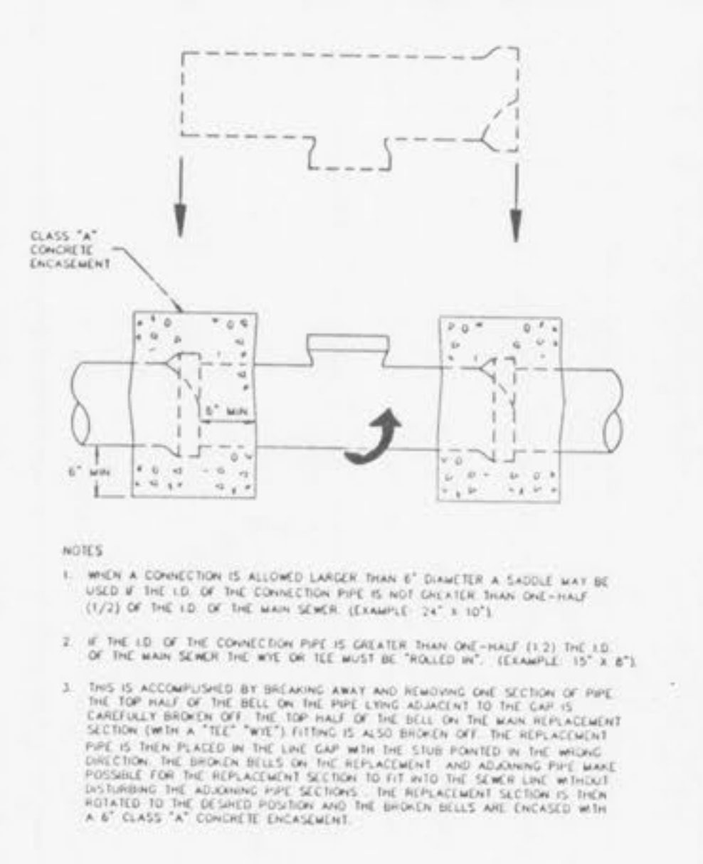
"ROLL-IN" (FOR EXISTING CLAY OR CONCRETE PIPE) METROPOLITAN ST. LOUIS SEWER DISTRICT Standard Details of Sewer Construction Dr. D.A.B. J.C.K. 1992 SHEET 63
