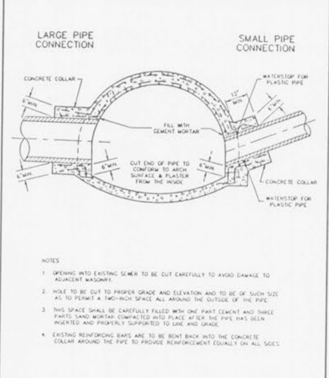
CONNECTIONS TO LARGE SEWERS METROPOLITAN ST. LOUIS SEWER DISTRICT Standard Details of Sewer Construction Dr. W.S.H. J.C.K. 1992 SHEET 64
