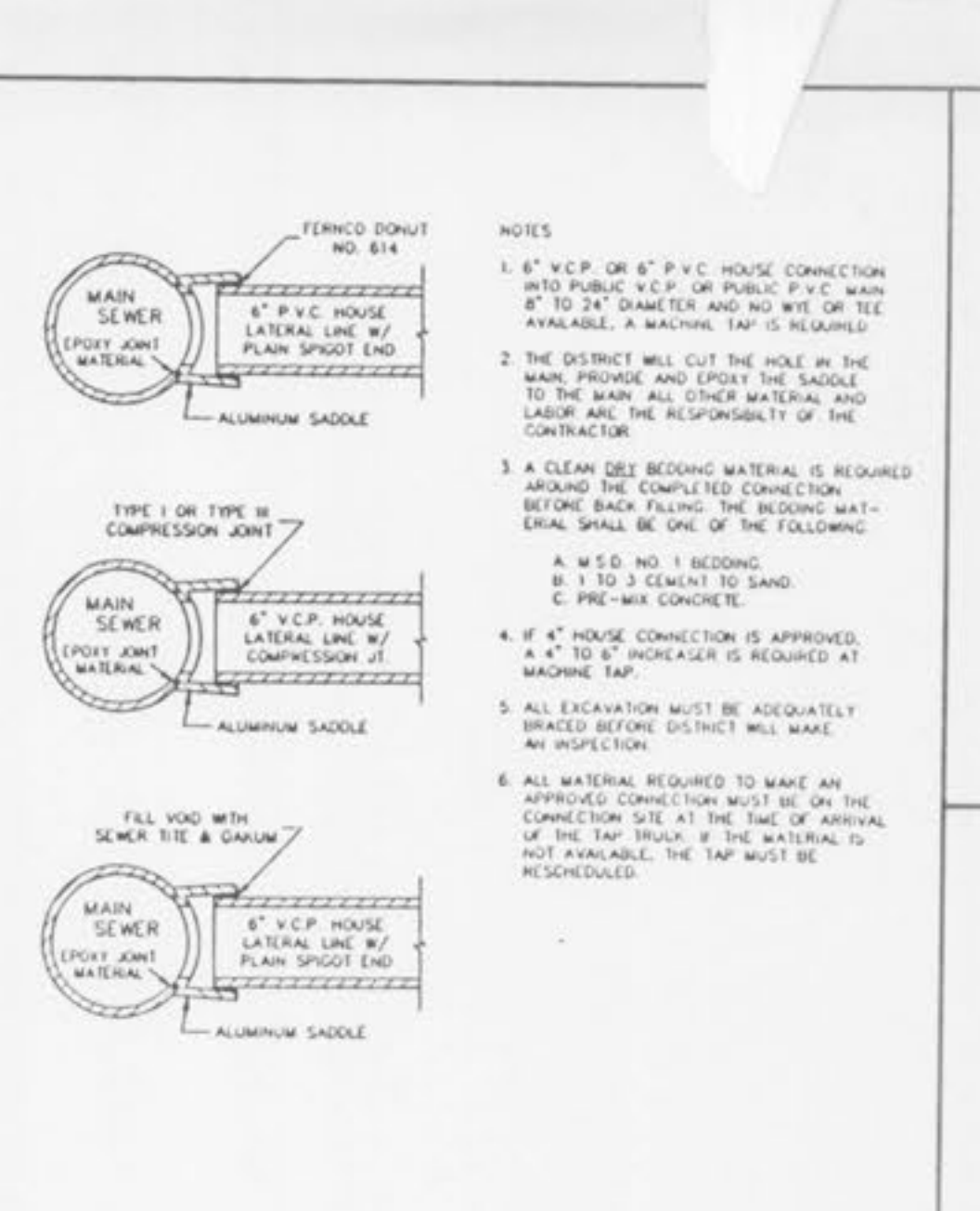
MACHINE TAP METROPOLITAN ST. LOUIS SEWER DISTRICT Standard Details of Sewer Construction Dr. W.S.H. J.C.K. 1992 SHEET 60
