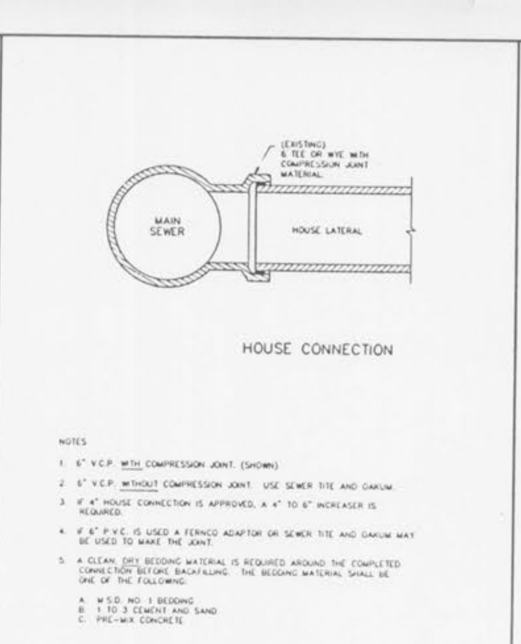
HOUSE CONNECTION TO EXISTING TEE OR WYE METROPOLITAN ST. LOUIS SEWER DISTRICT Standard Details of Sewer Construction Dr. D.A.B. J.C.K. 1992 SHEET 59
