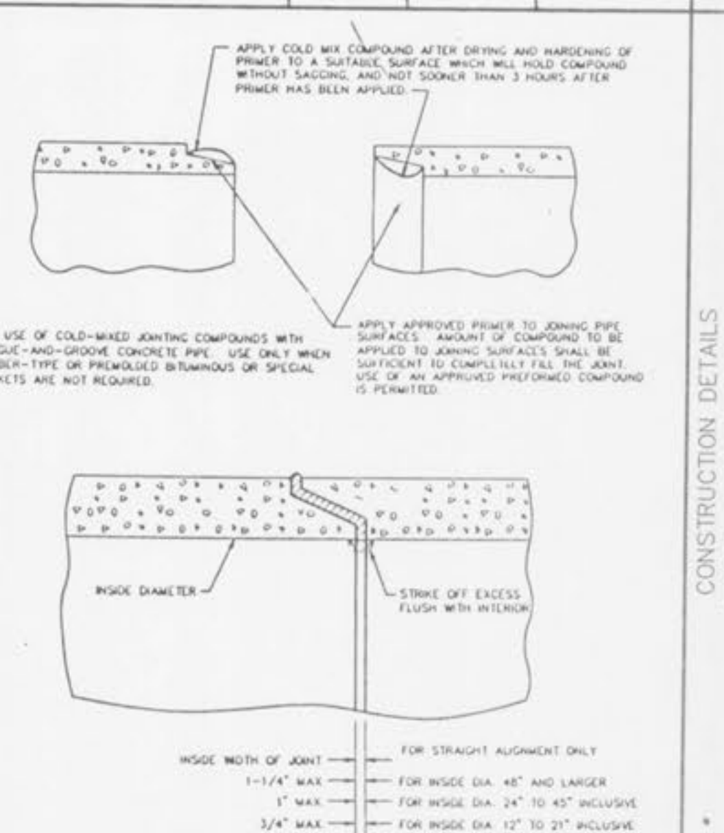
TONGUE AND GROOVE CONCRETE PIPE JOINTS METROPOLITAN ST. LOUIS SEWER DISTRICT Standard Details of Sewer Construction Dr. D.A.B. J.C.K. 1992 SHEET 66
