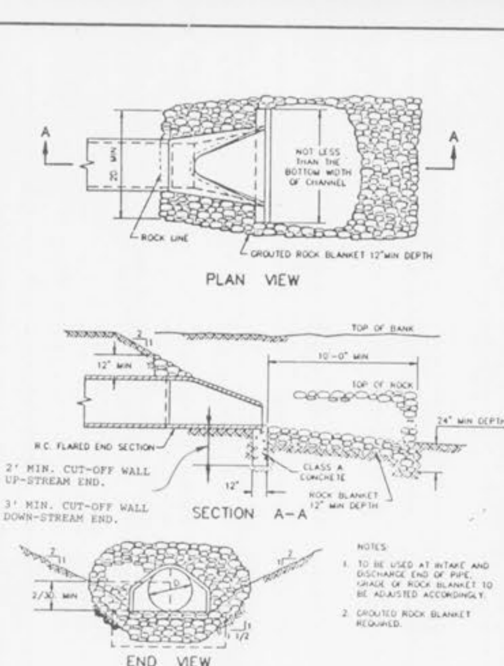
FLARED END SECTION METROPOLITAN ST. LOUIS SEWER DISTRICT Standard Details of Sewer Construction Dr. W.S.H. J.C.K. 1992 SHEET 57
