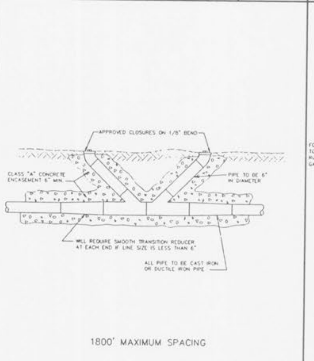
FORCE MAIN CLEANOUT (6" DIA. & SMALLER) METROPOLITAN ST. LOUIS SEWER DISTRICT Standard Details of Sewer Construction Dr. R.G.W. J.C.K. 1992 SHEET 65
