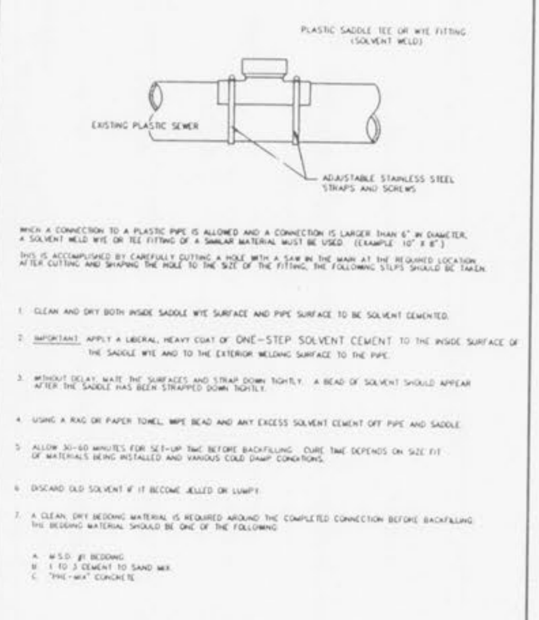
8" (& LARGER) CONNECTION TO PLASTIC MAIN METROPOLITAN ST. LOUIS SEWER DISTRICT Standard Details of Sewer Construction Dr. D.A.B. J.C.K. 1992 SHEET 62
