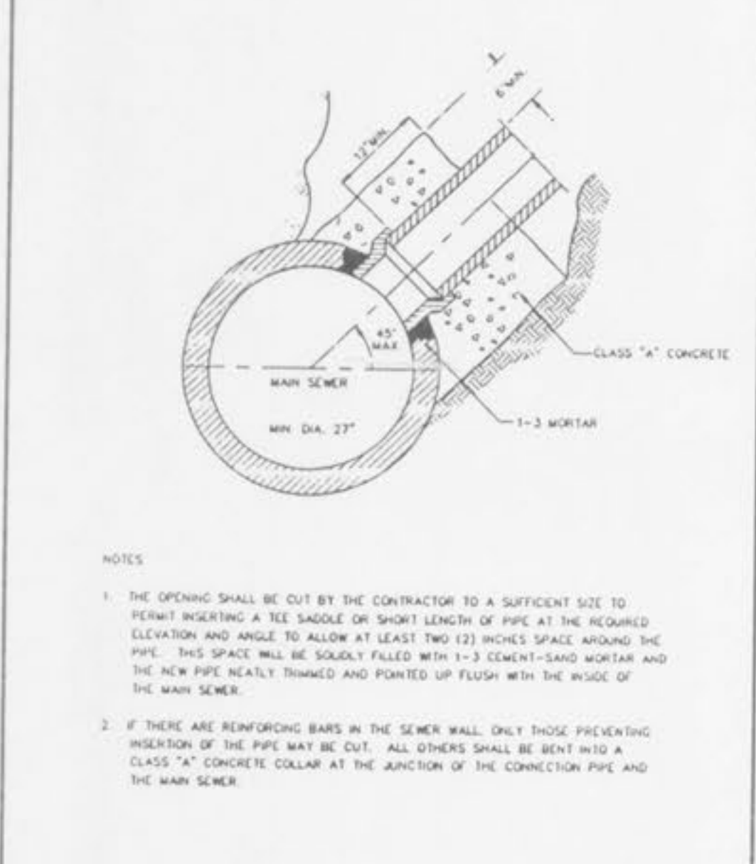
HOUSE CONNECTIONS ALLOWED BY TEE SADDLE METROPOLITAN ST. LOUIS SEWER DISTRICT Standard Details of Sewer Construction Dr. D.A.B. J.C.K. 1992 SHEET 61
