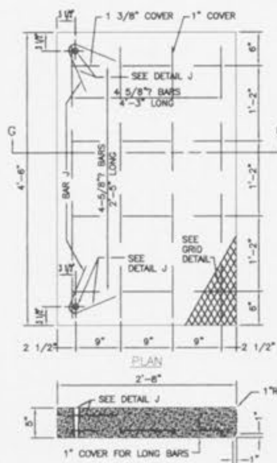
REINFORCED CONCRETE STONE FOR ADDITIONAL UNITS OF MULTIPLE UNIT INLET
