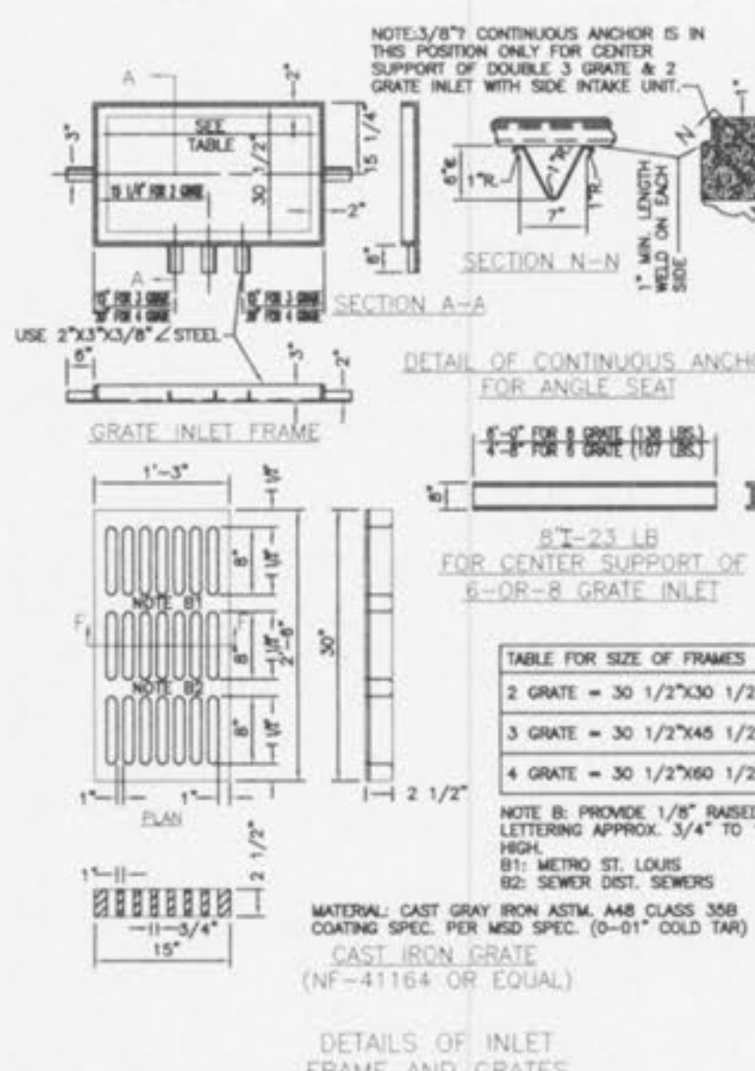
DETAILS OF INLET FRAME AND GRATES
