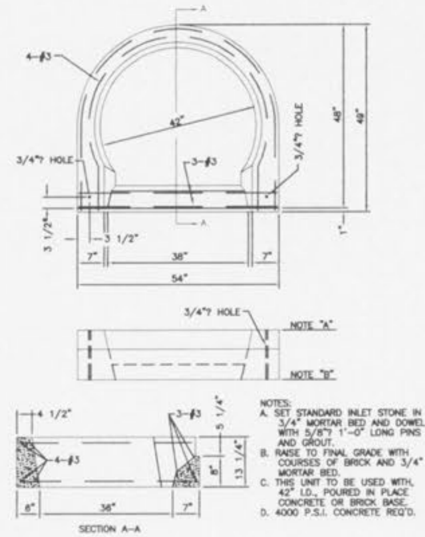
PRECAST CONCRETE UNIT FOR SINGLE CURB INLET
