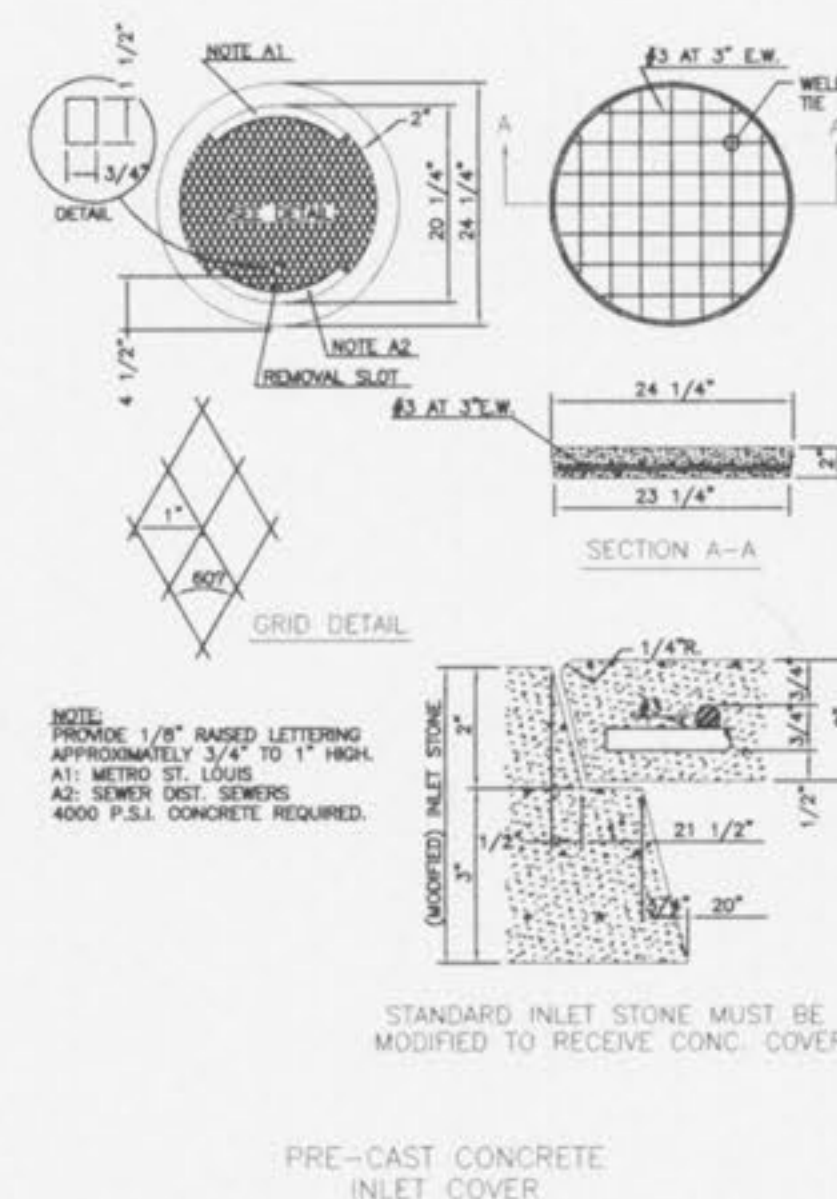
PRE-CAST CONCRETE INLET COVER
