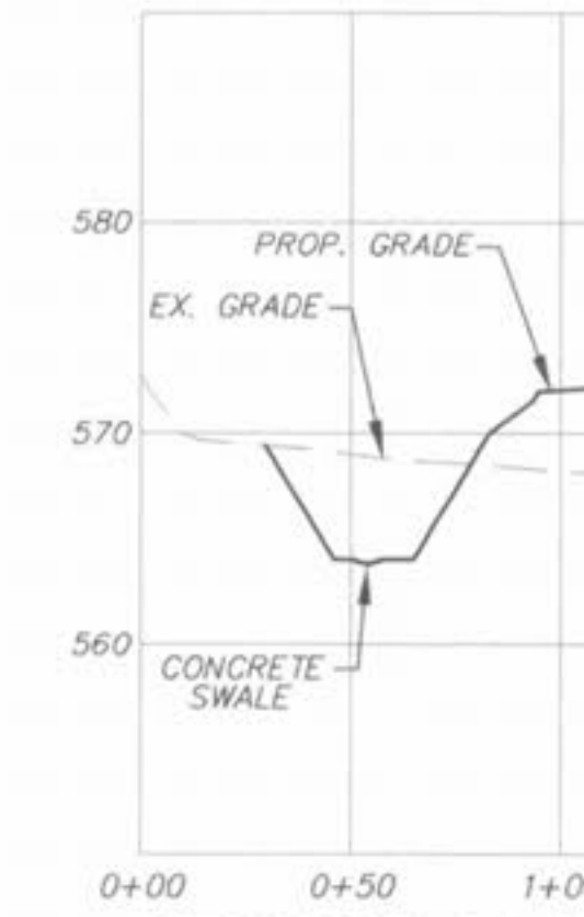
SECTION E-E
