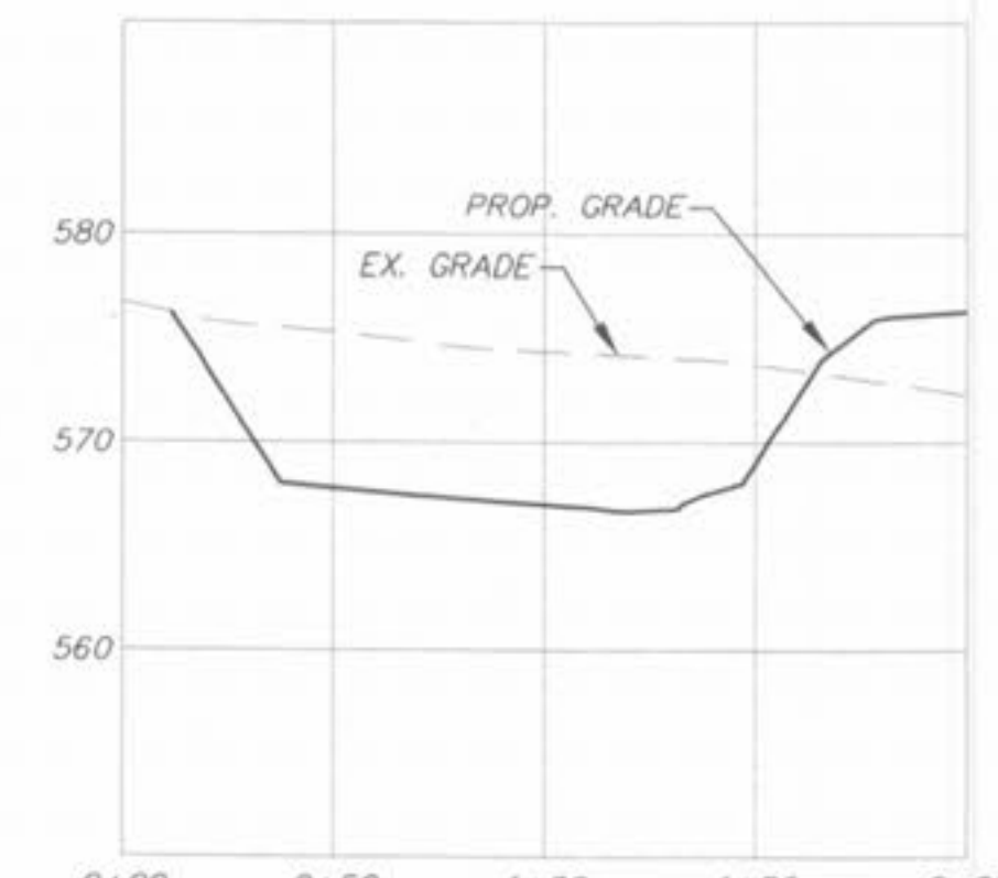
SECTION C-C
